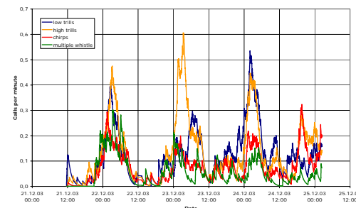
Diurnal variation in the emission rate of selected Weddell seal calls
