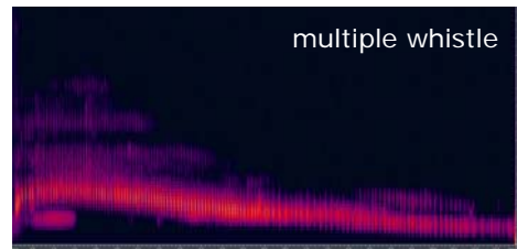
Spectrograms of selected Weddell seal calls
