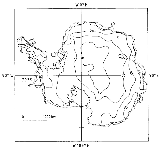
Fig. 2. Distribution of accumulation for present conditions as obtained from a computer interpolation on point measurements. Labelled contour lines are in cm/y
