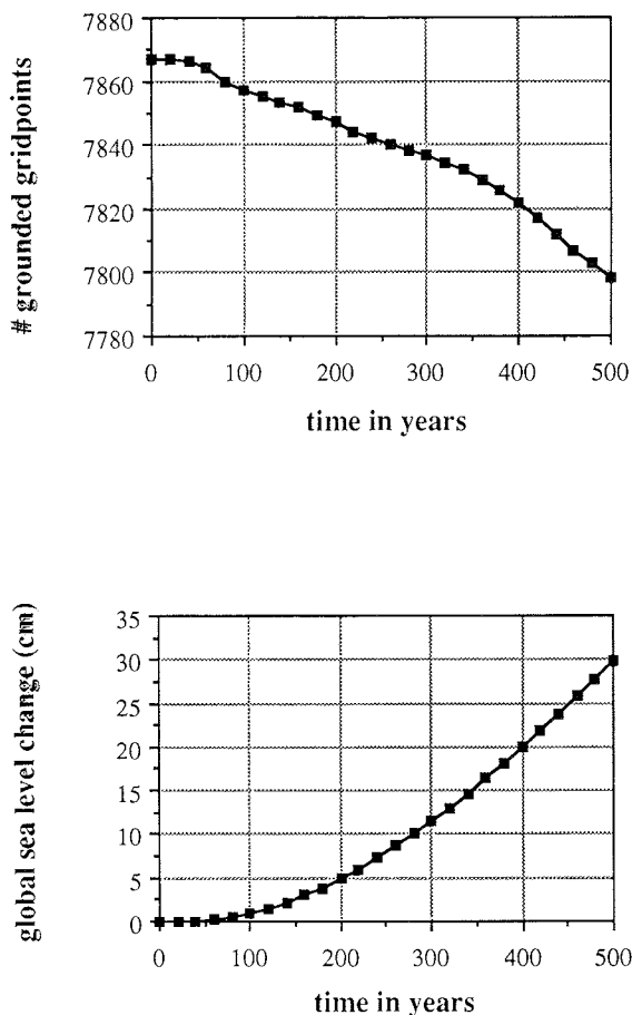
Fig. 11. Response of the Antarctic ice sheet to an instantaneously imposed melting rate beneath ice shelves of 1 m/yr. According to the model, the area of grounded ice would decrease by less than 1% in 500 years
