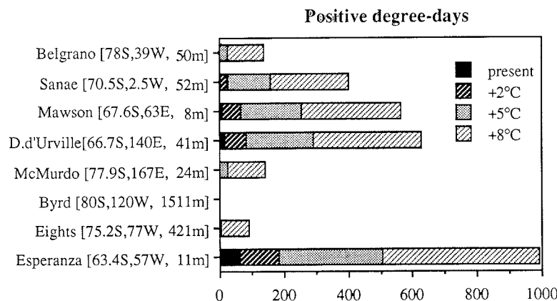
Fig. 4. Calculated amount of positive degree-days (PDD) for various Antarctic stations
