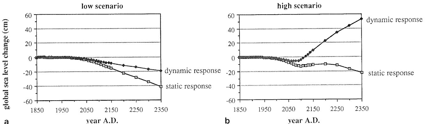
Fig. 9a, b. Response of the Antarctic ice sheet expressed in global sea level changes for the 'low scenario' (a), and for the 'high scenario' (b)
