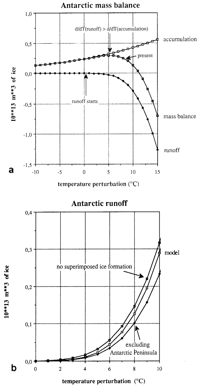
Fig. 5. a Dependence of Antarctic mass balance components on temperature relative to present. For a temperature rise below 5.3 K, the mass balance would be larger than today. b The effect of superimposed ice formation on the predicted runoff. The lowest curve indicates the relative importance of the Antarctic Peninsula
