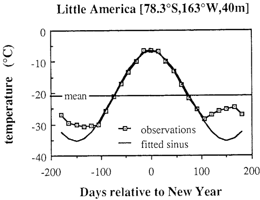
Fig. 3. Fitting of the temperature in the summer half-year with a sine function. This example is for station Little America
