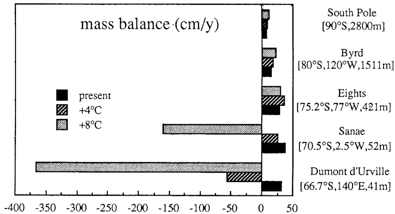
Fig. 6. Mass balance for present conditions and in a warmer climate for some selected Antarctic stations
