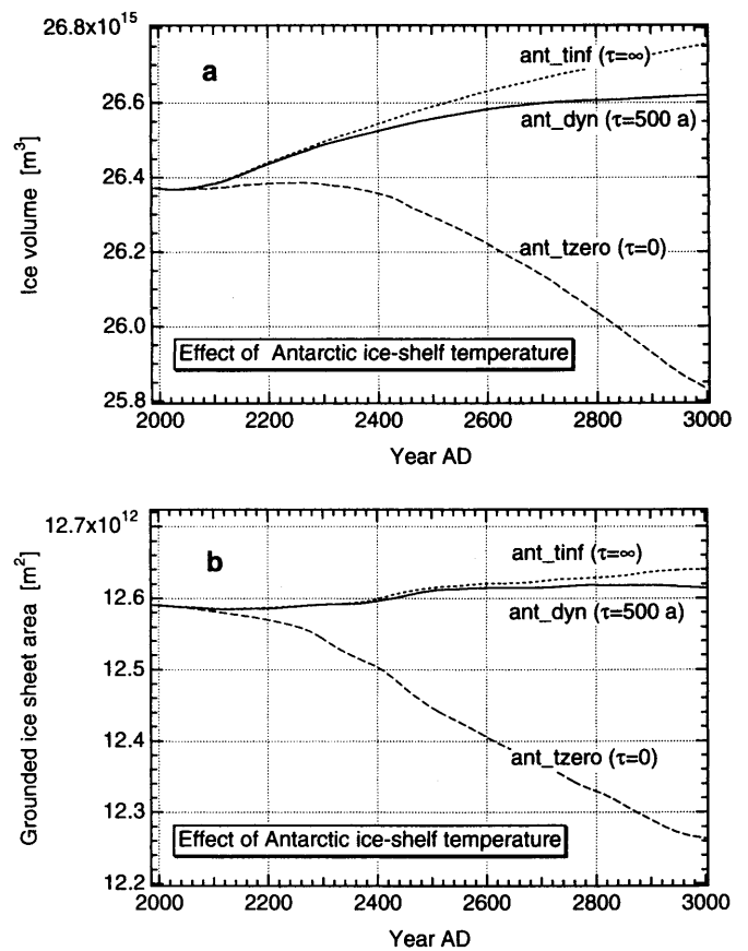
FIG. 13. Evolution of Antarctic ice volume (a) and grounded ice sheet area (b) in a series of experiments testing the effect of ice shelf temperature on grounding-line migration ( ant_tinf , the effective ice shelf deformation temperature is fixed throughout the experiment; ant_tzero , the ice shelf temperature follows the surface perturbation instantaneously; ant_dyn , the characteristic timescale for ice shelf temperature change is 500 yr).
