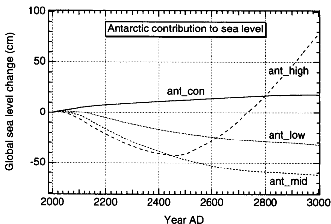
FIG. 7. Longer-term response of the Antarctic ice sheet to three climatic warming scenarios (low, 2 \times \text{CO}_2 ; mid, 4 \times \text{CO}_2 ; high, 8 \times \text{CO}_2 ) up to the year 3000 A.D. expressed in equivalent changes of global sea level. In these experiments, the background evolution (ant_con) is retained as a contribution.
