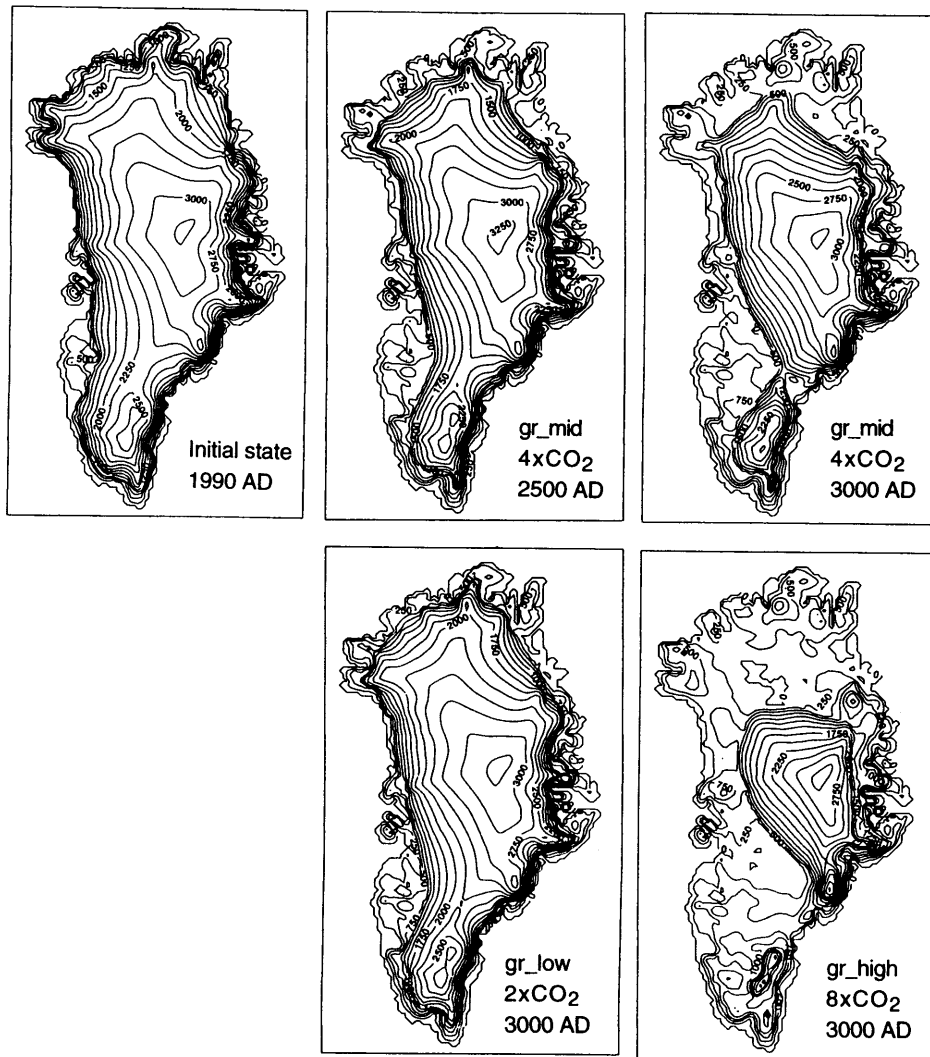
FIG. 11. Snapshots of Greenland surface elevation for the experiments and times indicated in the lower-right corner and further detailed in Table 2 and the main text. The ice sheet margin is easily distinguished by its high surface slope. Contour interval is 250 m.
