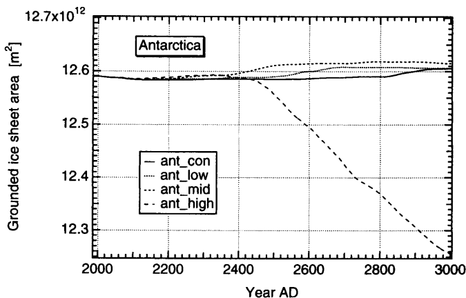
FIG. 8. Change of the grounded ice area of the Antarctic ice sheet for the experiments shown in Fig. 7. Details of the experimental setup are listed in Table 3. Except for the high scenario, grounding-line migration is very limited.
