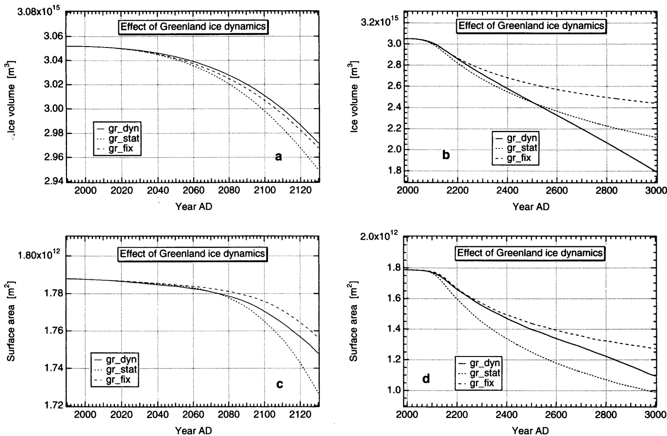
FIG. 10. Evolution of key variables in a series of experiments testing the role of ice dynamics. Shown are (a), (b) ice volume and (c), (d) surface area, (a), (c) both on the short term until 2130 A.D.; and (b), (d) as up to the end of the next millennium. Details of the experiments are given in Table 2 and in the text (gr_dyn, dynamic response; gr_stat, static response; gr_fix, fixed-geometry response).
