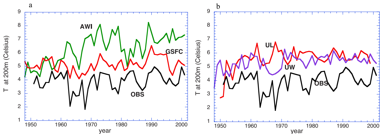
Figure 8. Temperature time series at 200 m from 73.5°N–76.5N, 15°E (i.e., the incoming Atlantic water): (a) the AWI and GSFC model data versus observed temperature (OBS, black; data gap in 1974 filled by interpolation). (b) UL, UW model data versus observations.
