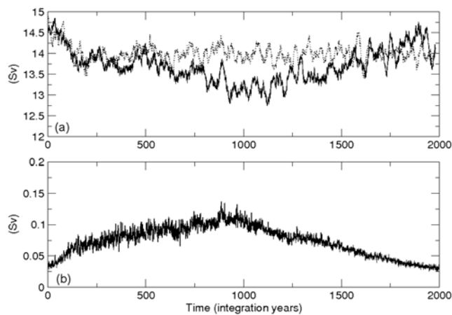
Figure 2. (a) Time series of the annual mean NADW export at 30^{\circ}\text{S} in the Atlantic basin for SRESA2 (solid line) and SRESA2F (dotted line). (b) Time series of the annual mean freshwater flux from Greenland as simulated in SRESA2. Integration year 0 corresponds to year 2000 AD.
