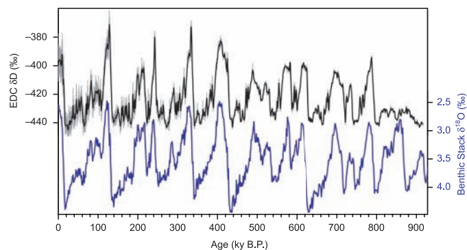
Fig. 1. Comparison of the \delta D Dome C record on the EDC3 time scale (with all data points in light gray and a smoothed curve in black) with the benthic oxygen-18 record (blue) on its own time scale (8). The 3259.7-m \delta D record, which includes published results down to 788 m (38), benefits from an improved accuracy (1 \sigma of \pm 0.5\% ) and a much more detailed resolution of 55 cm all along the core, whereas the previously published record was based on 3.85-m samples (1). The agreement between the two time series back to ~800 ky B.P. justifies the use of oceanic sediment nomenclature (MIS) for describing the ice core record.
