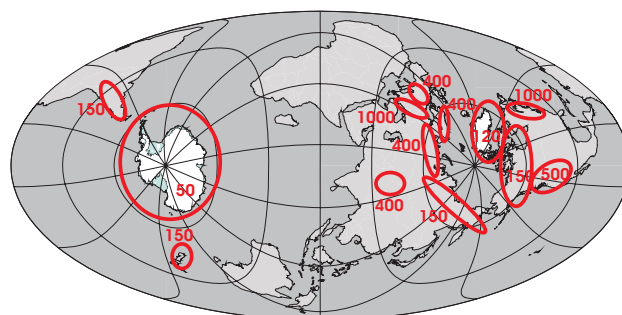
Fig. 8. Estimates of snow nitrate concentrations ( \mu\text{g kg}^{-1} ) for different snow-covered regions. See original references for details. Antarctica and sea ice zone (Mulvaney and Wolff, 1994) (much higher values may be found in the very surface layer in central Antarctic (Röthlisberger et al., 2000) and in coastal regions, where sea salt and mineral aerosols efficiently scavenge nitric acid (Beine et al., 2006)); Greenland and adjacent Arctic islands (Röthlisberger et al., 2002; Koerner et al., 1999); North America: maps at National Atmospheric Deposition Program (NADP) ( http://nadp.sws.uiuc.edu/isopleths/annualmaps.asp ); Alps (summer concentrations) (Preunkert et al., 2003); rest of Europe: EMEP ( http://www.nilu.no/projects/ccc/emepdata.html ); Himalayas (Hou et al., 1999); other regions by analogy. The uncertainty on these values due to extrapolation from specific sites is at the very least a factor 2, and this range has to be explored in sensitivity studies.
