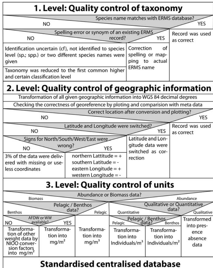
Fig. 1 Nassi-Shneiderman diagram (NSD) for the quality assurance algorithm applied to every record within the LargeNet database. All these tests were necessary to achieve the general comparability between the individual datasets
