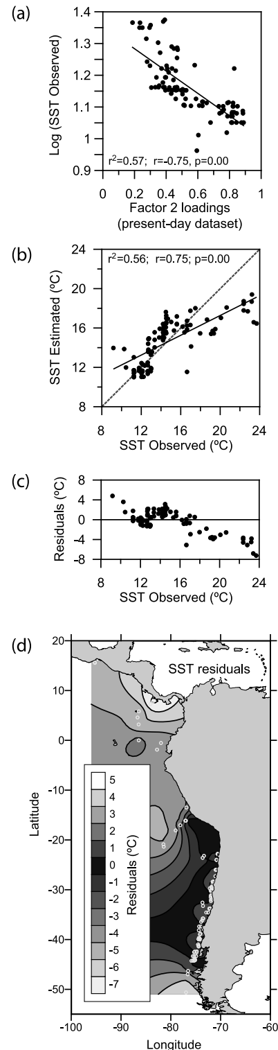
Figure 5. (a) Factor loadings from factor 2 (from the present-day data set) versus measured SSTs (in ^\circ\text{C} ), (b) SSTs measured versus estimated SSTs, (c) observed SSTs versus SST residuals (estimated minus measured, in ^\circ\text{C} ), and (d) SST residuals at core top locations in the equatorial and southeastern Pacific.
