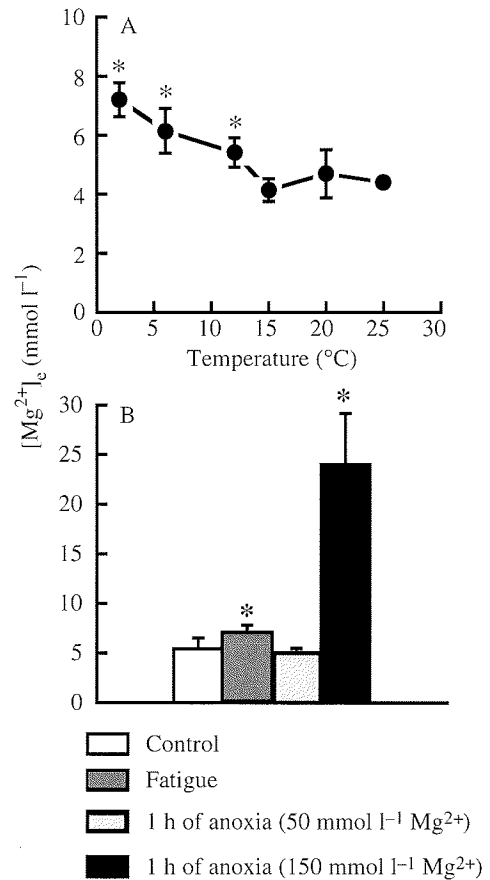
Fig. 3. (A) Extracellular [\text{Mg}^{2+}] as a function of temperature after 4 h of incubation. Each value represents a mean \pm s.d. of at least five animals. * indicates a significant difference ( P < 0.05 ) compared with control levels at 15^\circ\text{C} . (B) Extracellular [\text{Mg}^{2+}] as a result of different treatments. Electrical stimulation was applied until the animals were exhausted (fatigue), whereas anoxic incubations were performed in different media for 1 h. Each value represents a mean \pm s.d. of at least five animals. * indicates a significant difference ( P < 0.05 ) compared with control levels.
