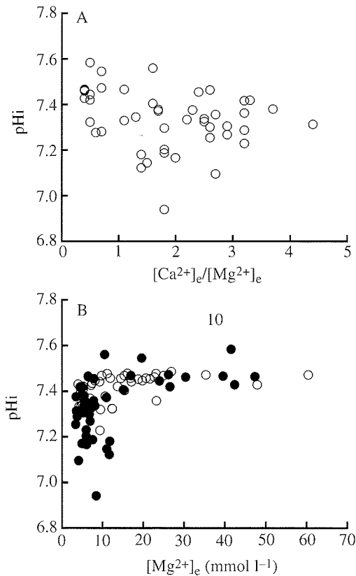
Fig. 2. (A) Relationship between intracellular \text{pH} values and the [\text{Ca}^{2+}]/[\text{Mg}^{2+}] ratio in the haemolymph of Crangon crangon . No significant correlation was detected ( P > 0.05 , r = 0.261 , N = 45 ). (B) Relationship between extracellular [\text{Mg}^{2+}] and intracellular \text{pH} in whole animals (filled circles, temperature incubation series; open circles, incubation in media with elevated [\text{Mg}^{2+}] , 150\text{--}250 \text{ mmol l}^{-1} \text{ Mg}^{2+} ). Both incubation series revealed a threshold level of \text{Mg}^{2+} at approximately 15 \text{ mmol l}^{-1} above which \text{pH}_i values were significantly different from the control ( P < 0.01 ).
