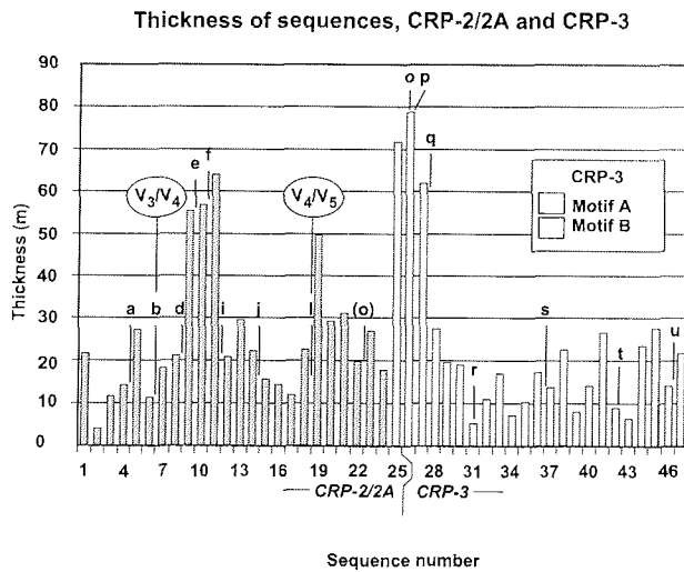
Fig. 4 - Plot of the distribution of sequence thickness in CRP-2/2A and CRP-3, showing the coincidence of sequence boundaries and other horizons with seismic reflectors (from Cape Roberts Science Team, 2000, and see Henrys et al., this volume). The uppermost sequence in CRP-3 (Sequence 25) is constructed on the assumption that the basal part of CRP-2/2A, the underlap between the two holes, and the uppermost part of CRP-3 all lie in one sequence. Note the occurrence of a package of thick (and relatively complete) sequences in the top part of CRP-3 (25-27), similar to Sequences 9-11 of CRP-2/2A. V3/V4 and V4/V5 refer to seismic sequence boundaries, and lower case letters to seismic reflectors.
