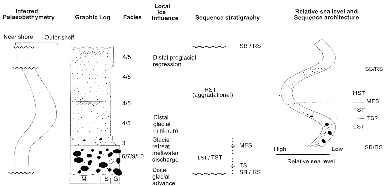
Fig. 3 - Diagram showing the character of sequences in the Cape Roberts drillholes, and their interpretation. A) fully-developed sequence Motif "A", B) less fully developed/cryptic Motif "B". SB/GSE - Sequence Boundary/Glacial Surface of Erosion, SB/RS - Sequence boundary amalgamated with transgressive Ravinement Surface, TS - Transgressive Surface, MFS - Maximum Flooding Surface, RSE - Regressive Surface of Erosion, LST - Lowstand Systems Tract, TST - Transgressive systems Tract, HST - highstand Systems Tract, RST - Regressive systems Tract. Facies codes are explained in Table 1.
