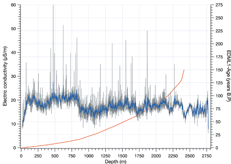
Fig. 23: Profile of the electric conductivity of the EDML ice core as measured by DEP in the science trench at Kohnen Station. Shown are temperature corrected ( -20^{\circ}\text{C} ) values. Breaks were not removed. The data are sampled to 0.5-m intervals (grey). The smoothed curve (blue) shows moving averages over 10 m.
