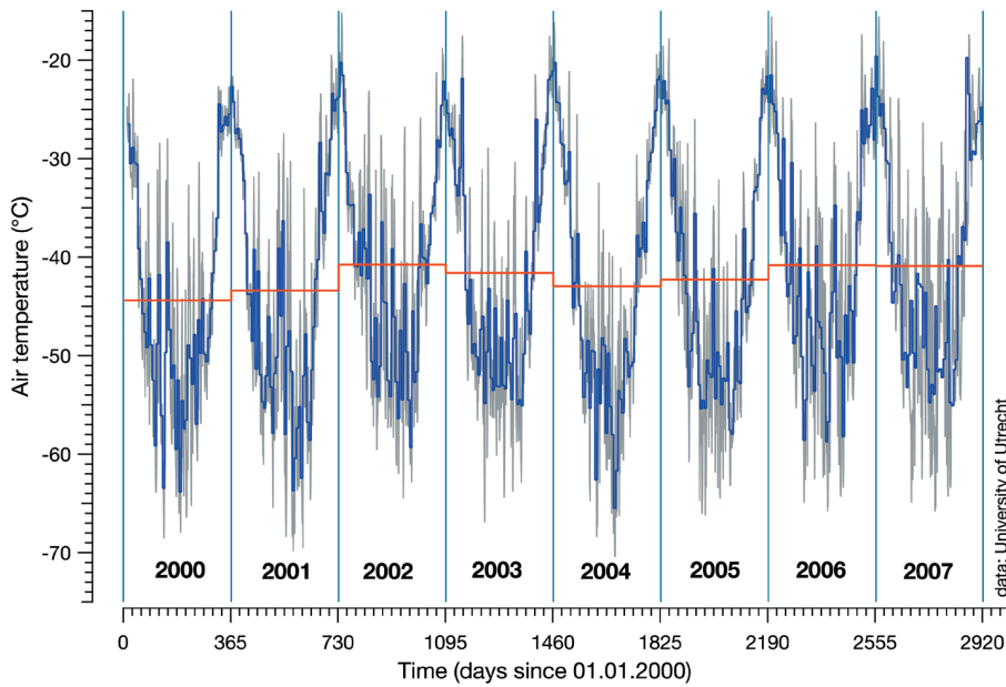
Fig. 4: Air temperature as measured at AWS9, 1.6 km westwards of Kohlen Station, from 2000-2007. Daily means are shown in grey, seven-days means in blue, and annual means in red. Data provided by C.H. Tjim-Rejimer & MR. Van den Broeke, University of Utrecht.
