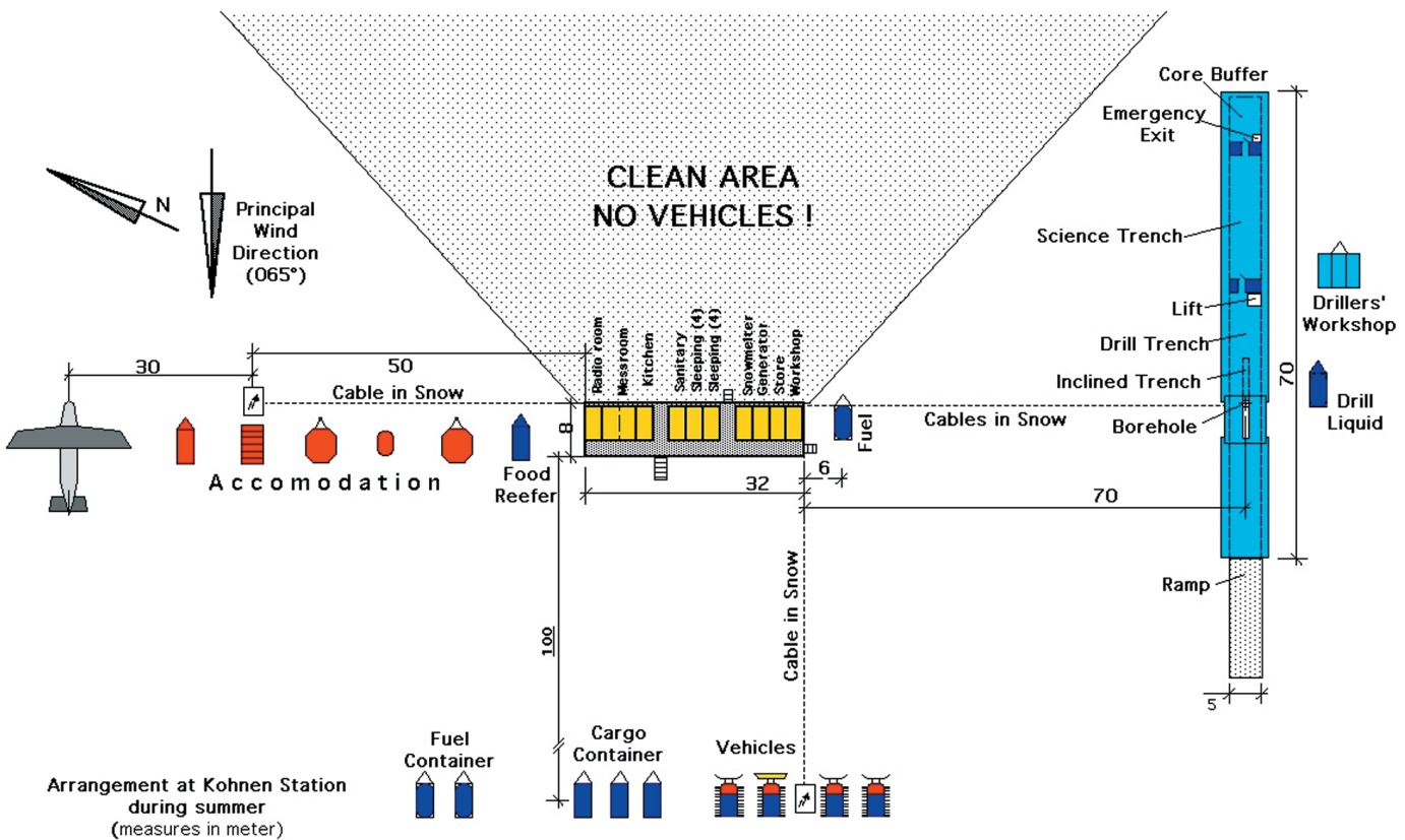
Fig. 12: Layout of the EPICA drill camp with Kohnen Station during drilling operations.
