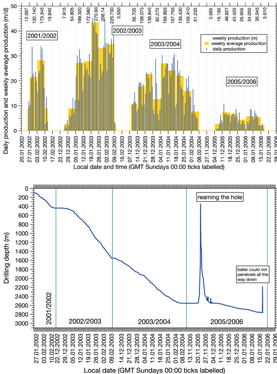
Fig. 20: Progress of drilling the EDML ice core. Top = Daily and weekly production rates for the four drilling seasons. The sticks (blue) give the daily production, while the bars (yellow) give the daily production averaged over one week. The total core production of the week is provided as a figure on top of the graph. Bottom = The penetration of the drill. Given is the final depth of the respective runs.
