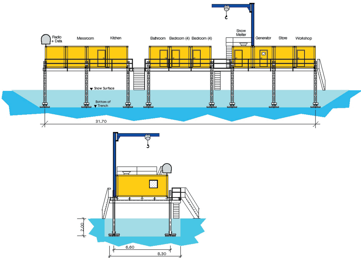
Fig. 9: Kohnen Station in longitudinal view (top) and gable view (bottom) of the container platform. The sketch shows also the foundation of the platform pillars. Using of the different containers is indicated: Radio & data transfer, mess room, kitchen, bathroom, two bedrooms, snow melter, generator, store, and workshop. The snow melter can be filled via an opening in the roof. For this purpose big bags with snow are lifted by the crane above the opening, where they get emptied.
