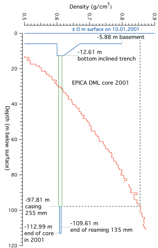
Fig. 19: Cross section through drill trench and cased borehole of the EDML core with density profile. All measures are given in reference to the snow surface on 10 January 2001.
