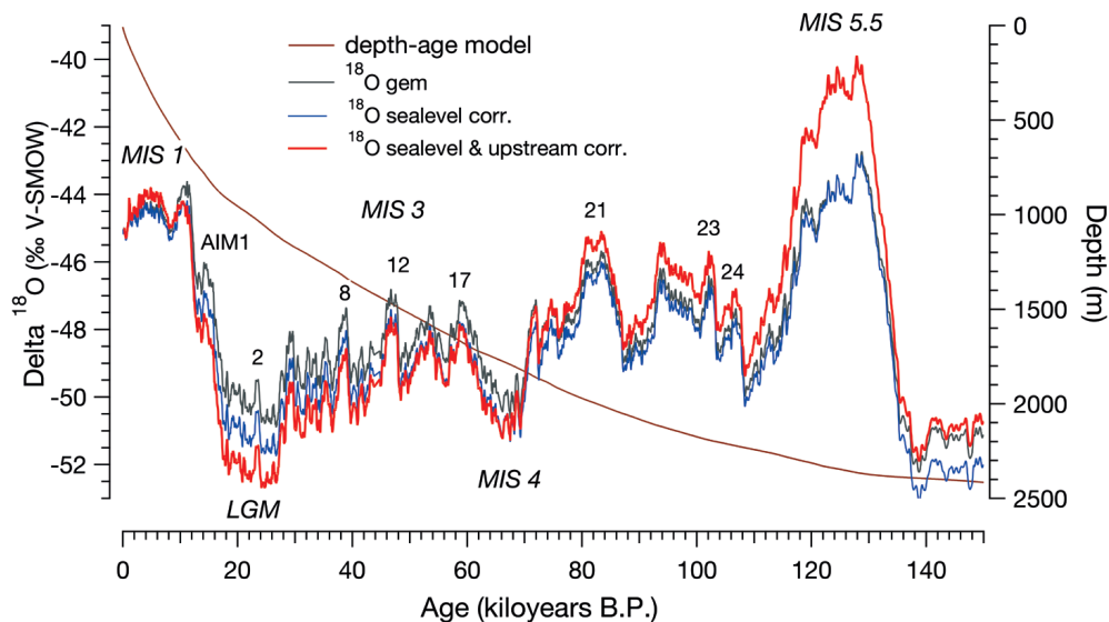
Fig. 30: \delta^{18}O record from the EDML ice core (EPICA COMMUNITY MEMBERS 2006) on the EDML1 age scale (RUTH et al. 2007). The grey curve shows the measured \delta^{18}O data, re-sampled (AnalySeries2.0 software, PAILLARD et al. 1996) to 50-years time steps and smoothed by 5-point running averages. The blue curve shows the same data corrected for changes of the original isotope content of seawater due to changing ice volume in the past (sea level change). The red curve contains in addition the necessary upstream corrections including temporal changes of the elevation of the ice surface. The brown curve represents the correlation between EDML1 age and depth. Some selected Antarctic Isotope Maxima (AIM), the Antarctic counterpart to the Dansgaard-Oeschger-Events in the North, are indicated by figures. MIS = Marine Isotope Stage. LGM = Last Glacial Maximum.
