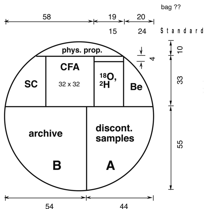
Fig. 24: Cutting scheme for the EDML ice core. The standard width for ^{18}\text{O} , ^2\text{H} and ^{10}\text{Be} samples was 15 and 24 mm. Only some selected bags (bag??), which were used to measure ^{18}\text{O} , ^2\text{H} on a 2.5 cm depth resolution, were cut differently. The core diameter is 98 mm; all measures are given in mm. SC = EPICA Steering Committee can make special arrangements for this piece. CFA = Continuous Flow Analysis. Phys.prop. = physical properties. Discont. samples = samples used for measurements of gas content and isotope ratios in gases as well as dust, which were done not continuously along the whole core.
