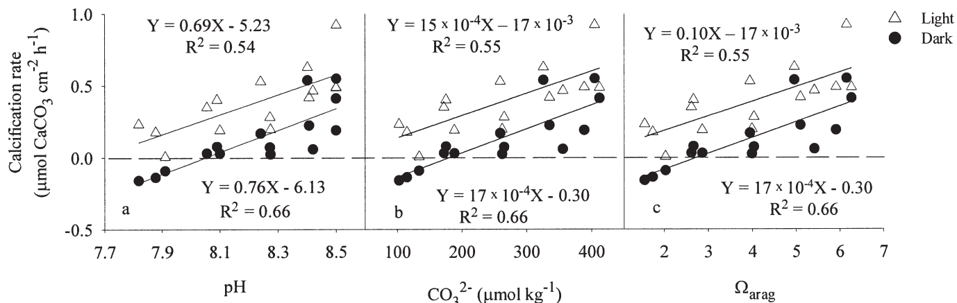
Fig. 1. Calcification as a function of (a) pH, (b) \text{CO}_3^{2-} , and (c) \Omega_{\text{arag}} under light and dark conditions and constant total inorganic carbon ( C_T ).
