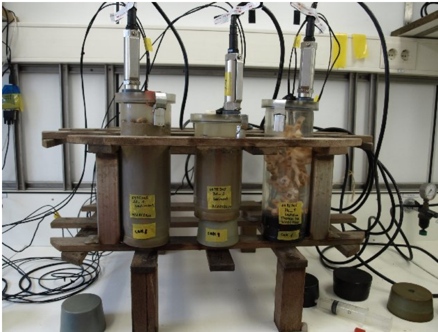
The incubation set-up in the cool container with 2 sedimentcores and one with coral.
