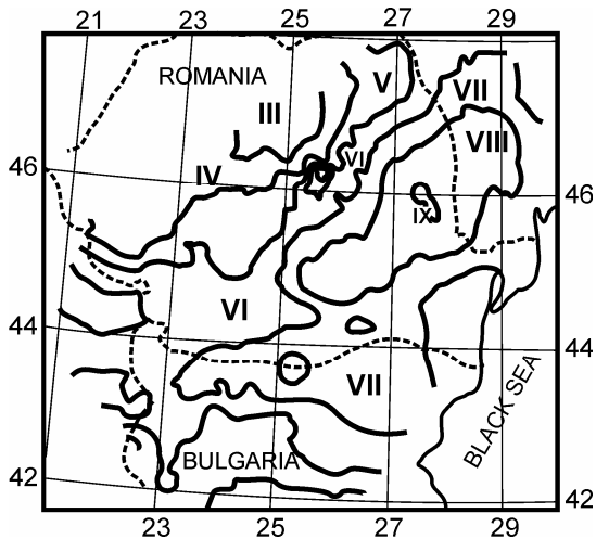
Figure D3. Iseismal maps of the 1940 Vrancea earthquake by De Rubeis et al. (1994). The strange NW-SE elongation of the strongest isoseismal I=IX and small “islands” of intensity VIII to the south of isoseismal I=VIII are not confirmed by the data.
