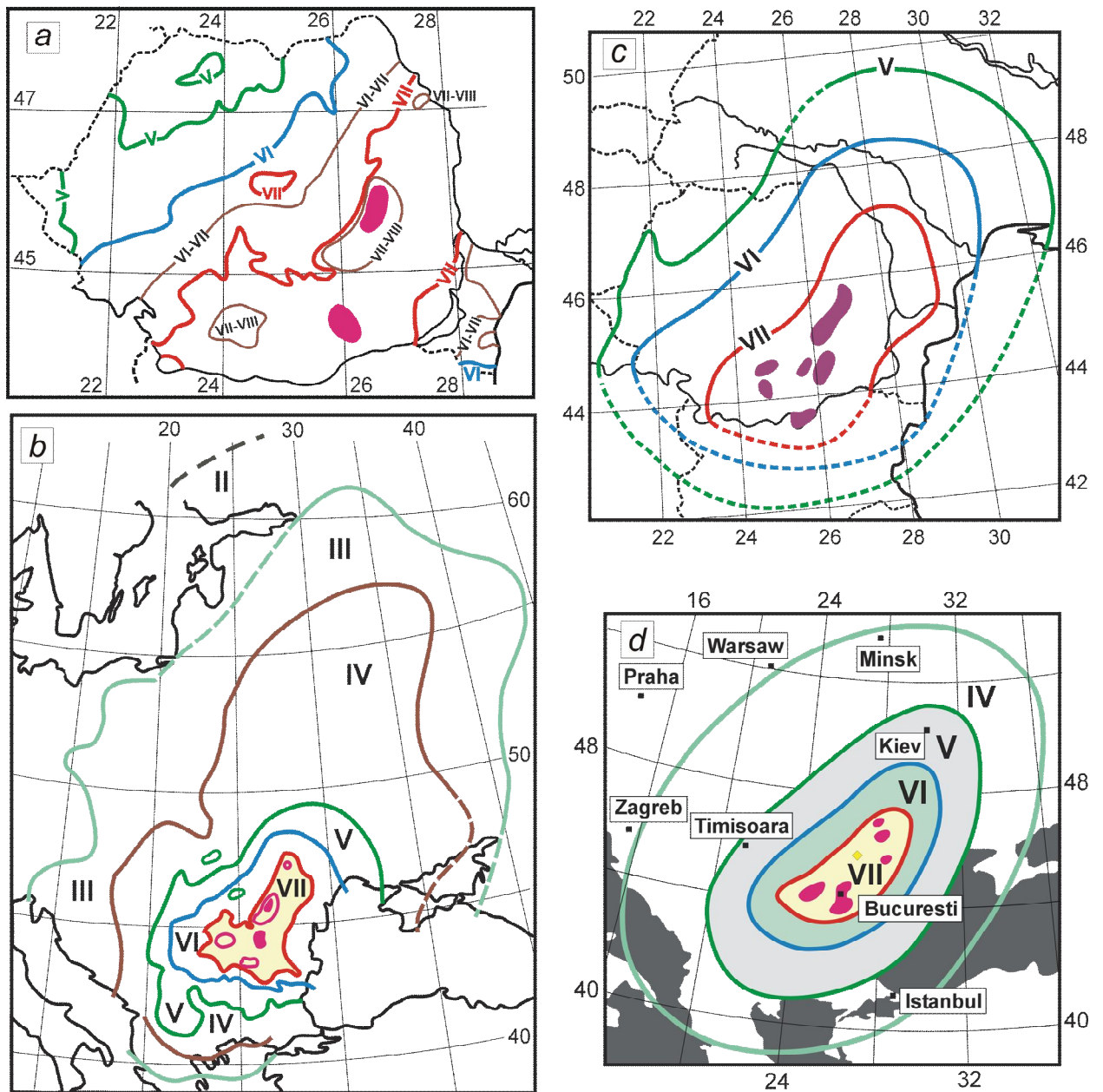
Figure D4. Published isoseismal maps of the 1977 Vrancea earthquake by: (a) Radu et al. (1979b), (b) Radu et al. (1979a); (c) Bune et al. (1986), (d) Shebalin (1977) as reported by Radu et al. (1979b). Red zones in panels (a), (b) and (d) are the areas of I=VIII , while in panel (c) are the areas of I=VII-VIII .
