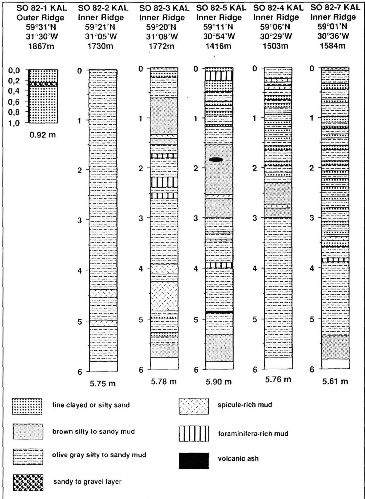
Fig. 3.5.2-2 Lithology of the giant gravity cores
