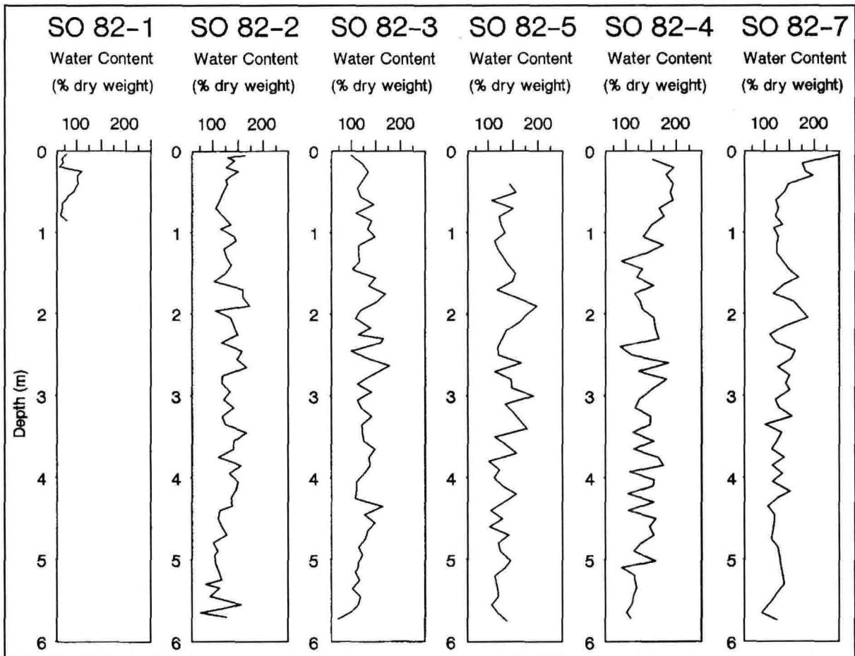
Fig.3.5.3.-2 Natural water content of the giant gravity cores
