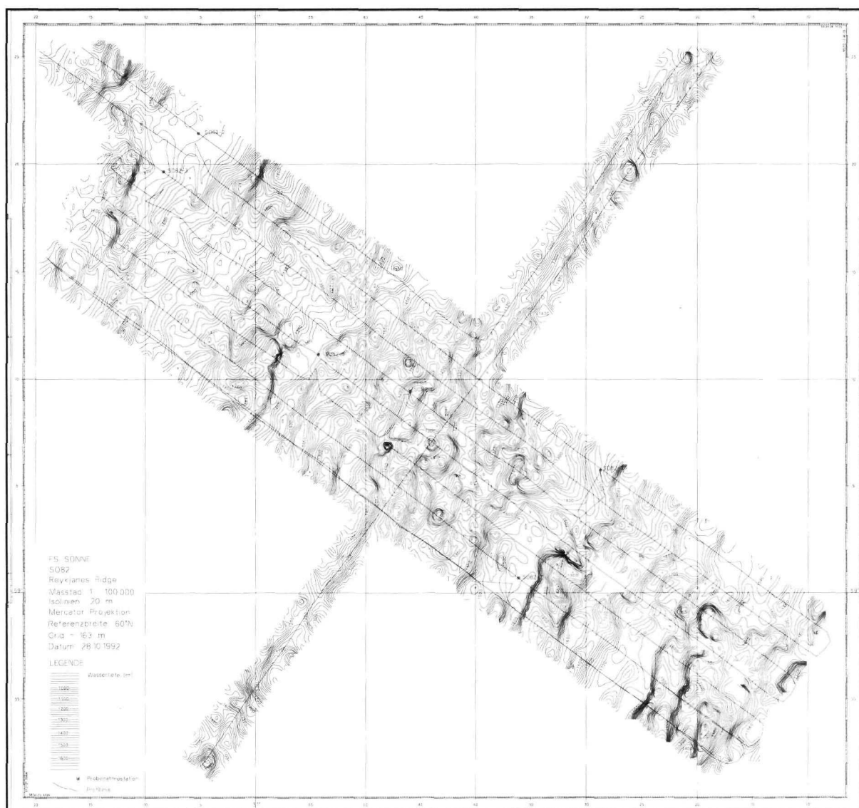
Fig. 3.5.1.-1 Topography of the Reykjanes Ridge near 59° 30'N (copy of a Hydrosweep map, created on board)
