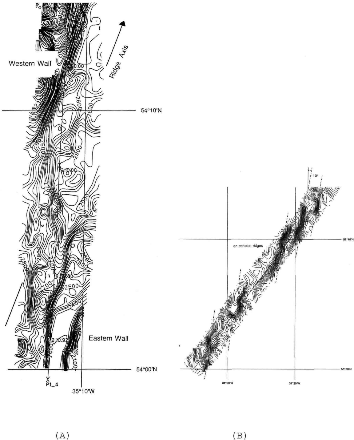
Fig. 2.5.3.-2 Hydrosweep stripes of the Reykjanes Ridge crest, 20 m contour intervall. (A) The southern segment is characterized by a median valley and bounding rift mountains, the valley is dominated by a tectonic graben. (B) En echelon ridges, trending perpendicularly to the spreading direction, but are oblique to the strike of the axis of spreading are located in the rift valley floor of the northern segment.
