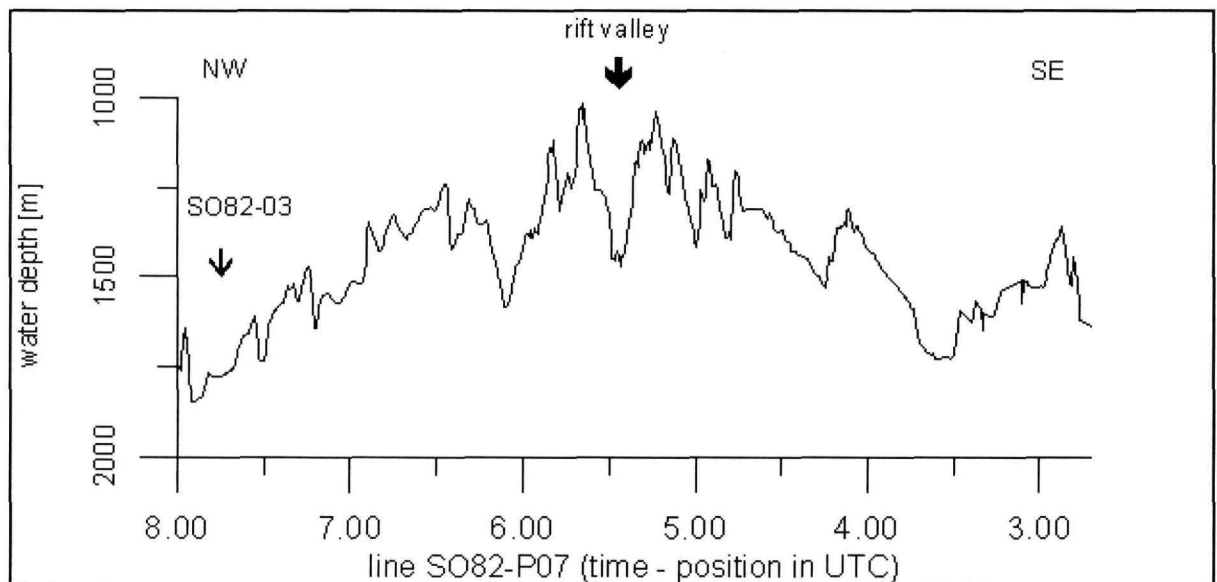
Fig. 3.5.1.-2 Relief of the central part of the Reykjanes Ridge at 59°09'N S082-03 - location of sampling station
