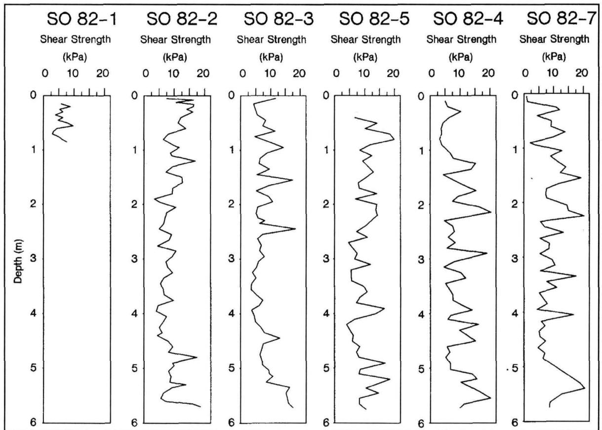
Fig. 3.5.3.-1 Shear strength of the giant gravity cores
