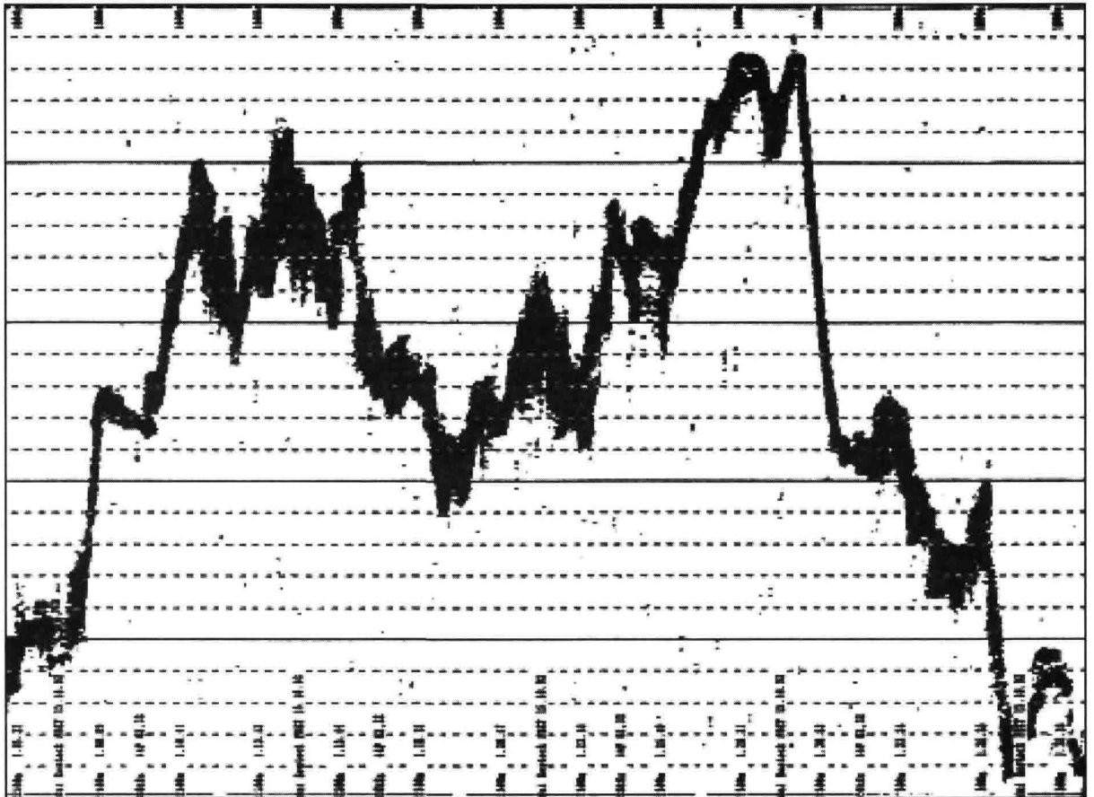
Fig. 2.5.2-2 SEL90 recording (amplitude display, 20 kHz) of a rough sea bottom with slopes up to 60°, depth range 1000 - 1500m, horizontal extension about 12 km
