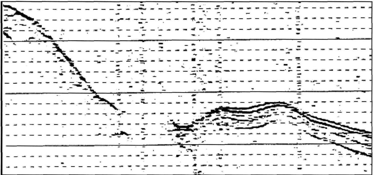
Fig. 2.5.2.-4 SEL90 recording (high resolution mode, 5 kHz) of a sediment pond with a penetration of more than 20 m, depth range 1310-1430 m, horizontal extension about 3.8 km
