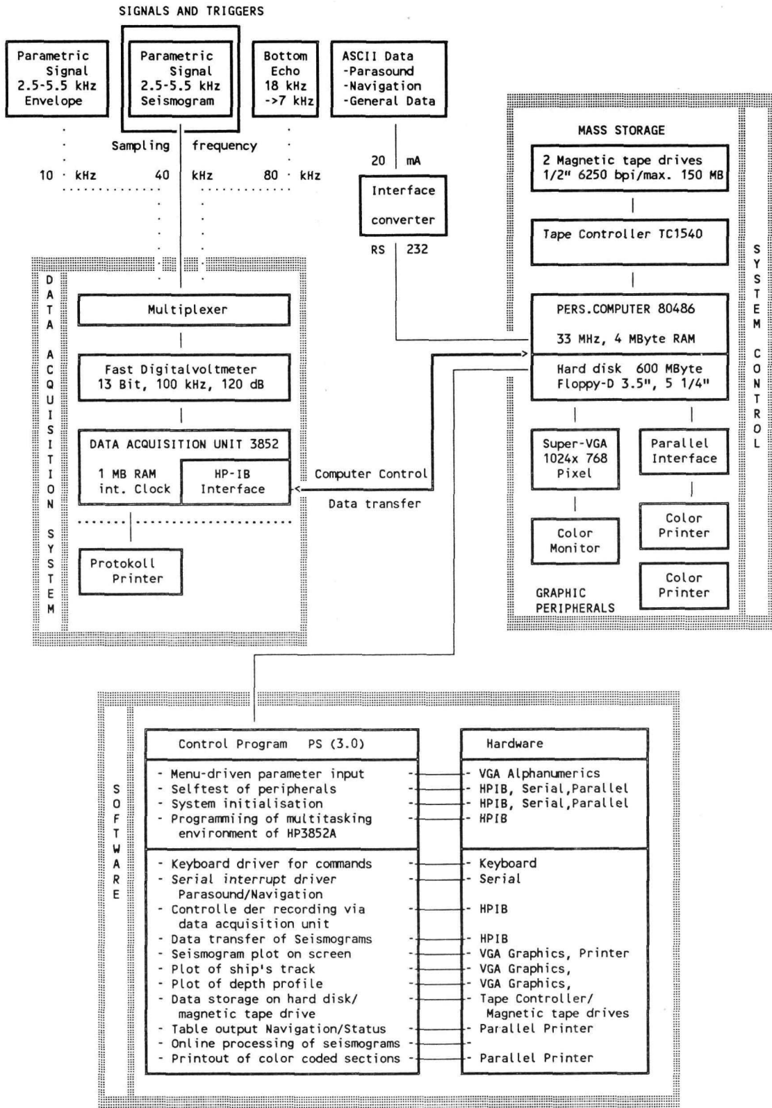
Fig. 2.5.1.-1 Hardware concept and software components of the Paradigma System (PARAsound DIGitizing and Multichannel Analysis System)
