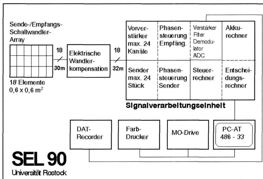
Fig. 2.5.2-1 Configuration of the sediment penetrating echosounder SEL90
