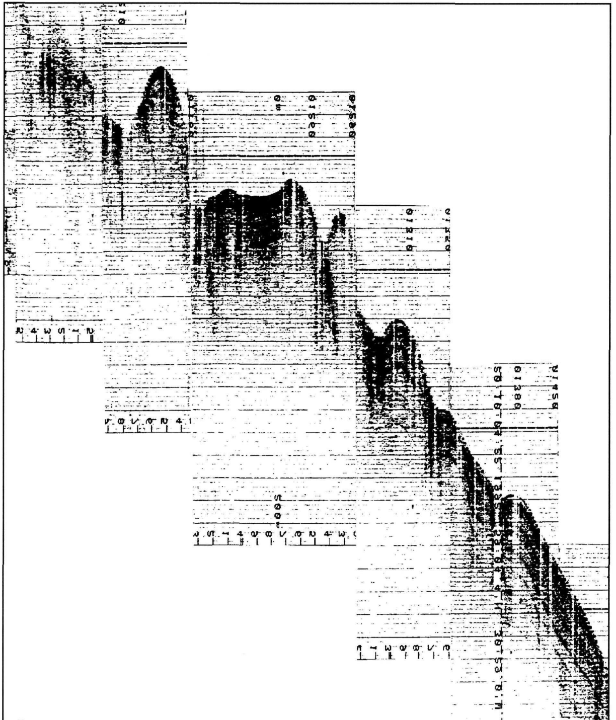
Fig. 3.5.1.-4 PARASOUND record of the eastern slope of the Ridge (see Fig. 3.5.1.-2 line P07, at 4:30 UTC)
