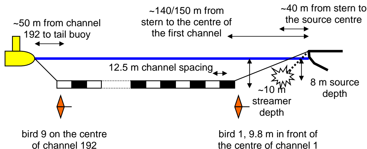
Figure 9: Seismic source and multichannel streamer geometry. The streamer has 192 channels at 12.5 m spacing, for a total length active of 2387.5. The first source-reciever offset was 100 m during the SUMD profiles, and 110 m for all subsequent profiles. Depth control birds were located 9.8 m in front of the centre of channel 1, on channel 24, then every 24 channels to place the ninth bird on channel 192 (Table 3).
