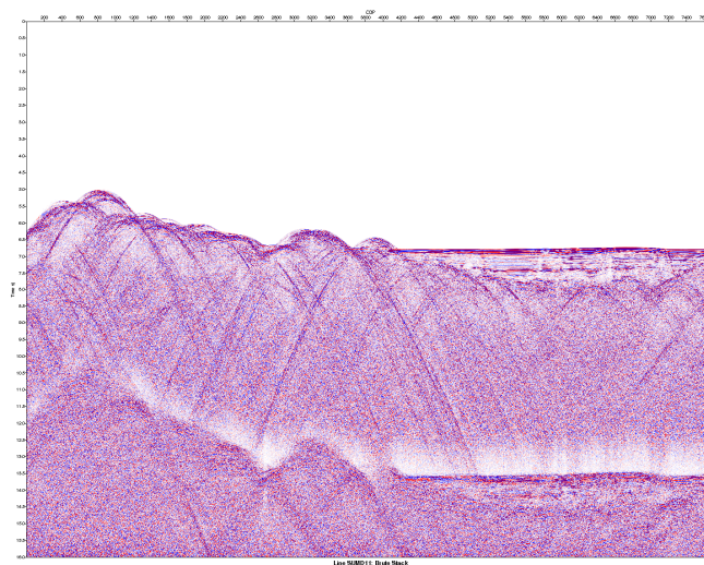
Figure 66: Stacked multichannel seismic section for profile SUMD11.
