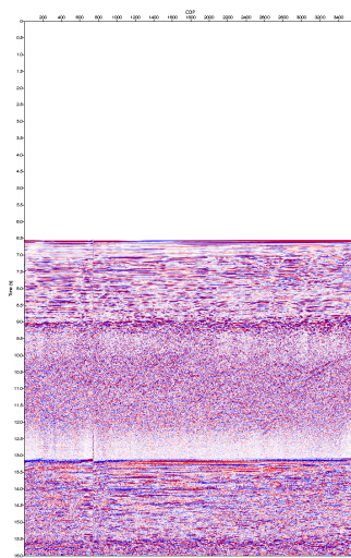
Figure 97: Stacked multichannel seismic section for profile SUME12.
