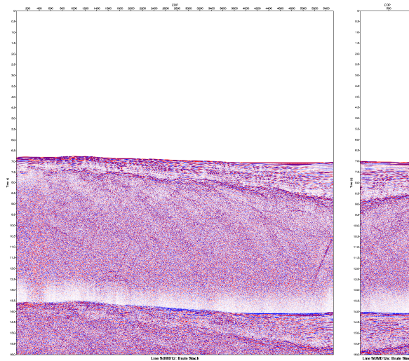
Figure 67: Stacked multichannel seismic sections for profile SUMD12 (left) and SUMD12a (right).
