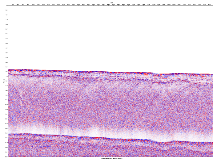
Figure 57: Stacked multichannel seismic section for profile SUMD02.
