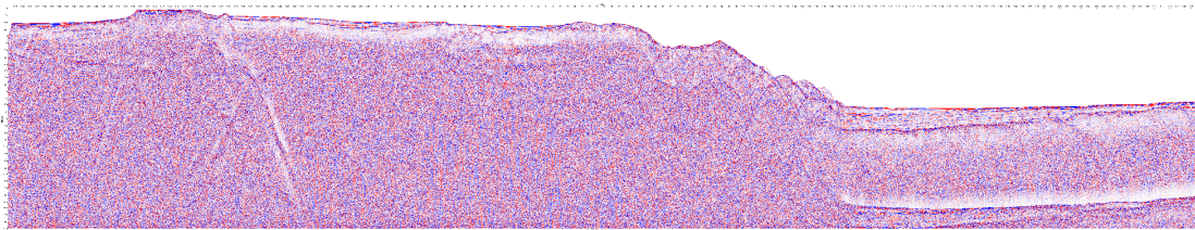
Figure 56: Stacked multichannel seismic section for profile SUMD01b.
