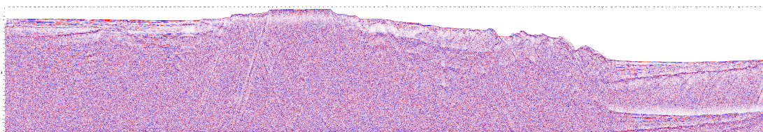
Figure 87: Stacked multichannel seismic section for profile SUME03.
