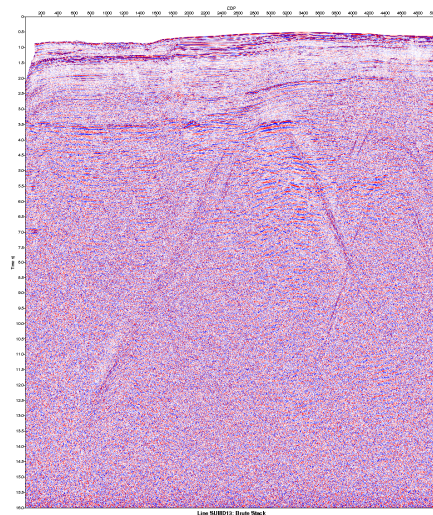
Figure 69: Stacked multichannel seismic section for profile SUMD13.
