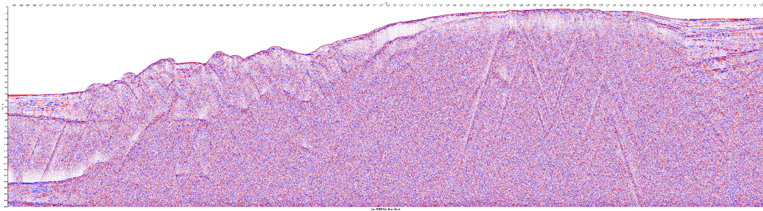
Figure 68: Stacked multichannel seismic section for profile SUMD12b.
