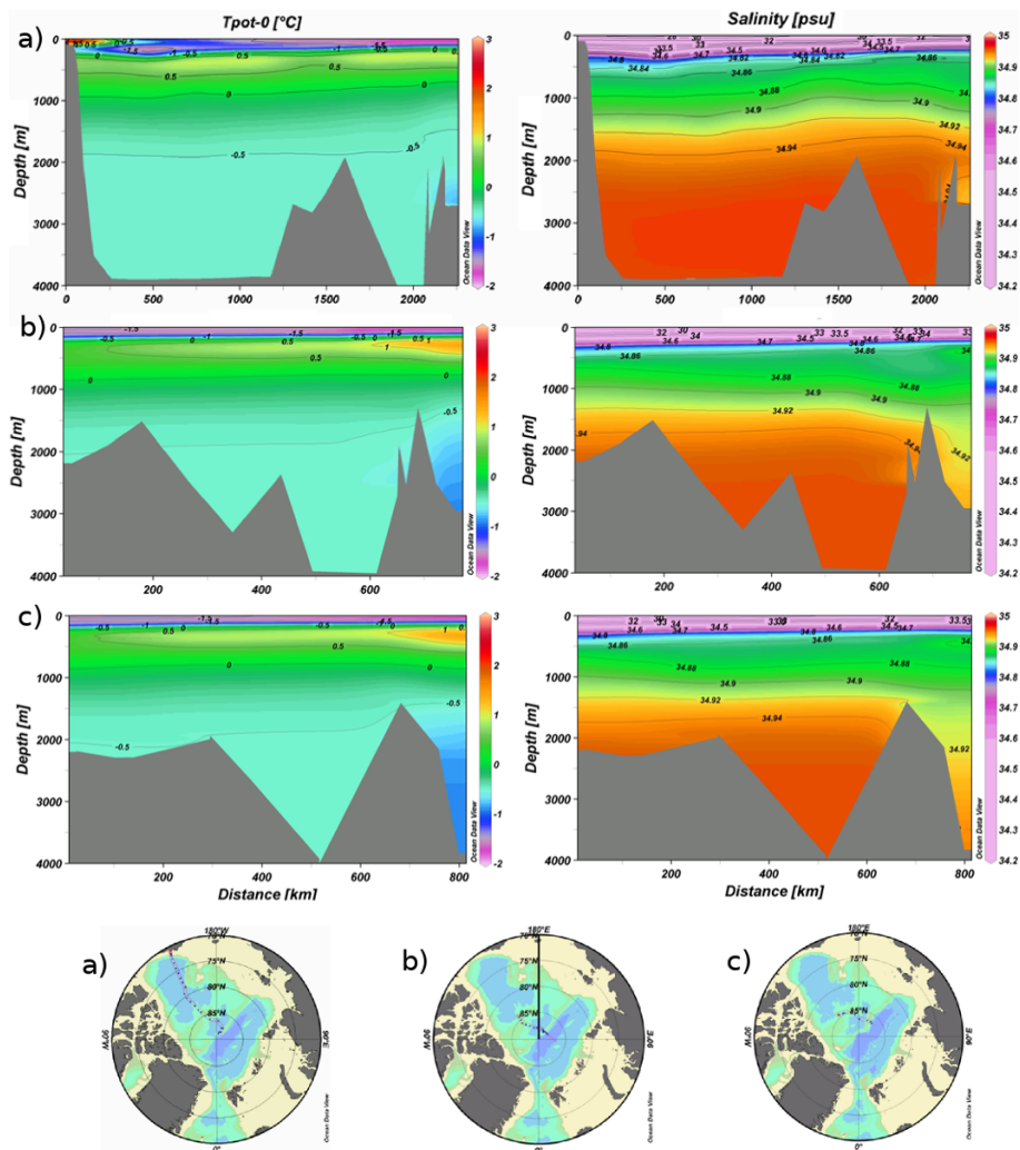
Fig. 1. Upper panel and left map: sections of potential temperature and salinity from Alaska to the Lomonosov Ridge taken by IB Oden in 2005. Centre panel and centre map: sections of potential temperature and salinity between the Alpha Ridge and the Lomonosov Ridge taken by R/V Polarstern 2007 (western section). Lower panel and right map: sections of potential temperature and salinity between the Alpha Ridge and the Lomonosov Ridge taken by R/V Polarstern 2007 (eastern section). Figures are created using Ocean Data View (Schlitzer, 2012).
