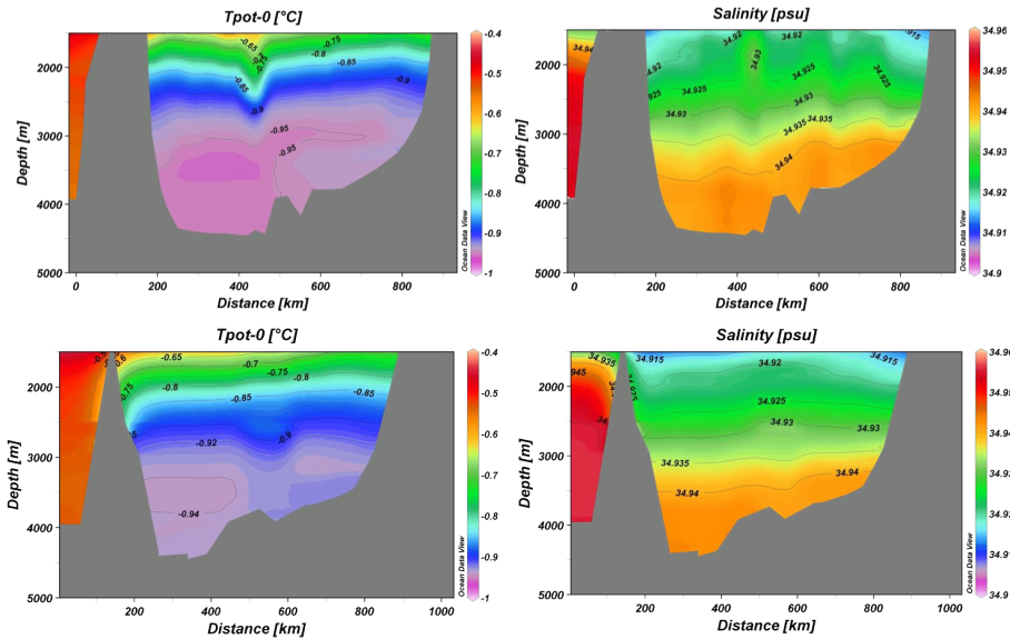
Fig. 22. Potential temperature and salinity sections across the Eurasian Basin taken in 1996 (upper panel) and 2007 (lower panel.) showing the temperature increase, and a possible salinity decrease, below 1500 m. The mean temperature difference is estimated at 0.015\text{ }^{\circ}\text{C} .
