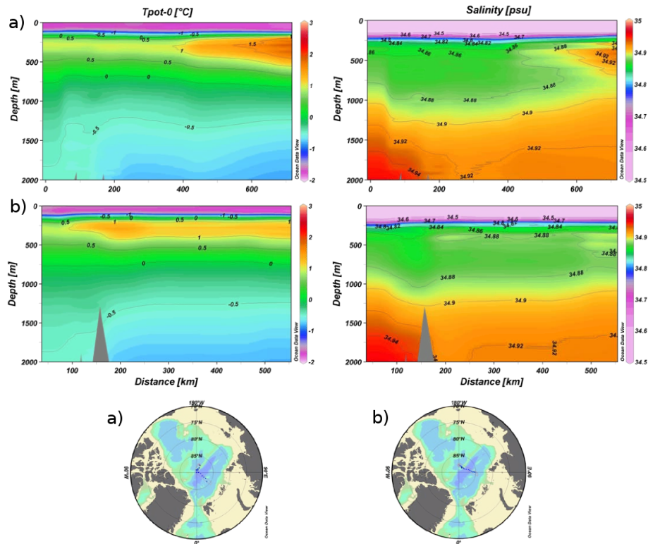
Fig. 16b. Sections of potential temperature and salinity from the Gakkel Ridge (right) across the Amundsen Basin and the Lomonosov Ridge into the Makarov Basin from different years: upper panel and left map – 2005 ( Oden ); lower panel and right map – 2007 ( Polarstern ).
