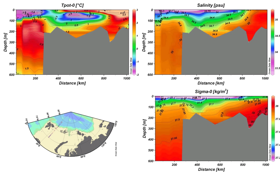
Fig. 3. Potential temperature, salinity and potential density sections from the SPACE transect along 3° E from the Barents Sea into the Nansen Basin.
