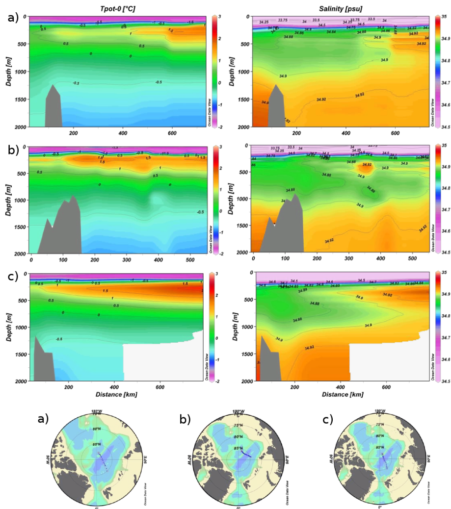
Fig. 16a. Sections of potential temperature and salinity from the Gakkel Ridge (right) across the Amundsen Basin and the Lomonosov Ridge into the Makarov Basin from different years: upper panel and left map – 1991 ( Oden ); centre panel and centre map – 1996 ( Polarstern ); lower panel and right map – 2001 ( Oden ).
