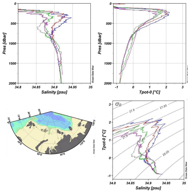
Fig. 10. Profiles of salinity and potential temperature, and \theta S curves from the Laptev Sea slope. No smooth temperature and salinity profiles are seen in the Fram Strait branch Atlantic core, and the presence of intrusive layers indicates mixing between the branches. The Atlantic water is still warmer and more saline over the deeper part of the slope (red and blue stations) than closer to the shelf but has become considerably colder and less saline compared with section 3 (Fig. 9).
