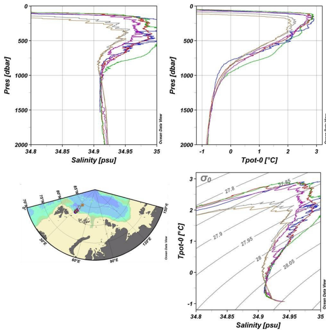
Fig. 6. Profiles of salinity and potential temperature, and \theta S curves from the deep stations on the first SPACE section. Notice the colder, less saline Atlantic water and the salinity minimum at 900 m at the northern stations and the deep (1500 m), weak salinity minimum closer to the slope (better seen in the \theta S diagram).
