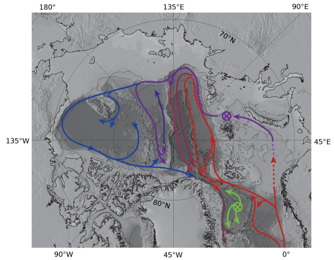
Fig. 15 . Circulation schematics for the Atlantic and intermediate waters showing the two inflow branches and their suggested distribution in the Arctic Ocean. Red colour indicates warm Atlantic water and the Fram Strait branch, and magenta shows the cooled, less saline Barents Sea branch. After the confluence and mixing of the branches north of Severnaya Zemlya, the main part of the Fram Strait branch water returns to Fram Strait in the Nansen Basin (red stream), while the Barents Sea branch dominates in the other basins. The colour scale indicates the amount of Fram Strait branch water present, more in the Amundsen Basin and at the Lomonosov Ridge than in the Makarov Basin. Shelf processes in the Canada Basin change the intermediate water properties, indicated by blue streams and arrows, and part of this water enters the Makarov Basin from the North American slope and flows along the Lomonosov Ridge towards Siberia. The loops from the different basins exit through and merge in Fram Strait. The green streams indicate Arctic Intermediate Water created by convection in the Greenland Sea and partly advected into the Arctic Ocean through Fram Strait. (Figure redrawn from Rudels et al., 2012 and adapted from Rudels et al., 1994.)
