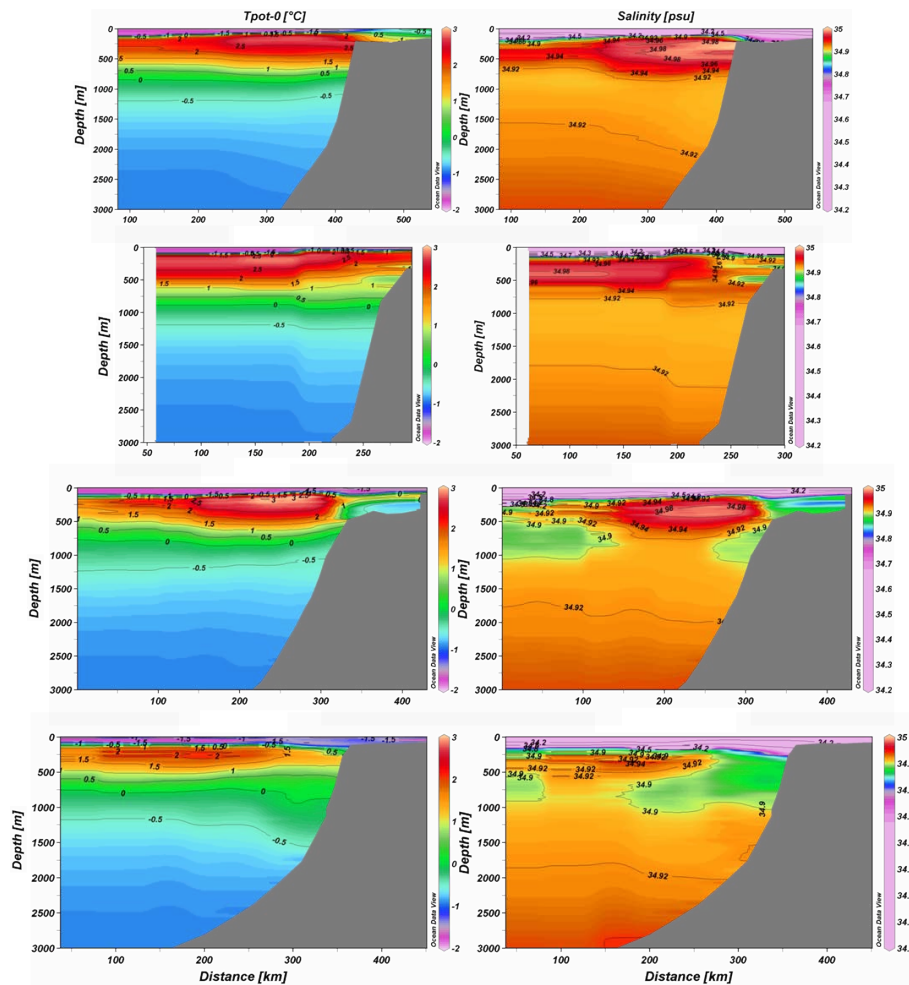
Fig. 11 . Potential temperature and salinity sections from the shelf into the deep Nansen Basin: upper panel – western Barents Sea; upper centre panel – Franz Josef Land; lower centre panel – eastern Kara Sea; lower panel – Laptev Sea.
