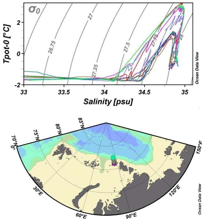
Fig. 4. \theta S curves from the shelf and slope in the eastern Kara Sea showing the colder, less saline Barents Sea branch on the shelf and the warmer, more saline Fram Strait branch on the slope. The winter mixed layers are located above the thermocline, and here the Barents Sea branch is more saline than the Fram Strait branch.
