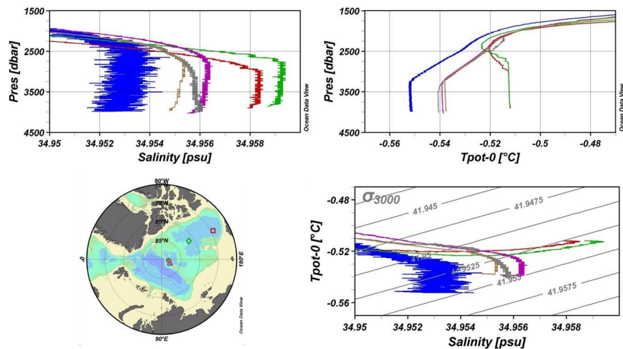
Fig. 21 . Profiles of salinity and potential temperature, and \theta S curves from the Makarov Basin taken in 1991 (blue station), 2001 (grey station), 2005 (magenta station) and 2007 (brown station). The green and blue stations are from the southern (red) and northern (green) taken in 2005. The deep temperature minimum is absent in the Makarov Basin, but the Makarov Basin deep water could supply the temperature minimum of the Canada Basin, which is located at the same level as the sill depth of the Alpha and Mendeleev ridges. The temperature of the Makarov Basin bottom water has increased suggesting either heating or a temporary absence of colder deep water from the Amundsen Basin spilling over the ridge that otherwise would cool the deeper layers. The salinity in the bottom layer might be increasing with time, which would require some influx of the more saline Canada Basin deep water, not just geothermal heating. However, the observed salinity increase is not continuous in time and is very close to instrumental limitations.
