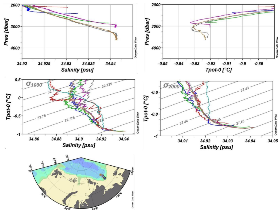
Fig. 19. Profiles of salinity and potential temperature, and \theta S curves from SPACE section 4 north of the Laptev Sea. Here the slope of the deeper part of the \theta S curves has become more perpendicular to the isopycnals, indicating both a salinity reduction due to the Barents Sea inflow and a deeper salinity increase due to slope convection and entraining, saline and dense plumes bringing heat and salt downwards. Bottom water with increasing temperature and salinity with depth are observed at the slope between 2000 m and 3500 m (blue, green and magenta stations).
