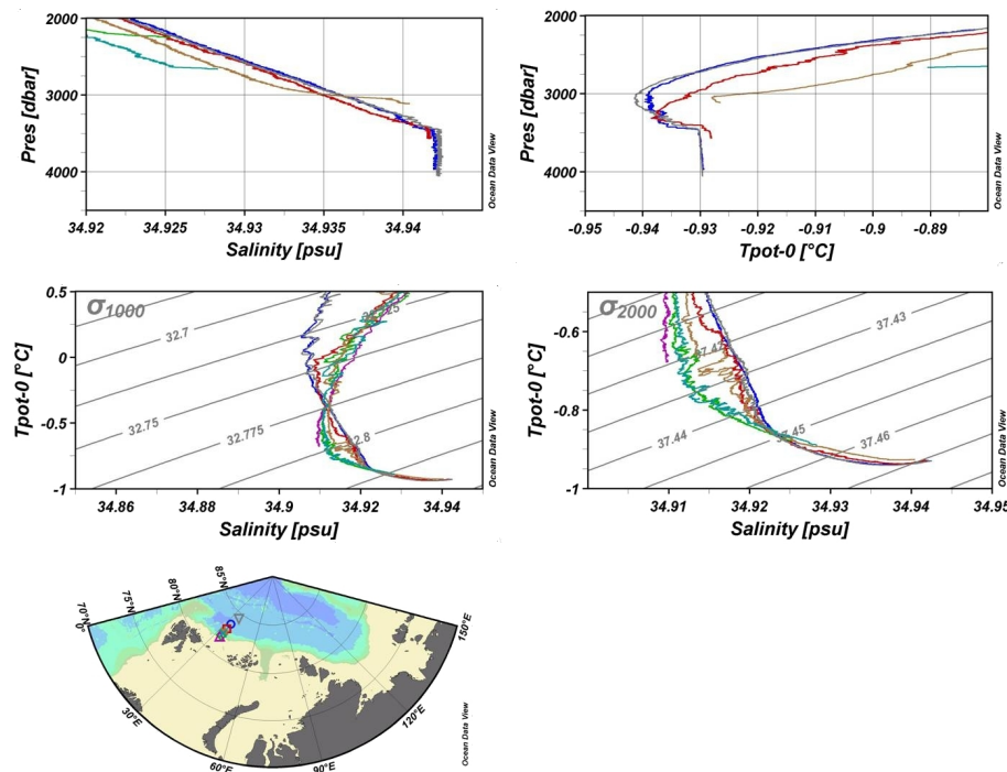
Fig. 17. Profiles of salinity and potential temperature and \theta S curves showing the characteristics of the deep and bottom water in the Nansen Basin on the SPACE section along 33^\circ\text{E} and the presence of then deep temperature minimum and the homogenous bottom layer below (profiles) and the less saline deep inflow from the Nordic seas through Fram Strait ( \theta S curves).
