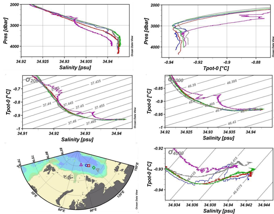
Fig. 20 . Profiles of salinity and potential temperature, and \theta S curves shown with different blow-up levels from SPACE stations taken above the Gakkel Ridge. The simple deep water structure found in the basins is here disrupted by several different maxima and minima. A strong input of warmer and more saline water is found at 2700 m (magenta station), and a smaller deep intrusion is seen between 3100 m and 3300 m (blue station). The cause of these maxima could be geothermal activity at the ridge.
