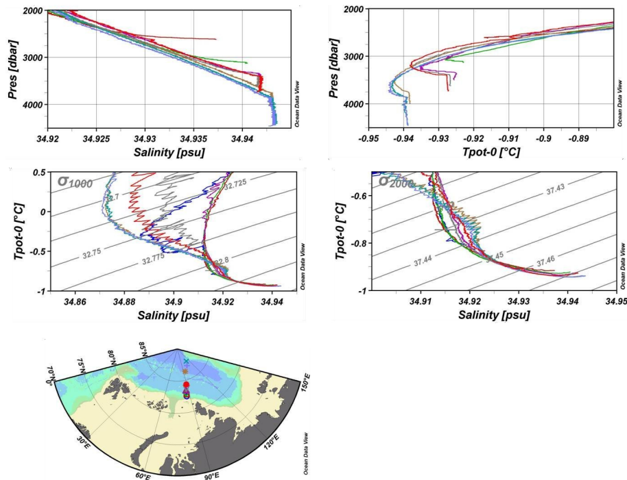
Fig. 18. Profiles of salinity and potential temperature and \theta S curves showing the deep and bottom water in the Nansen and Amundsen basins along SPACE section 3. A deep temperature minimum and a homogenous bottom layer are present in both basins. The Amundsen Basin is deeper and its bottom water colder and more saline. In the \theta S curves the less dense salinity minimum, found both at the slope (blue station) and in the interior, is derived from the Barents Sea inflow. The deep salinity maximum is observed in the Amundsen Basin and indicates an inflow of Amerasian Basin deep water across the Lomonosov Ridge.
