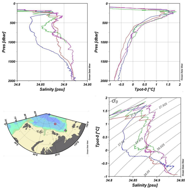
Fig. 23. Profiles of salinity and potential temperature and \theta S curves showing different eddies observed on the SPACE cruise 2007. Especially the 800-m-thick eddy of Barents Sea branch water found in the intra-basin in the central Lomonosov Ridge (blue station) is remarkable.
