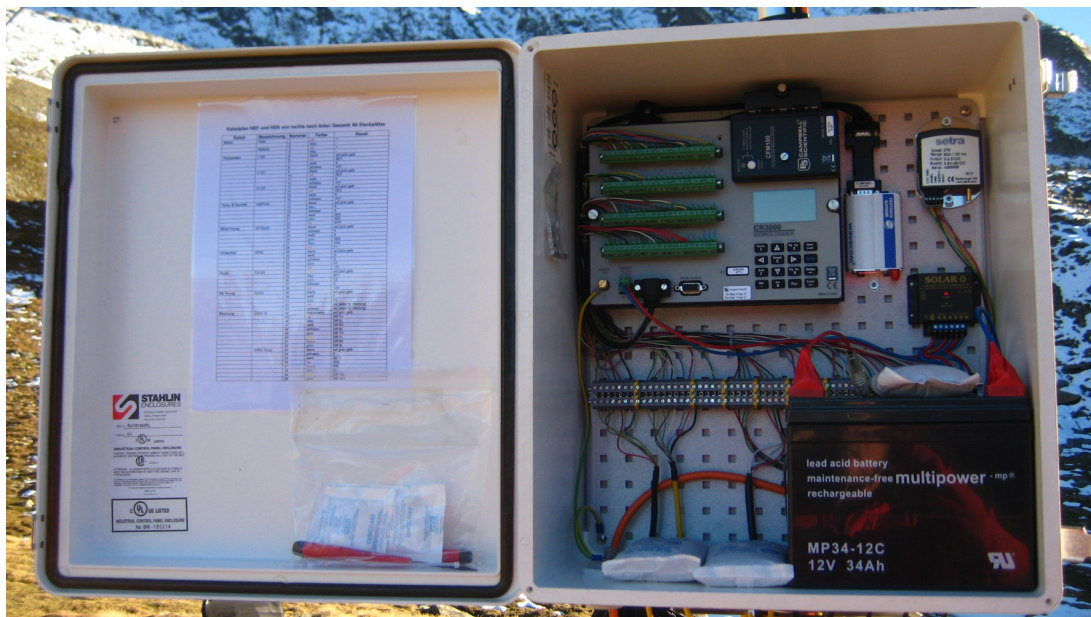
Figure 2.5: Enclosure of the AWS.
