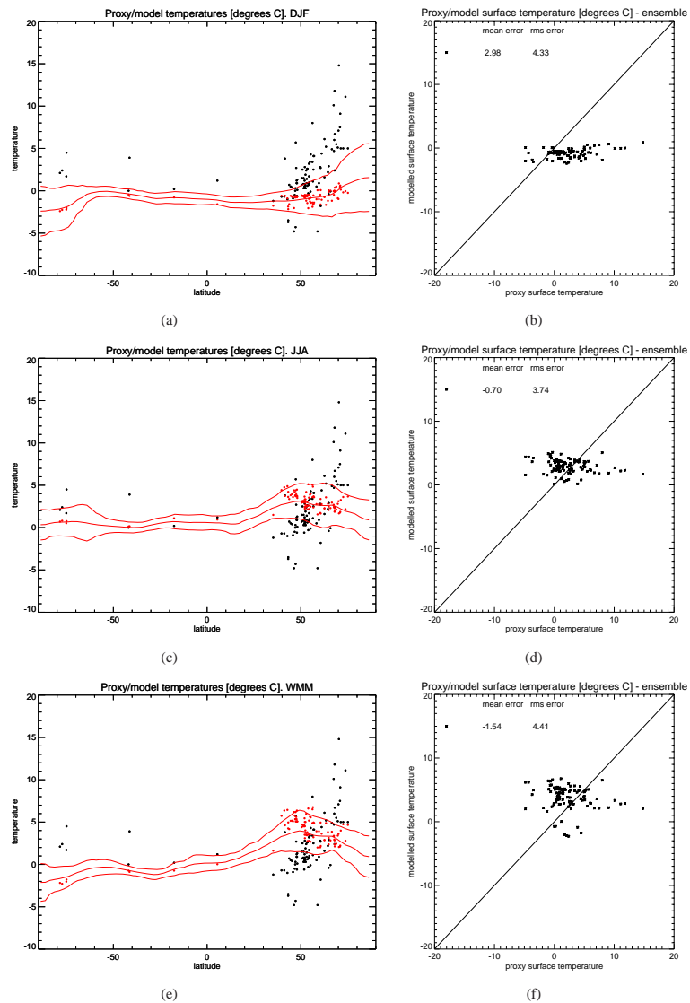
Fig. 8. Comparison of ensemble mean surface air temperature change, LIG minus pre-industrial, with data from Turney and Jones (2010). (a, c, e) Latitudinal distribution of data (black dots), compared with the ensemble mean model (red dots, from the same locations as the proxy data), with the zonal model ensemble mean (thick red line), and \pm 1 standard deviation of the zonal model ensemble mean (thin red lines). (b, d, f) Modelled ensemble mean temperature vs. proxy data temperature for each terrestrial site in the Turney and Jones (2010) dataset. (a, b) are for DJF, (c, d) are for JJA, and (e, f) are for WMM. All units are ^{\circ}\text{C} .
