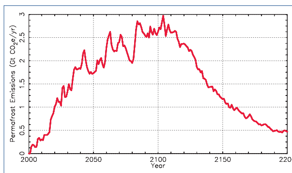
Figure 22: CO 2 and methane emissions from thawing permafrost can continue for decades or even centuries, as seen in this plot of estimated annual permafrost emissions in CO 2 equivalent for the IPCC A1B scenario. In this scenario, anthropogenic emissions stop in 2100, but permafrost CO 2 and methane emissions continue well past 2200 (Schaefer et al. 2011)
