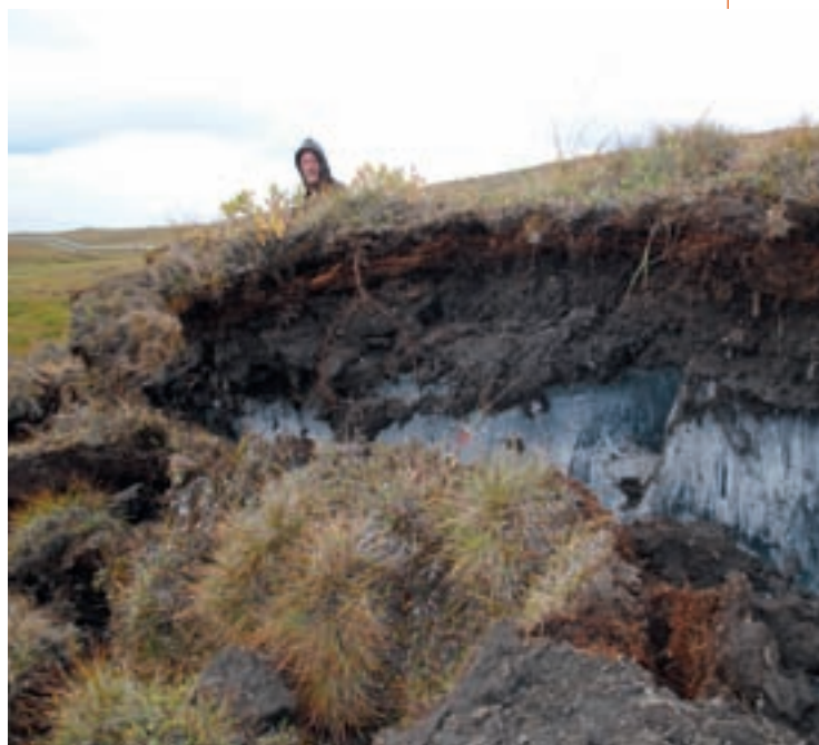
Figure 6: A typical thermokarst depression forms when melting ground ice causes the overlying vegetation and soil to collapse. This thermokarst depression formed when an ice layer about one meter thick melted in continuous permafrost on the North Slope of Alaska (Photo: Kevin Schaefer).
