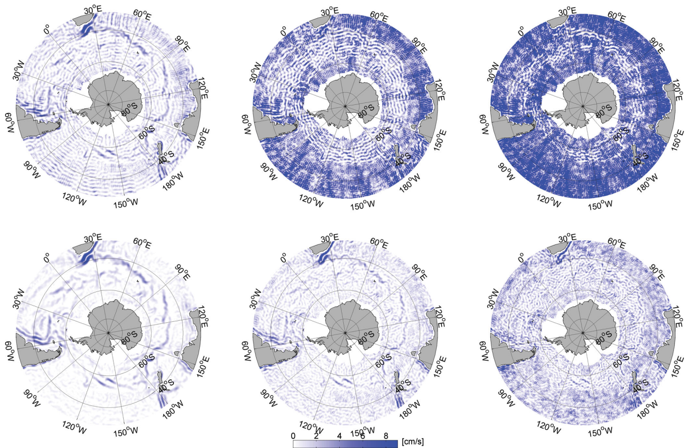
Figure 6. Magnitude of the geostrophic velocities in different spectral bands computed from MDT using ITG-Grace2010 (upper panel) and GOCE-TIM3 (lower panel) gravity models. The harmonic components from 90 to 120 (left), from 120 to 150 (middle) and from 150 to 180 (right) are shown. Units are \text{cm s}^{-1} .
