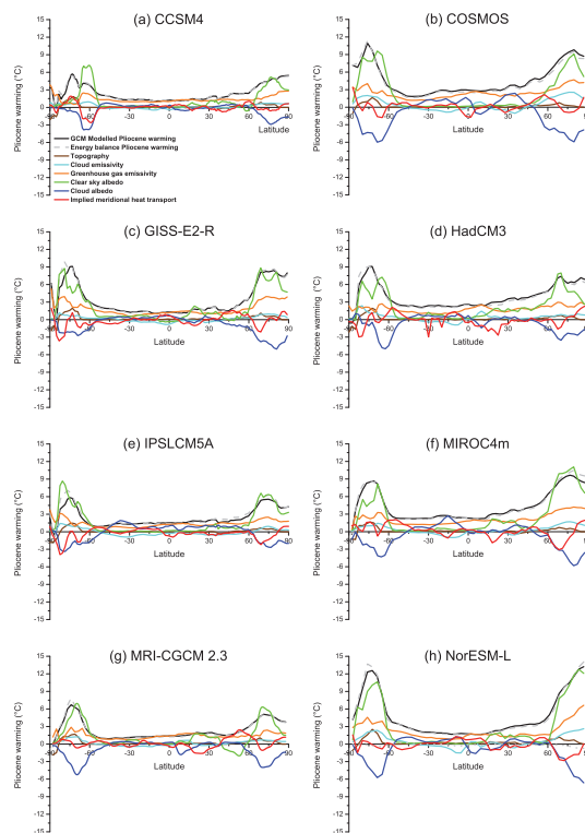
Fig. 2. Energy balance analysis for each of the eight PliocMIP Experiment 2 simulations, from (a) CCSM4, (b) COSMOS, (c) GISS-E2-R, (d) HadCM3, (e) IPSLCM5A, (f) MIROC4m, (g) MRI-CGCM 2.3 and (h) NorESM-L. Plots show the zonal mean warming, at each latitude in the model, from each of the energy balance components. Solid black line is the zonal mean surface air temperature increase from the GCM simulation, while the dashed grey line is the Pliocene warming approximated by the energy balance calculations.
