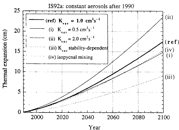
Fig. 5. Sea-level contribution of thermal expansion (cm) from 1990 to 2100 for the updated IS92a Scenario with aerosols constant at the 1990 level: results are shown for the reference case and for 4 alternative parameterizations of the ocean heat mixing.
