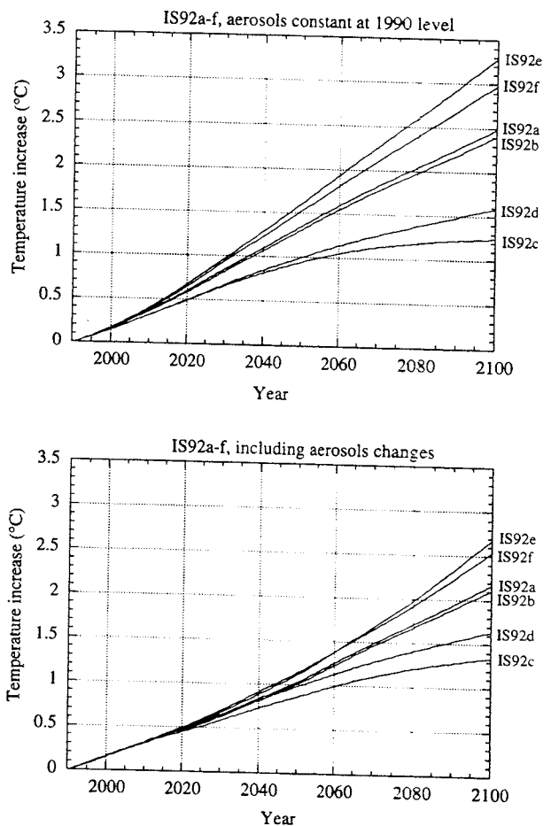
Fig. 2. Global and annual mean atmospheric temperature changes (°C) from 1990 to 2100, calculated with the zonal mean climate model for the updated IS92 radiative forcing scenarios, with aerosols constant at the 1990 level (upper plot) and with the inclusion of aerosol changes (lower plot).
