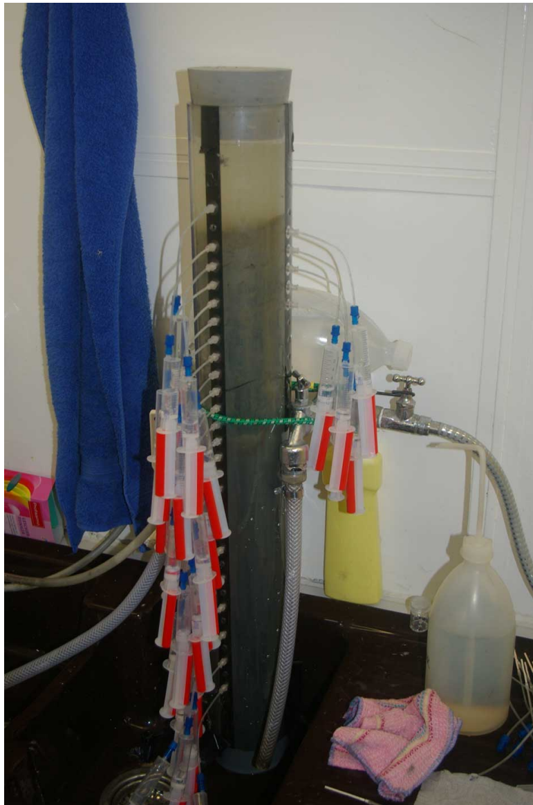
Fig. 4.4-3: The use of rhizons for the extraction of pore waters.
