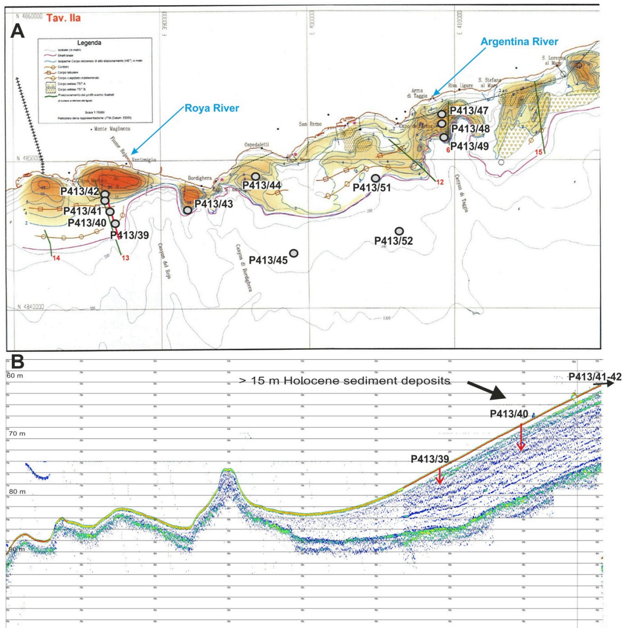
Fig. 4.4-13: (A) Thickness of Holocene sediments on the western Ligurian shelf (Corradi et al., 2004) with core locations during cruise P413. (B): Shelf transect off the mouth of the Roya River with coring locations.
