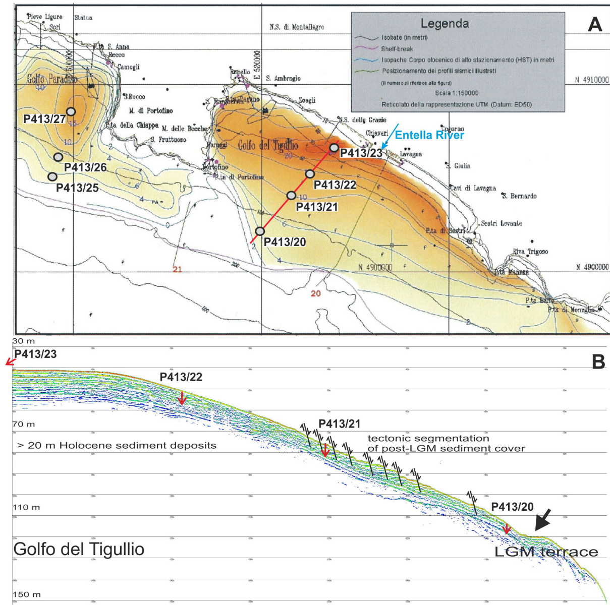
Fig. 4.4-9: (A) Thickness of Holocene sediments in the Gulf of Tigullio (Corradi et al., 2004) with core locations during cruise P413. (B): Shelf transect in the Golfo del Tigullio with coring stations.
