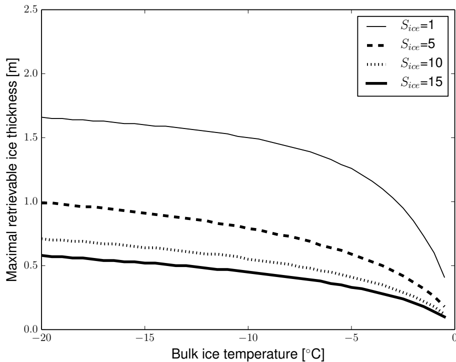
Fig. 6. d_{max} under different T_{ice} [°C] and S_{ice} [ g\ kg^{-1} ].
