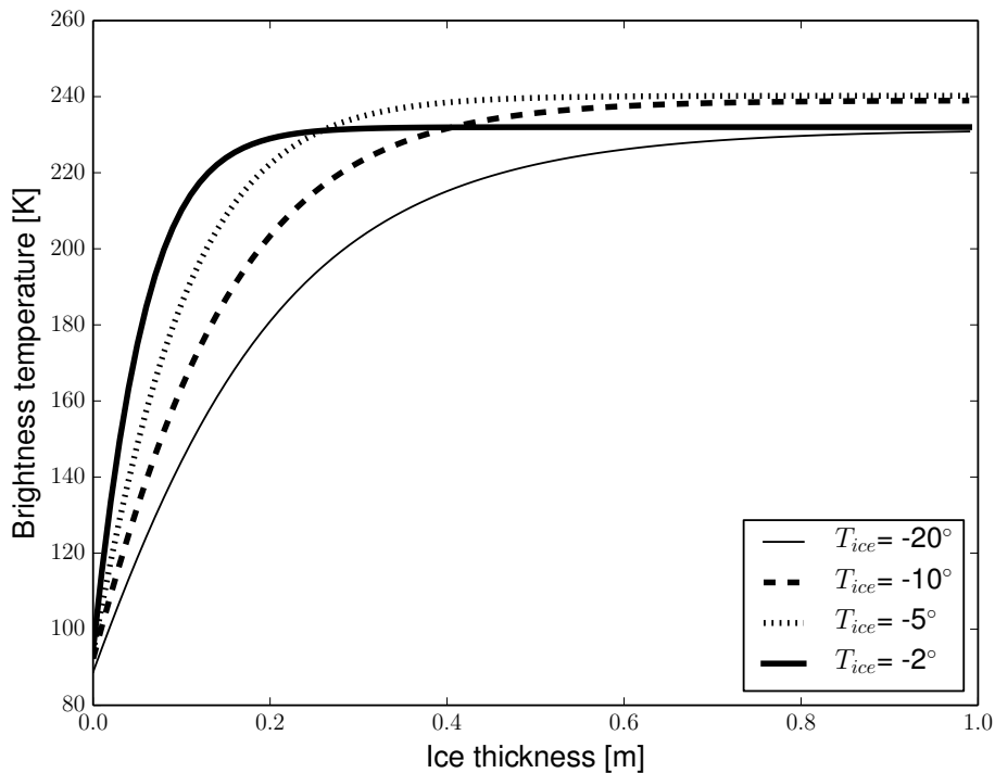
Fig. 5. TB as function of d_{ice} under different T_{ice} , calculated with the sea ice radiation model with a S_{ice} of 8 \text{ g kg}^{-1}
