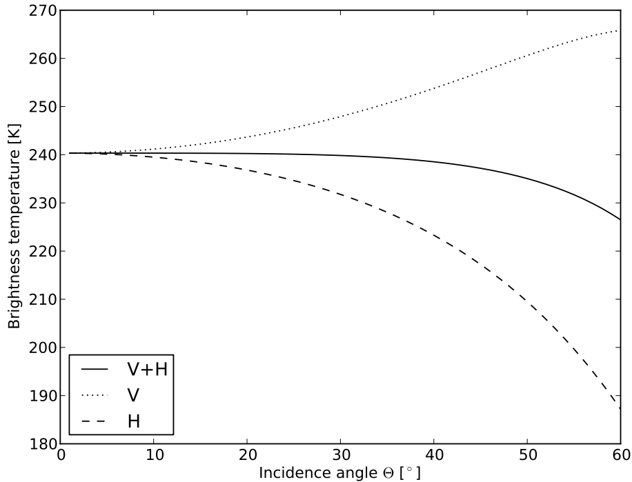
Fig. 3. Vertically (V) and horizontally (H) polarized TBs and the first Stokes parameter as a function of incidence angle calculated using a three layer model for sea ice with a thickness of d_{\text{ice}} = 1 m, a bulk salinity of S_{\text{ice}} = 8 \text{ g kg}^{-1} , and a bulk ice temperature of T_{\text{ice}} = -7^\circ\text{C} .
