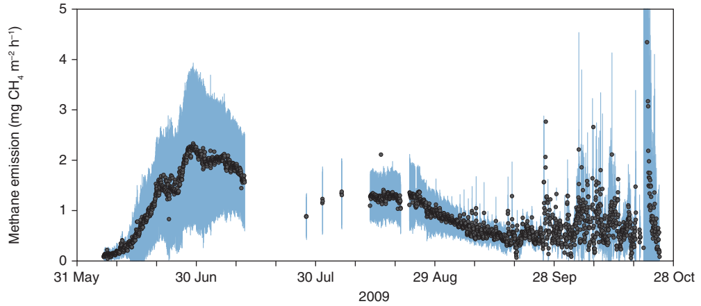
Figure 2.14 Methane ( \text{CH}_4 ) emissions 2009.
