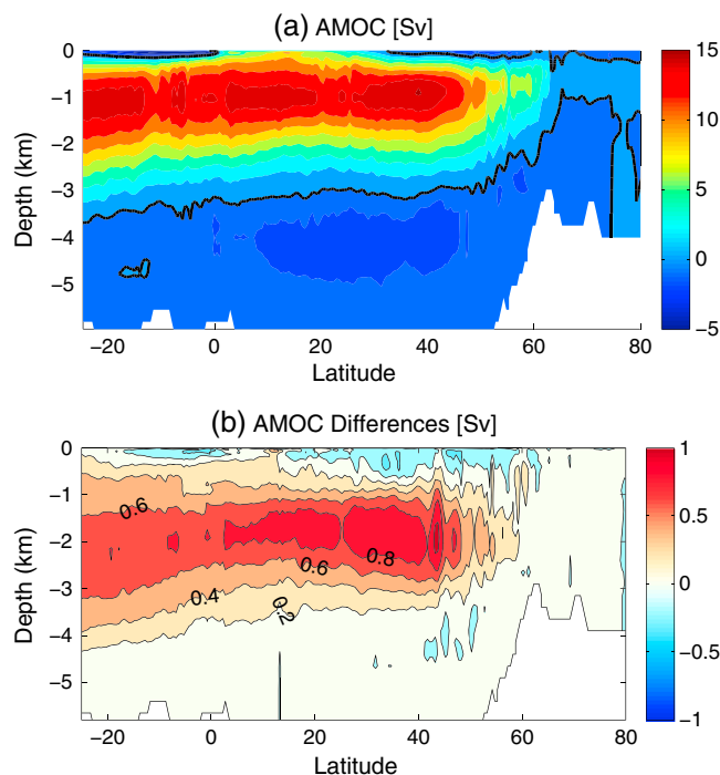
Figure 3. Same as in Figure 2, except for the Atlantic Meridional Overturning Circulation (in Sv) as a function of depth and latitude.
