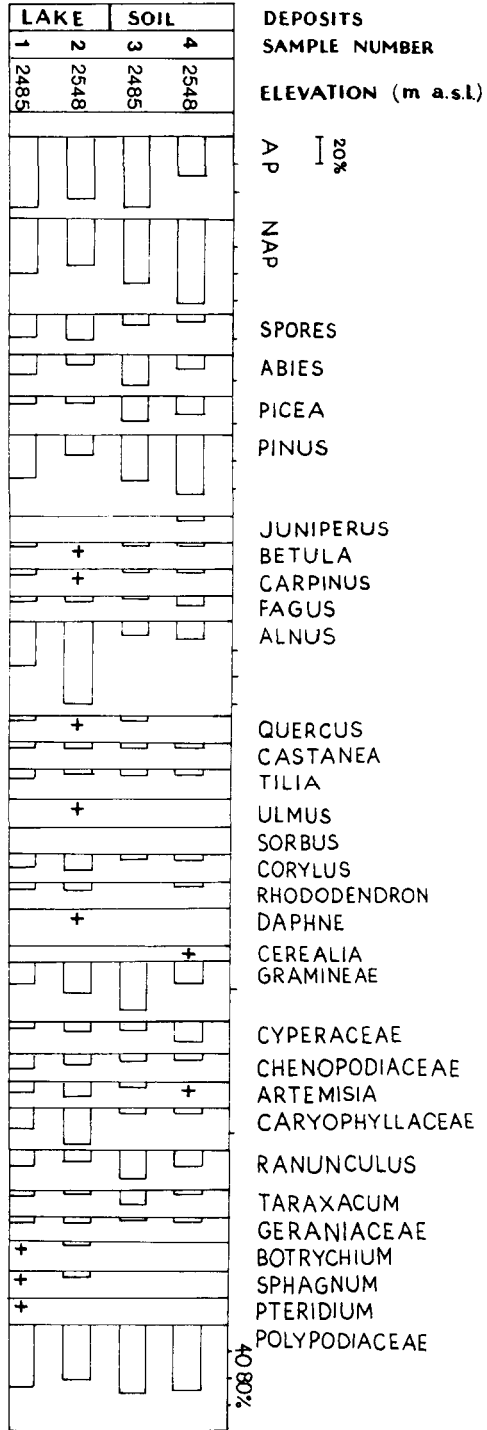
Fig. 1. Spore-pollen diagram of recent sediments at the headwaters of the river Bezymianka 1, 2 - lake samples, 3, 4 - soil samples
