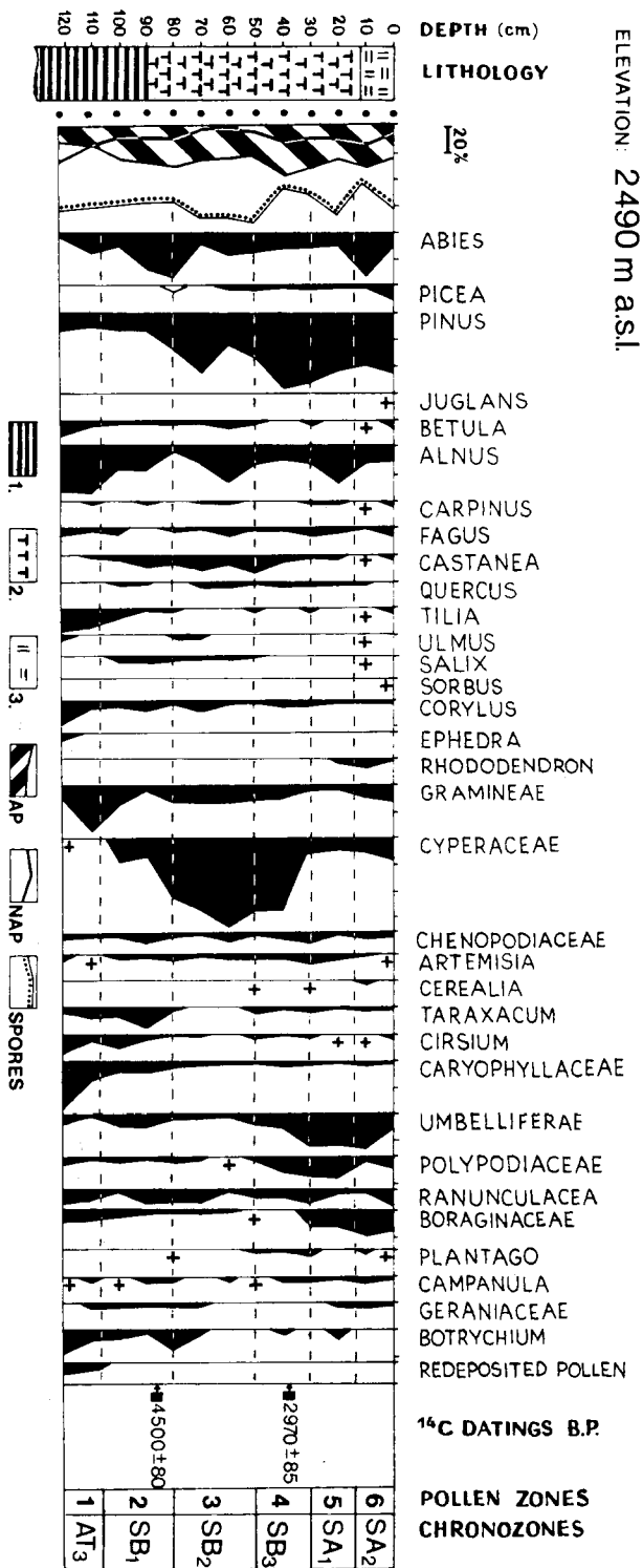
Fig. 2. Spore-pollen diagram of the profile near Bathing Chamouis' lake 1 - clay, 2 - peat, 3 - soil stratum
