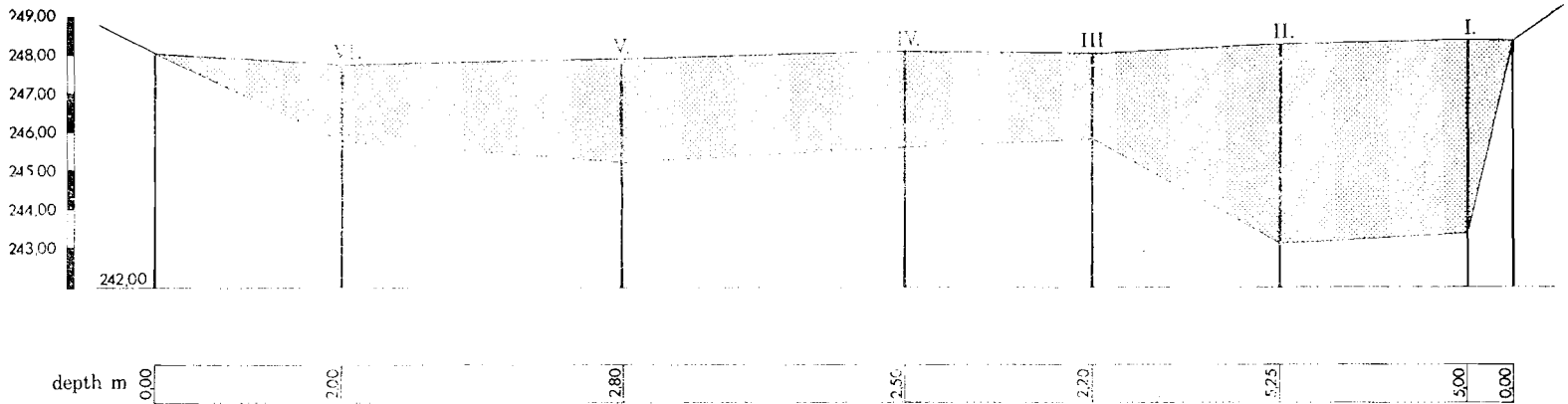
Fig. 3. Slopee mire: NE-SW section
