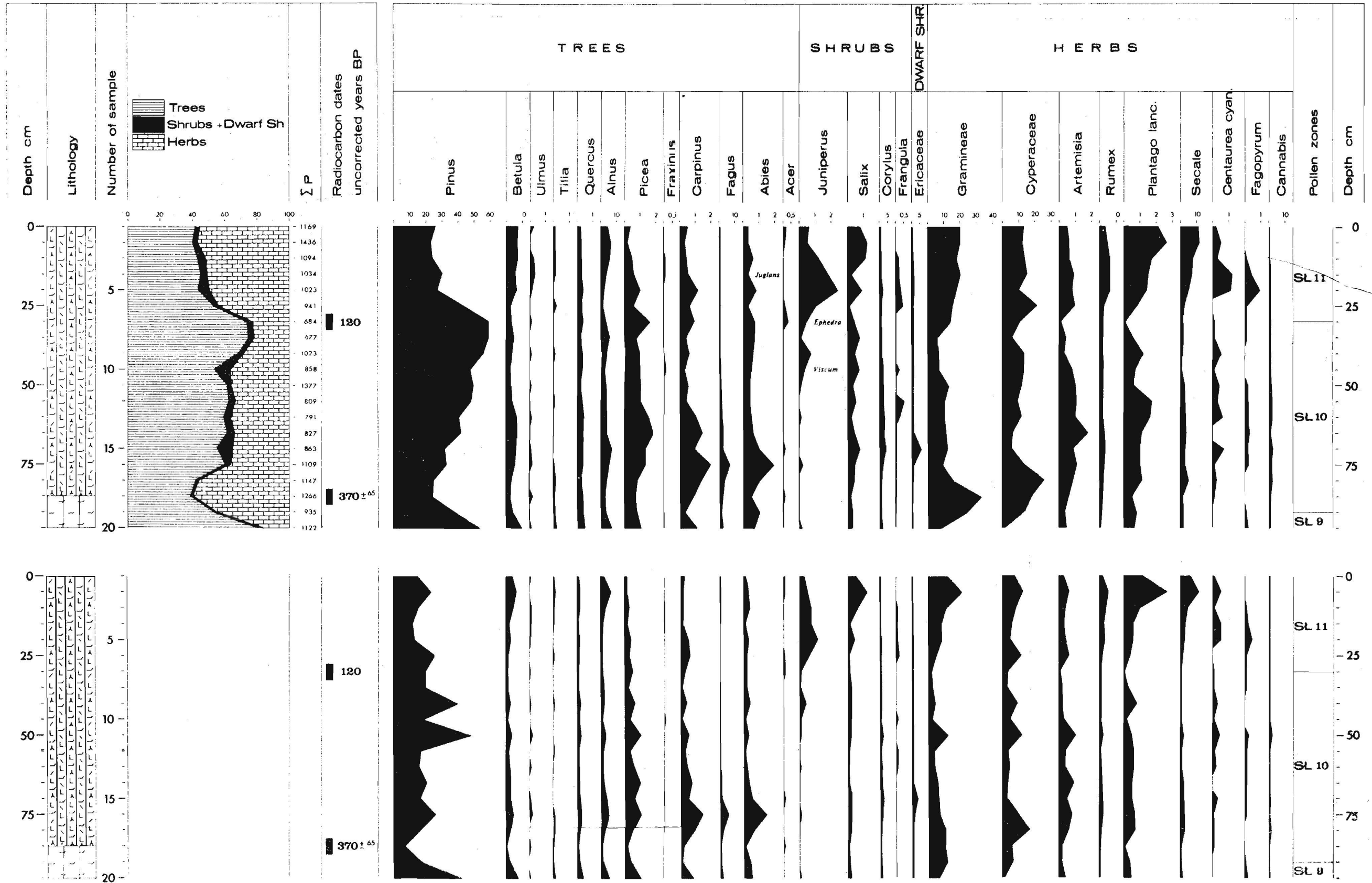
Fig. 6. Percentage pollen diagram (above) of the upper part of Słopiec profile, and pollen concentration diagram (beneath).
