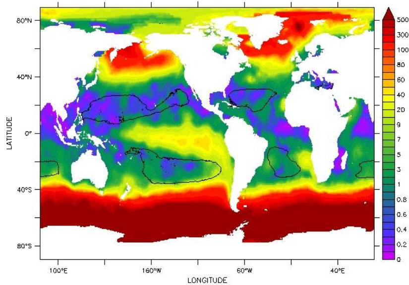
Atmospheric deposition turnover time (years) NO 3
