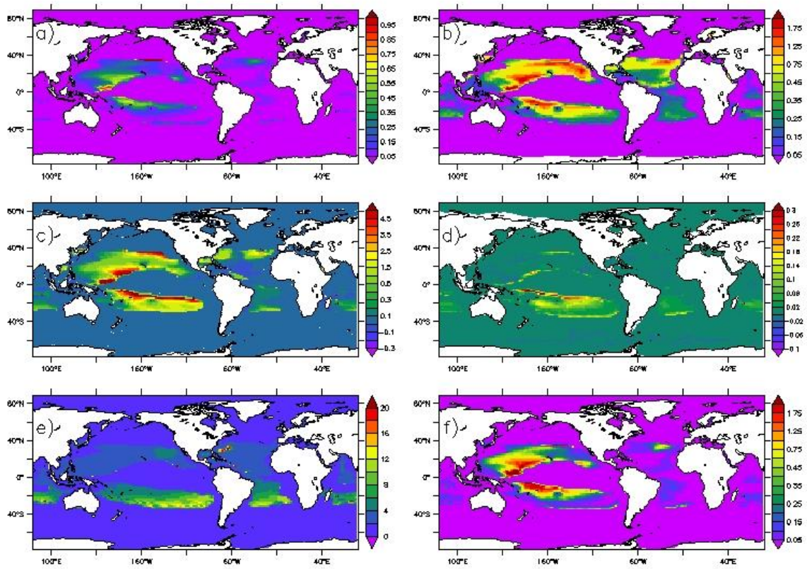
Figure 6. Surface changes (between surface and 100m) induced by the pulse addition applied on the 15th of July (see methods and Table 2). Maximum relative change in a) surface Chl a; b) surface NPP; c) surface Nfix; d) export à 100m; e) Residence time (in days) of the most limiting nutrient. The residence time is defined as the duration of the perturbation of the considered nutrient and f) Maximum relative change in total grazing on phytoplankton.
