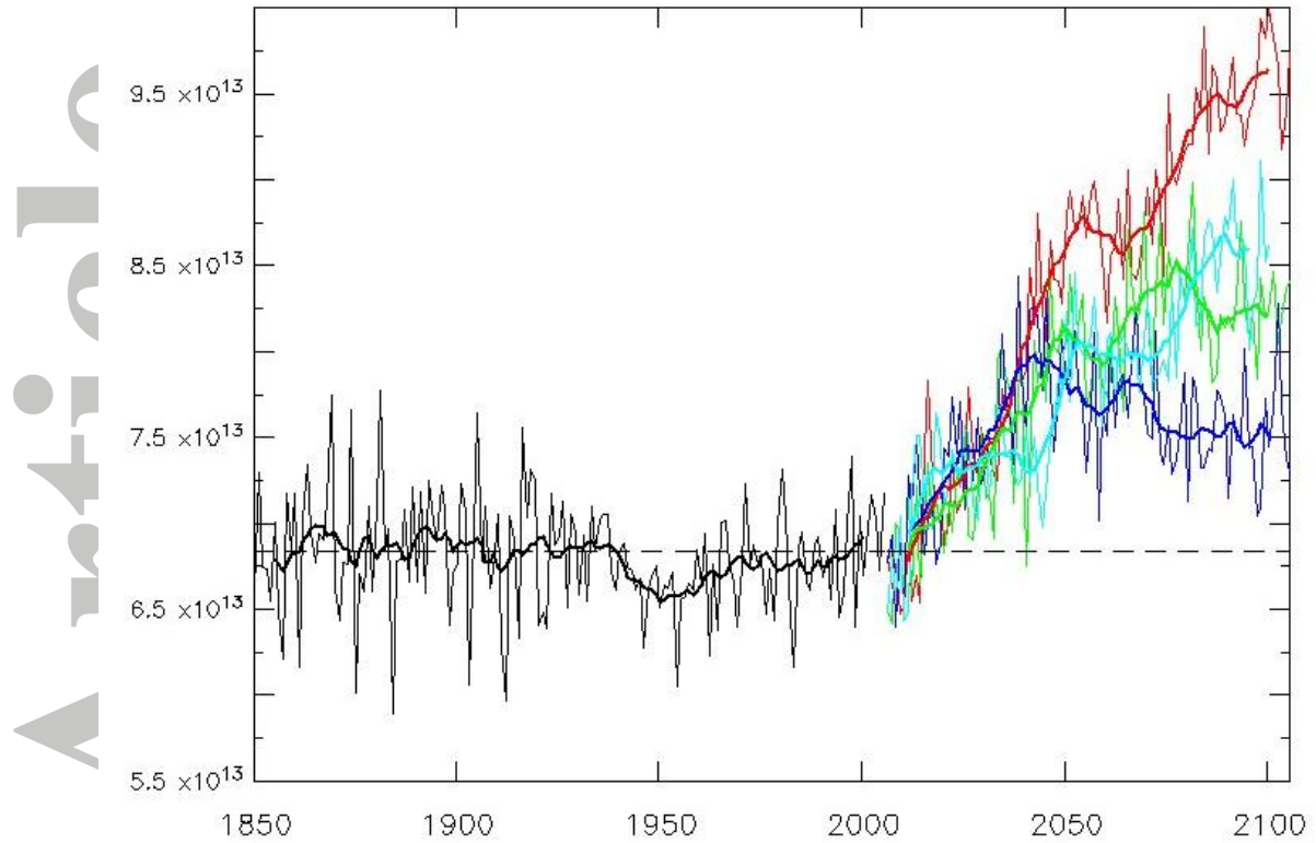
Figure 7. Evolution of the size of oligotrophic areas over 1850-2100, for the historical period (black) and 4 representational concentration pathways (RCPs) scenarios (RCP2.6 blue, RCP4.5 green, RCP6.0 light blue and RCP8.5 red)).
