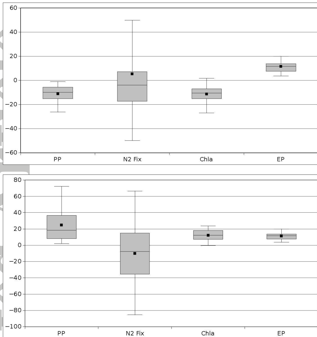
Figure 4. Impact of modification of the mean magnitude of atmospheric deposition on primary production (PP), nitrogen fixation ( N_2 fix), surface chlorophyll- a (Chla) between surface and 100m and export production at 100 m depth (EP), in LNLC regions as computed with the NEMO-PISCES models. Box-Whisker plots (box portion = interquartile range (25 th to 75 th percentile) of the dataset. Horizontal bar within the box = median value. Black square = mean value. Also represented maximum and minimum values) showing relative changes (as percentage) with respect to the standard run using standard climatological atmospheric deposition fields (Fig. 1b) described in the Methods and Table 2. These relative changes are computed from the maximum daily response, simulated over the year, following the change in atmospheric deposition (see Methods) and includes changes in all nutrients together (total set of 4 experiments): when zero deposition are considered (No 'D' experiment; upper panel) and when atmospheric deposition has been multiplied by 5 ('D' experiment; lower panel).
