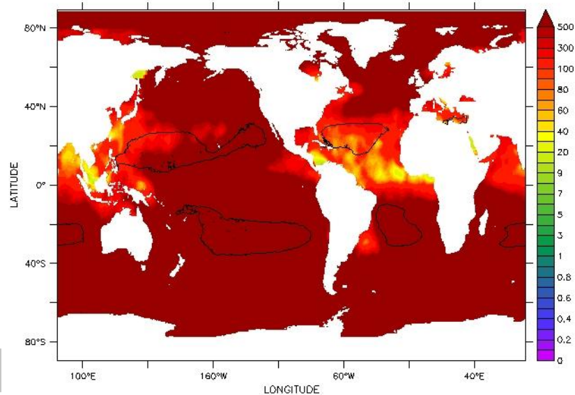
Atmospheric deposition turnover time (years) PO 4
