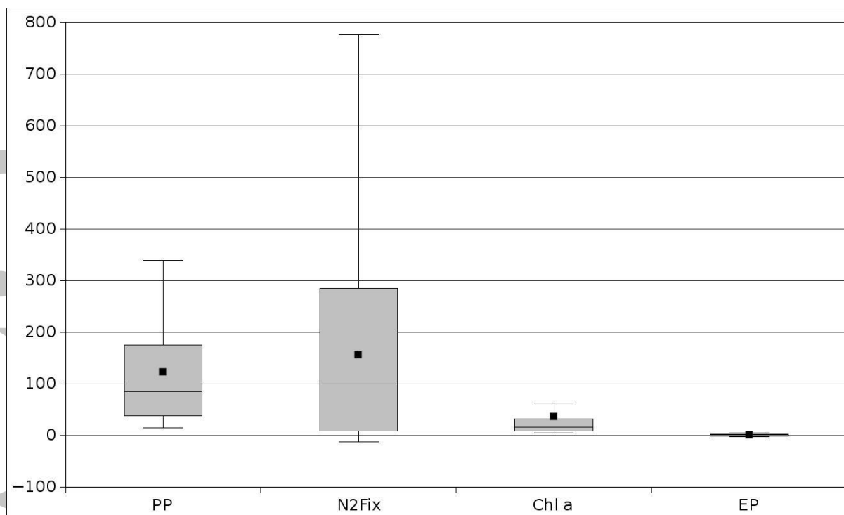
Figure 5. Impact of one pulse of dust and N (on the 15 th of January or on the 15 th of July) superimposed over the standard climatological atmospheric deposition fields, for primary production (PP), nitrogen fixation (N 2 fix), surface chlorophyll a (Chl a) between surface and 100 m and export production at 100 m depth (EP), in LNLC regions computed using the NEMO-PISCES models (Pulse experiments, see Methods and Table 2). Box-Whisker plots (box portion = interquartile range (25 th to 75 th percentile) of the dataset. Horizontal bar within the box = median value. Black square = mean value. Also represented maximum and minimum values) showing the maximum daily relative change averaged over the LNLC regions (as percentage) relative to the Standard run.
