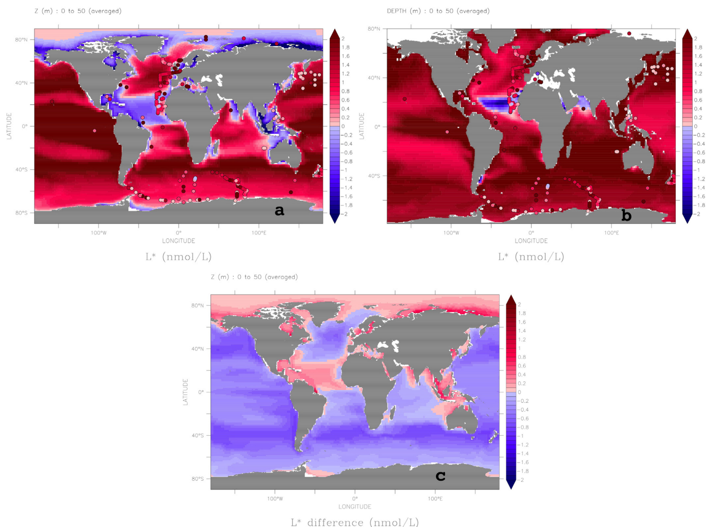
Fig. 8. Ligand excess L^* in the upper 50 m for both standard model runs (panel a: LIGA, panel b, LIGB), together with data-based estimates for this quantity (Boyd and Tagliabue, 2014—in this issue). The lower panel c shows the difference in L^* between an additional model run with changed scavenging (described in this section) and LIGA.
