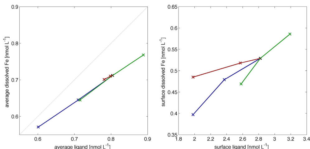
Fig. 7. Changes in globally averaged dissolved iron versus ligand concentrations for the sensitivity runs. Runs differing in r_{L-C} (runs L2C2, L2C1, and LIGB) are connected by a blue line, those differing in p_{col} (runs COL1, L2C2, and COL2) by a green line, and those differing in k_{phot} (runs L2C2, PHOT1, and PHOT2) by a red line. The ‘central’ sensitivity run L2C2 is denoted by a black cross. The left plot shows the average over the whole water depth, the right plot the average over the top 50 m. (For interpretation of the references to color in this figure legend, the reader is referred to the web version of this article.)
