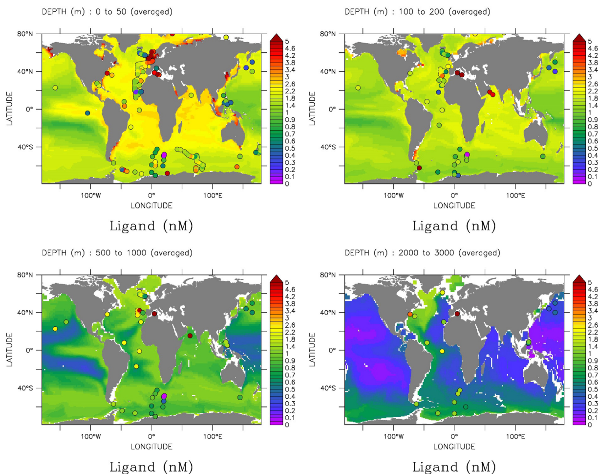
Fig. 2. Ligand distribution after 2000 years in model run LIGB. Symbols in the same color coding show our compilation of in situ-measurements. (For interpretation of the references to color in this figure legend, the reader is referred to the web version of this article.)
