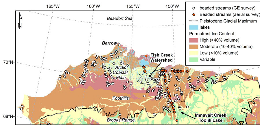
Figure 2. The distribution of beaded streams located using Google Earth and from aerial surveys across the North Slope of Alaska in relation to permafrost ice content (Jorgenson et al., 2008) and the Pleistocene glacial maximum (Manley and Kaufman, 2002). The locations of the Fish Creek watershed (focus area of this study) and Innavait Creek (focus area of the majority of previous work on beaded streams) are indicated.
