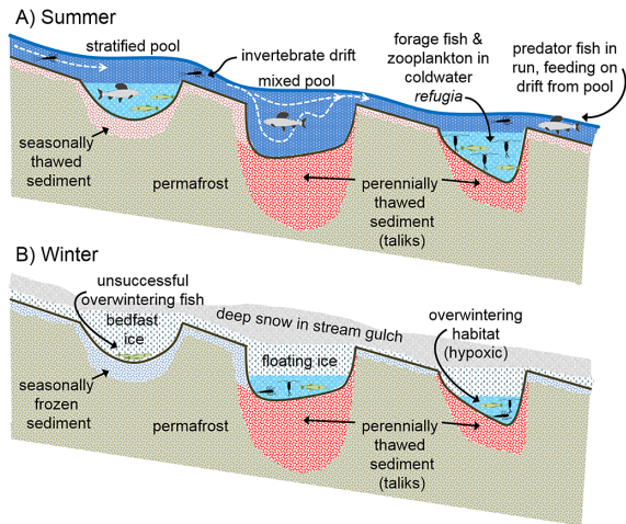
Figure 15. Conceptual diagram showing morphology, physical regimes, habitats, and organisms of a hypothetical pool-run system in the summer (a) and winter (b) based on observations and monitoring studies in multiple beaded stream systems during these time periods over many years.
