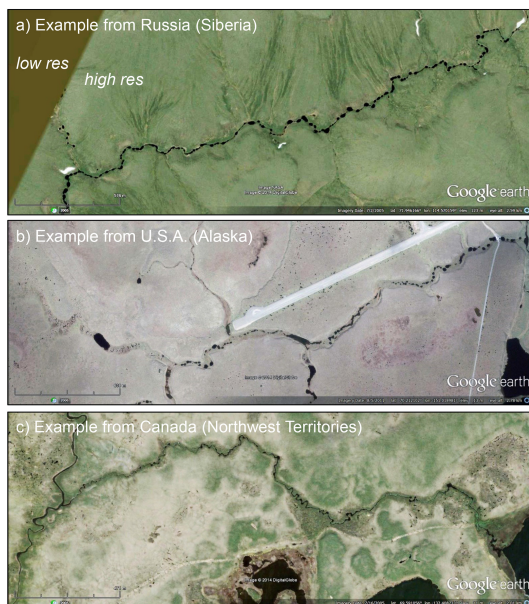
Figure 1. Examples of beaded stream networks located by scanning high-resolution (<5 m) imagery available in Google Earth in (a) Russia (Anabar River watershed), (b) USA (near Nuiqsut, Alaska), and (c) Canada (Tuktoyaktuk Peninsula).
