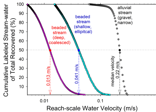
Figure 14. Examples of reach-scale water velocity distributions (reach length/travel time) measured using hydrologic tracer tests (rhodamine WT pulse additions) shown as cumulative tracer recovered downstream. Results from two beaded streams, Crea Creek (blue squares) and Blackfish Creek (red triangles) are compared to an alluvial stream (black circles) in a mountain meadow (Arp unpublished data, stream described in Arp et al., 2007); all three streams had similar discharges ranging from 85 to 140 L s -1 during tracer tests and slopes ranging from 0.1 to 0.2 %, but with otherwise differing morphologies (experimental data and inverse modeling results shown in Table 3).
