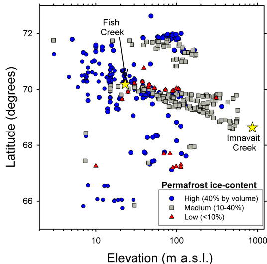
Figure 5. The distribution of beaded stream channels throughout the circum-Arctic in relation to latitude, elevation, and permafrost ground-ice content. Stream networks were identified using imagery in Google Earth in the zone of continuous permafrost where high-resolution imagery was available. The location of streams in the Fish Creek (focus area for this study) and Imnavait Creek (focus area for majority of previous beaded stream research) watersheds are indicated with yellow stars.
