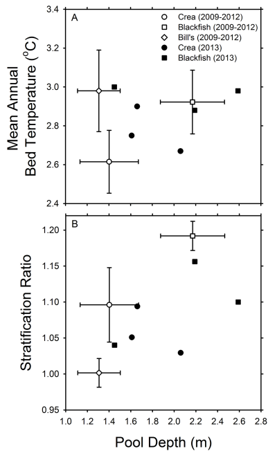
Figure 12. Thermal regime characteristics of single pools at three beaded streams averaged over 4 a (error bars are standard deviations). In 2013, three additional pools within two of these beaded streams were monitored to assess within-stream variability of thermal characteristics. Thermal regimes were characterized by mean annual temperatures at pool beds (a) and stratification ratios as the average ratio between the pool surface and bed during the period from July to mid-August in each year (b). Pool depths are averaged during the same period that temperature was summarized in each plot.
