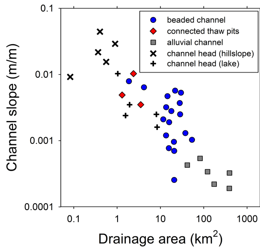
Figure 7. The organization of the major channel forms and channel initiation points (heads) in the Fish Creek watershed are shown in relation to drainage area and channel slope (measured from a 5 m DEM).
