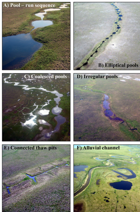
Figure 4. Oblique photographs showing typical pool-run morphology (a) and examples of beaded channel forms (b–e) compared to alluvial channel (f) morphology.
