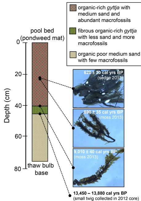
Figure 10. Diagram of generalized sediment core stratigraphy from a large pool in Crea Creek (indicated in Fig. 9) collected in both 2012 and 2013 showing the location of macrofossil fragments collected for radiocarbon dating. The sharp transition from organic-rich gyttja to medium sand is interpreted to be the base of the pool at its time of formation.
