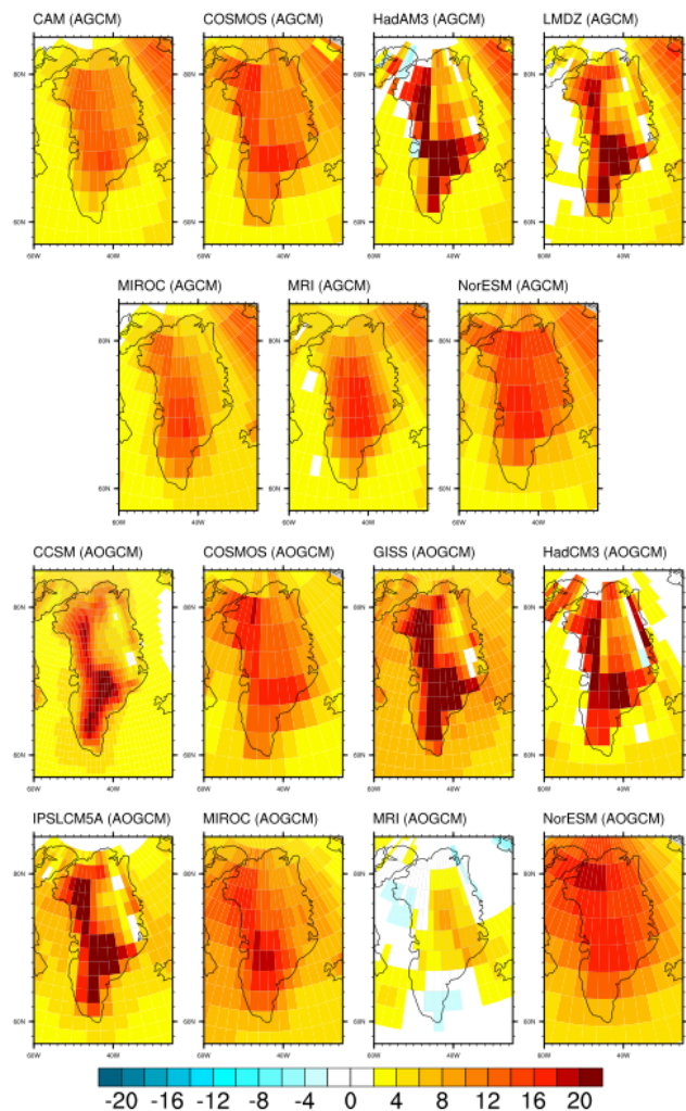
Figure 4. mPWP minus pre-industrial mean July surface air temperature ( ^\circ\text{C} ) over Greenland for the PlioMIP ensemble using atmosphere-only (AGCMs) and coupled atmosphere–ocean climate models (AOGCMs). Temperature plotted on the original climate model resolution.
