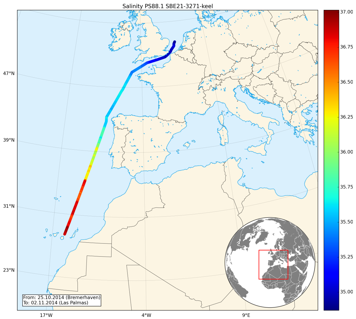
Figure 5: Salinity map of TS Keel
