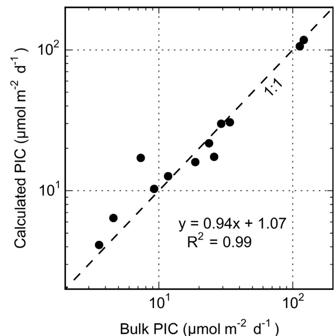
Fig. 4. Relationship between the measured bulk PIC flux and the calculated PIC flux (sum of the foraminifer, the 20–63 \mu\text{m} and the <20 \mu\text{m} fine fractions PIC fluxes). Dashed line denotes the 1:1 relationship. The equation of the regression performed on the raw data is given.
