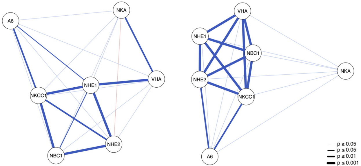
Fig. 6. Correlation networks of ion transporter protein expression. Correlation networks of ion transporter protein expression in gills of Atlantic cod ( G. morhua ) acclimated to 550 \mu\text{atm} , 1200 \mu\text{atm} and 2200 \mu\text{atm} \text{CO}_2 and 10 °C (A) or 18 °C (B), respectively. Spearman correlation analysis was performed and the corresponding matrices were used as input for correlation networks. Edge width was scaled according to respective significance levels (0.05, 0.01 and 0.001). Color saturation was cut at p \geq 0.05 . For corresponding Spearman correlation coefficients, see supplementary material.
