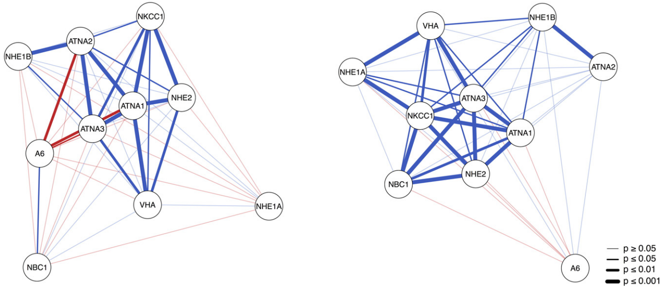
Fig. 4. Correlation networks of ion transporter mRNA expression. Correlation networks of ion transporter mRNA expression in gills of Atlantic cod ( G. morhua ) acclimated to 550 \mu\text{atm} , 1200 \mu\text{atm} and 2200 \mu\text{atm} \text{CO}_2 and 10 °C (A) or 18 °C (B), respectively. Spearman correlation analysis was performed and the corresponding matrices were used as input for correlation networks. Edge width was scaled according to respective significance levels (0.05, 0.01 and 0.001). Color saturation was cut at p \geq 0.05 . For corresponding Spearman correlation coefficients, see supplementary material.
