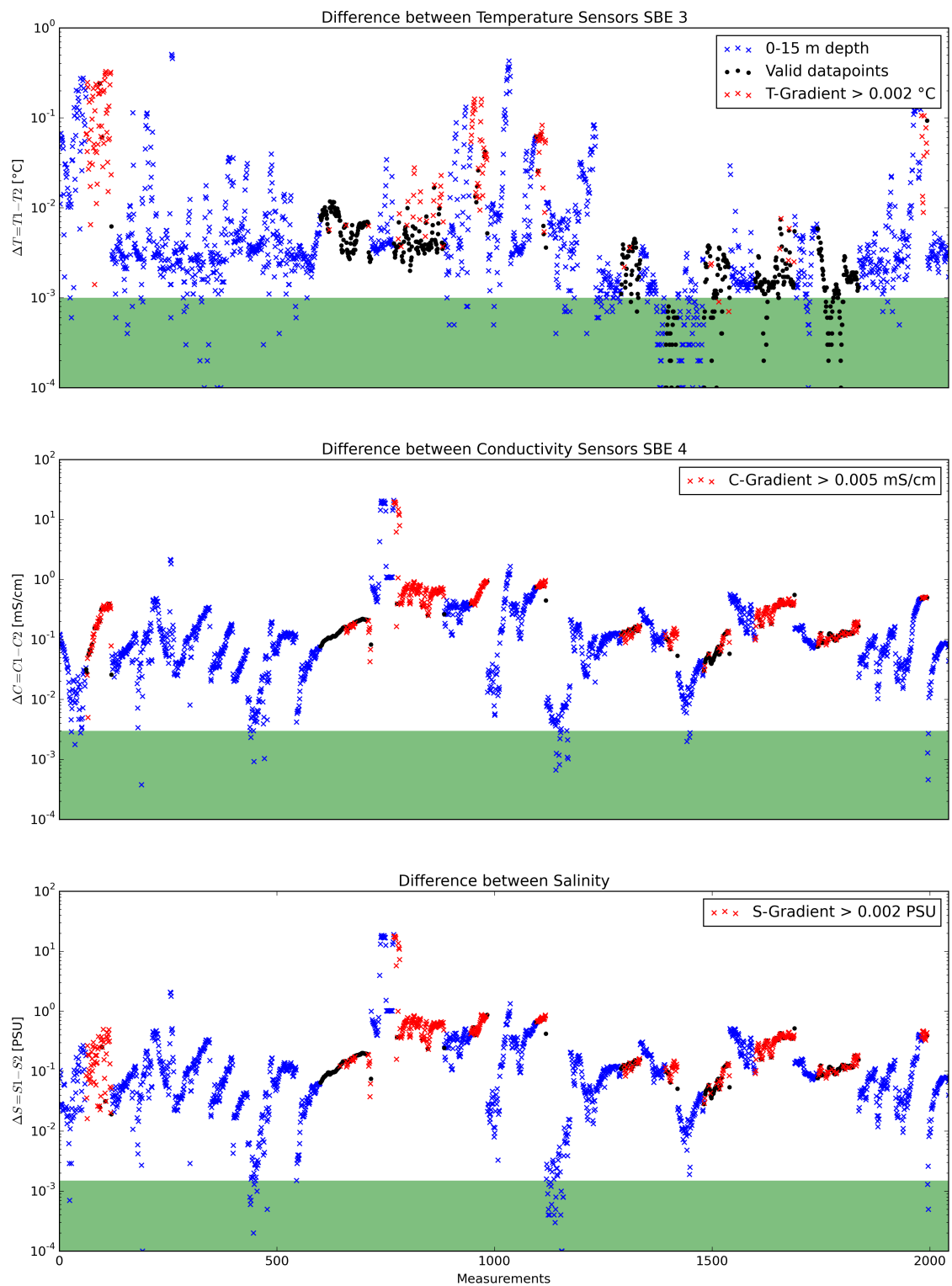
Figure 2: Data accuracy of sensor pairs HE454
