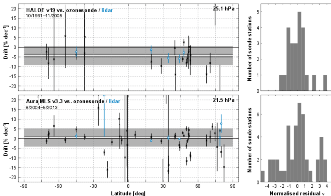
Figure 3. (Left) Drift \hat{\alpha}_j and one sigma uncertainty \hat{\sigma}_{\alpha,j} of HALOE (top) and Aura MLS (bottom) around 25 km relative to co-located observations at each station in the NDACC/GAW/SHADOZ ozonesonde (black) and NDACC lidar (blue) networks. Also shown are the weighted mean for the ozonesonde network \bar{\alpha} (horizontal white line), its adjusted uncertainty \sigma_{\bar{\alpha}}^* (dark grey area) and the standard deviation of the ensemble of single sonde site drift estimates (light grey area). (Right) Corresponding distribution of normalised residuals \nu from the ozonesonde network.
