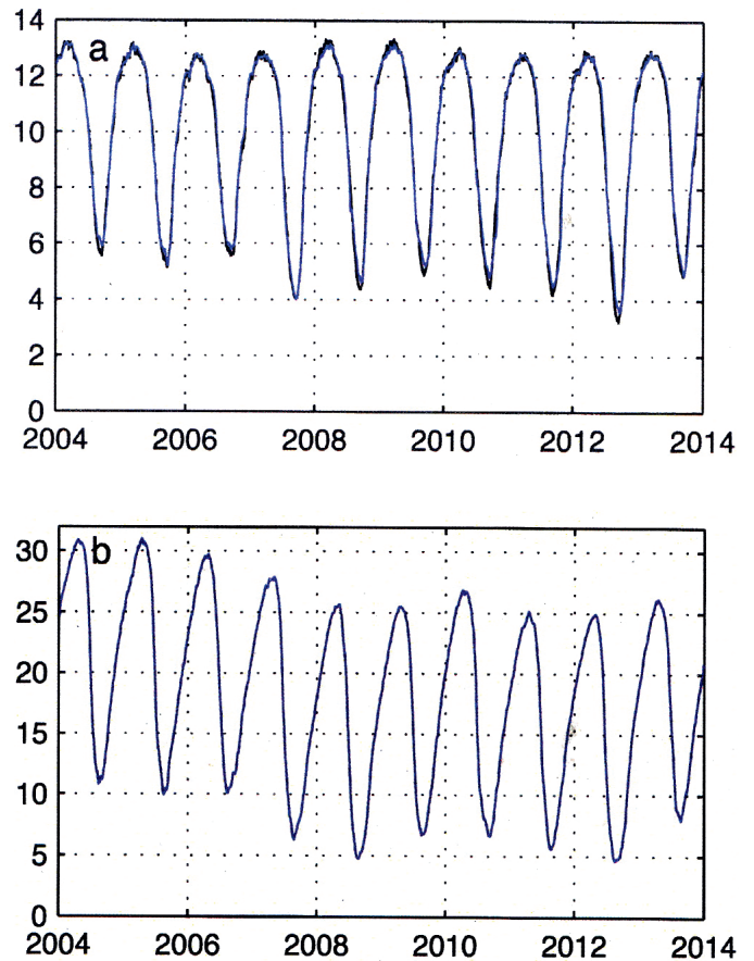
Fig. 2: a): Modelled (blue) and observed (CAVALIERI et al. 1996, black) sea-ice extent (15 % concentration limit) of the entire model domain, daily averages 2004–2013 (million km 2 ); b): Modelled total sea ice volume, daily average 2004–2013 (thousand km 3 ).
