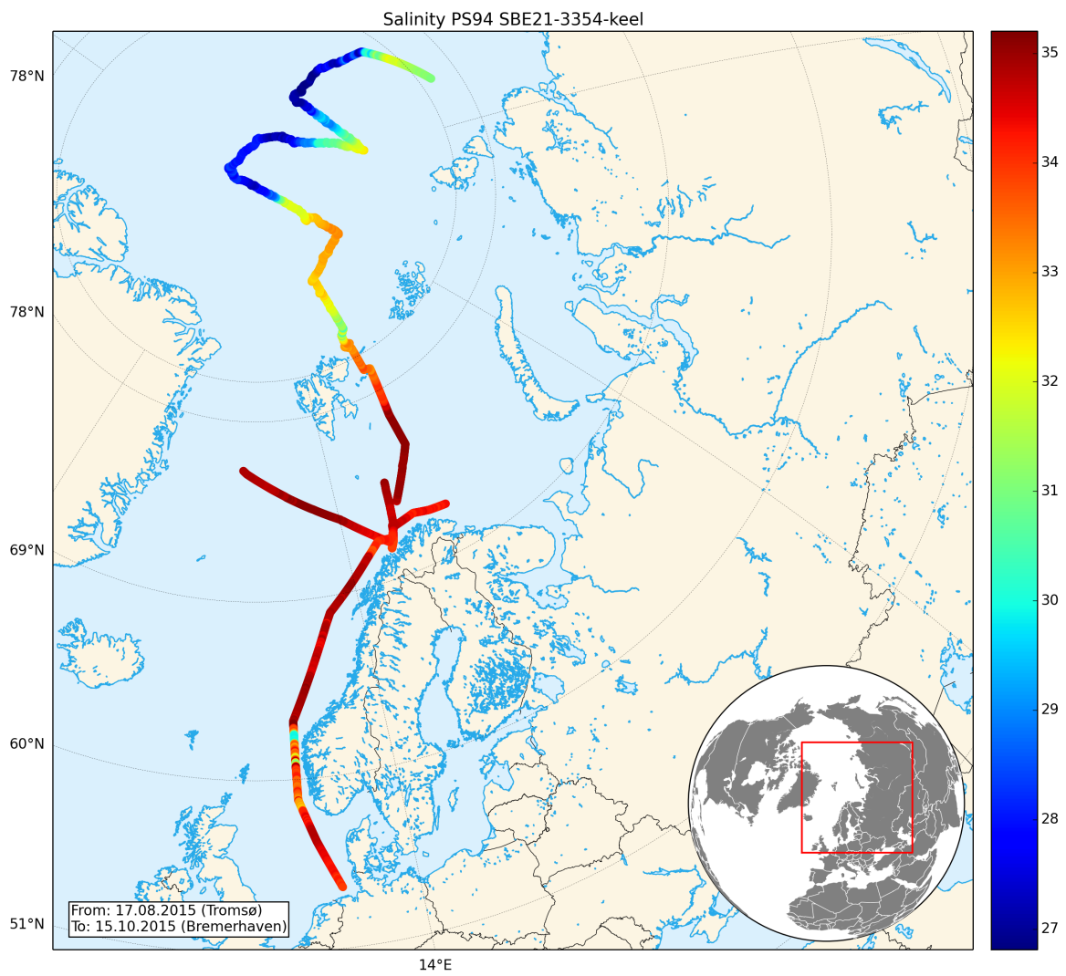
Figure 5: Salinity map of TS Keel
