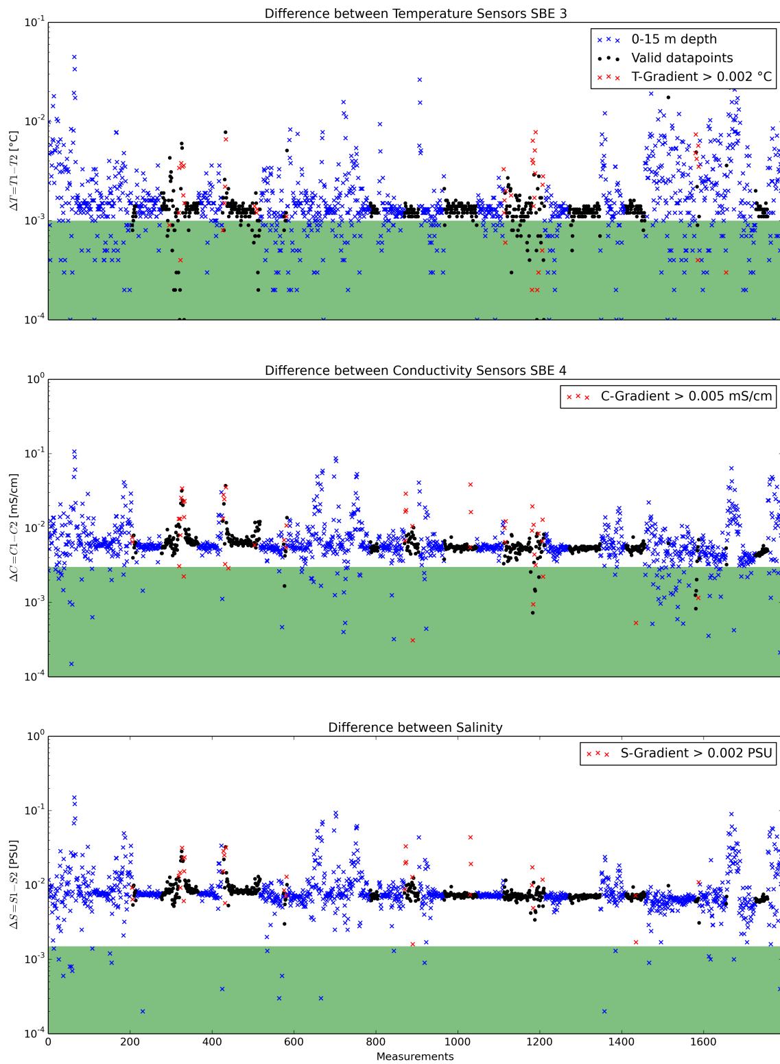
Figure 2: Data accuracy of sensor pairs HE418
