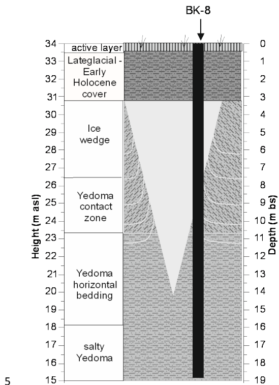
Figure 7. Scheme of the BK-8 permafrost core including the main cryolithological units. The legend is given in Figs. 4 and 6.
