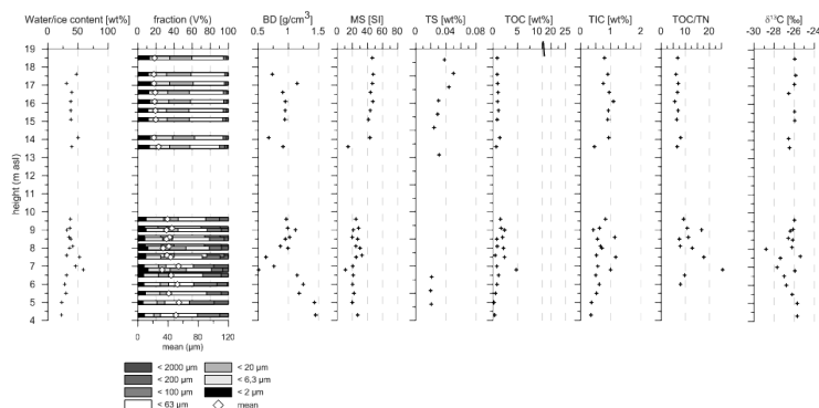
Figure 6. Cryolithological and organic matter properties of the Buo-04 profile (note that due to overlapping sub-profiles, different values may be displayed at similar heights)
