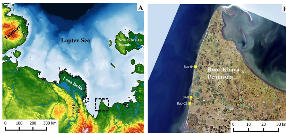
Figure 1. Study region in the central Laptev Sea (A, based on IBCAO 3.0 Jakobsson et al. 2012) including Buor Khaya Peninsula marked by the black frame and Yedoma IC reference sites on Bol'shoy Lyakhovsky Island (1) and Bykovsky Peninsula (2); and position of the study sites Buo-02, Buo-04, and BK-8 at the western coast of the Buor Khaya Peninsula (B, LANDSAT_8 image from 2015).
