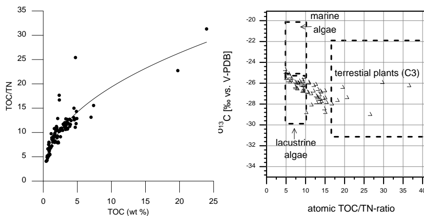
Figure 16. Organic matter characteristics of the Buor Khaya Yedoma. Left: Correlation of the TOC content and the TOC/TN ratio. Right: Distribution of the TOC – \delta^{13}\text{C}_{\text{TOC}} relationships according to Meyers (1997).
