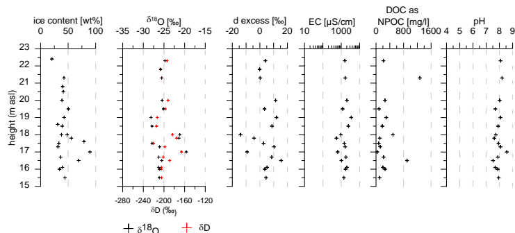
5 Figure 9. Measurements of ice content, isotope ratios, electrical conductivity (EC), pH, and solutes over height in m asl for samples from the Buo-02 exposure.
