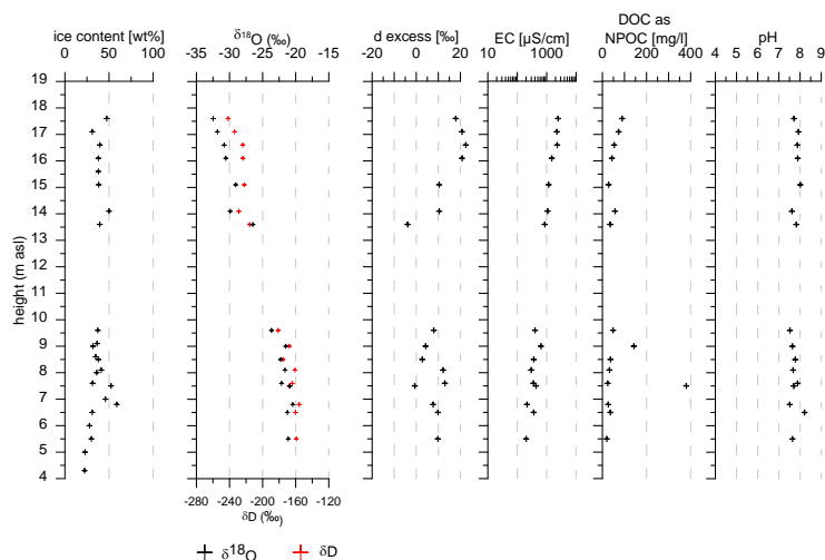
Figure 10. Measurements of ice content, isotope ratios, electrical conductivity (EC), pH, and solutes over height
