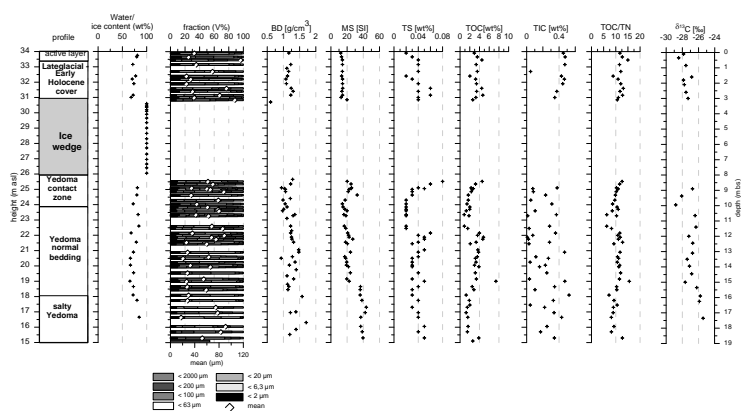
Figure 8. Cryolithological and organic matter properties of the BK-8 Yedoma IC core.
