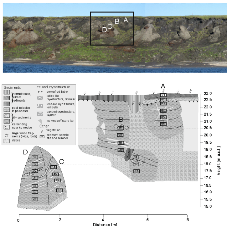
Figure 3. Overview photo and scheme of the Bu0-02 Yedoma IC exposure with sample positions and main cryolithological features (modified from Strauss and Schirmeister, 2011).
