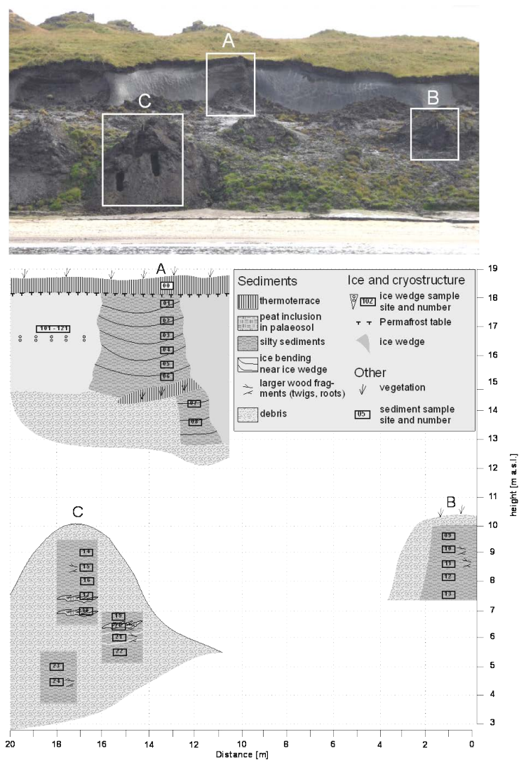
Figure 5. Overview photo and scheme of the Buo-04 Yedoma IC exposure with sample positions and main cryolithological features (modified from Strauss and Schirrneister, 2011).
