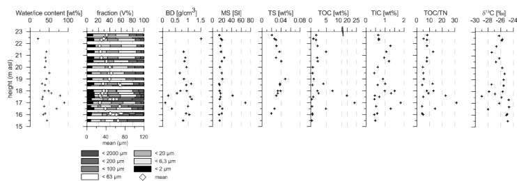
Figure 4. Cryolithological and organic matter properties of the Bu0-02 profile (note that due to overlapping sub-profiles, different values may be displayed at similar heights).
