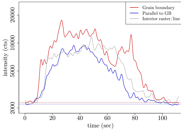
Fig. 5.7: Exemplary laser ablation data of three locations in one grain for sodium (run 48, small-grain layer, grain 5). The calculated background level for each measurement is indicated (dashed lines); the values vary slightly in this example. The GB is clearly enriched in sodium, while the grain interior is depleted; this pattern holds true for the majority of the collected sodium data.
