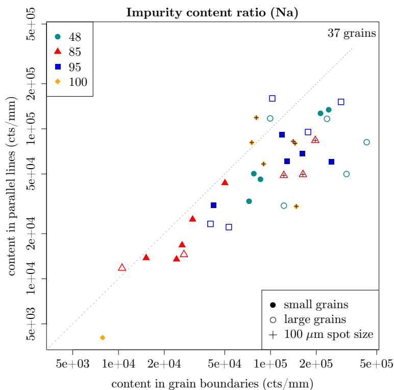
Fig. 5.10: The sodium content in grain boundaries is scattered against the content in the associated parallel lines, illustrating their ratio. Each symbol represents a pair. Filled symbols represent small and open symbols large grains, different symbols indicate the four depths with colors for visual support, the larger spot size is indicated by black crosses, both axes are logarithmic, the dashed line indicates the 1:1 ratio.
