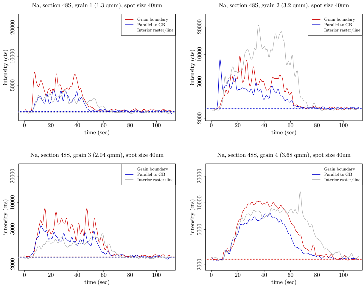
Fig. C.1: Small-grain section 48S: Grain boundaries show mostly higher sodium content than grain interiors. Grain 2 is an exception/outlier to that observation, grain 4 is not clear either – both grains are larger than the others. Grain 5 is shown in Fig. 5.7, p. 77.
