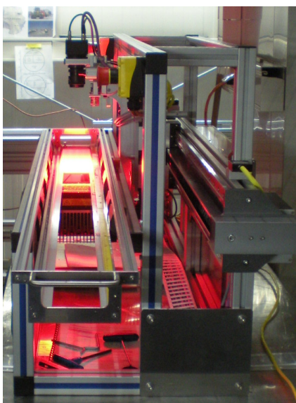
Fig. 3.10: Photo of line scan instrument at AWI. The ice slab is placed in a tray and illuminated from below while the camera records from above.
