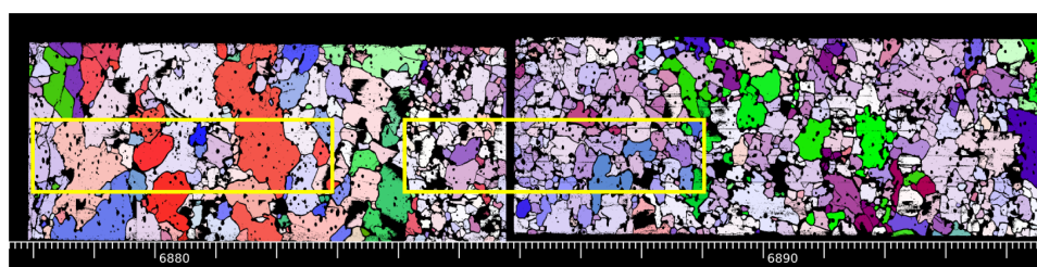
Fig. 3.16: Fabric grain images of run 95 with depth scale in cm. The yellow boxes illustrate the position of the ablation chamber seal on the ice surface which is actually perpendicular to the here displayed fabric surface.
