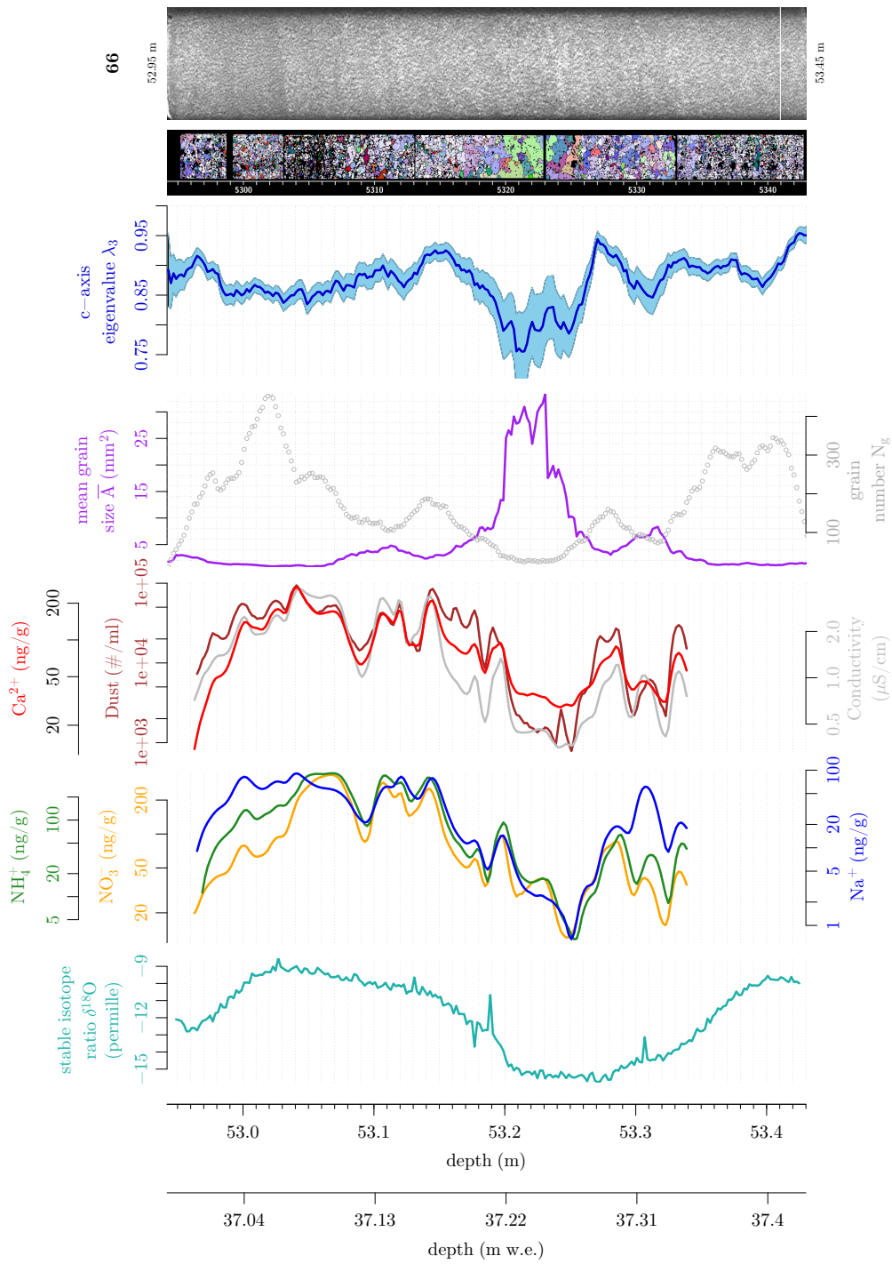
Fig. B.21: Fabric and microstructure parameters in cm-resolution in comparison with CFA data for KCC range 66.
