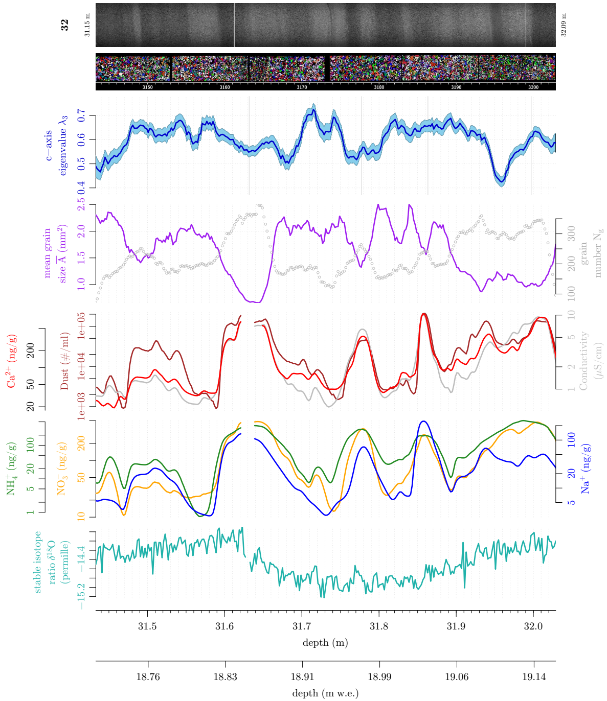
Fig. 5.1: Fabric and microstructure parameters in cm-resolution in comparison with CFA data for KCC range 32. Calcium ( \text{Ca}^{2+} , red), sodium ( \text{Na}^+ , blue), ammonium ( \text{NH}_4^+ , green) and nitrate ( \text{NO}_3^- , orange), the conductivity of the melt water (gray), the particulate dust content (brown) and the stable oxygen isotope ratio \delta^{18}\text{O} (in ‰, turquoise) are shown. Vertical grey solid lines indicate annual-layers as picked from CFA data.
