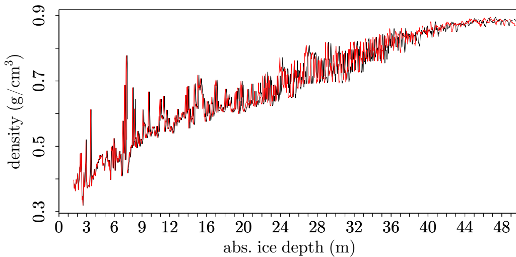
Fig. B.6: Illustration of the depth scale correction for X2D density. Smoothed (with a bandwidth of 0.05 m) high resolution density for the upper 50 m of the KCC ice core with old (black) and corrected (red) depth scale. The cumulative shift at the bedrock amounts to 55 cm.
