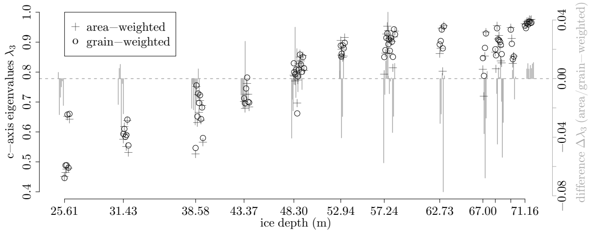
Fig. 4.4: Comparison of KCC c -axis eigenvalues for area- and grain-weighted computation. The difference \Delta\lambda_3 is illustrated in grey bars and is mostly restricted to \pm 0.04 with some larger differences in the lower part of the core.
