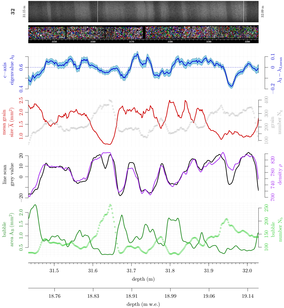
Fig. B.9: Fabric and microstructure in cm-resolution for KCC run 32. Line scan grey value and density showed a systematic offset of 2 cm for the line scan values, based on the comparison with the mean grain size, which can be a likely result from erroneous depth assignment. This offset was corrected for plotting and correlation computation. Line scan and eigenvalue record exhibit some common features.
