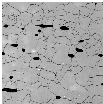
(h) Angular grains in inclined small grain section in 62.93 m depth, sample 85-22.
