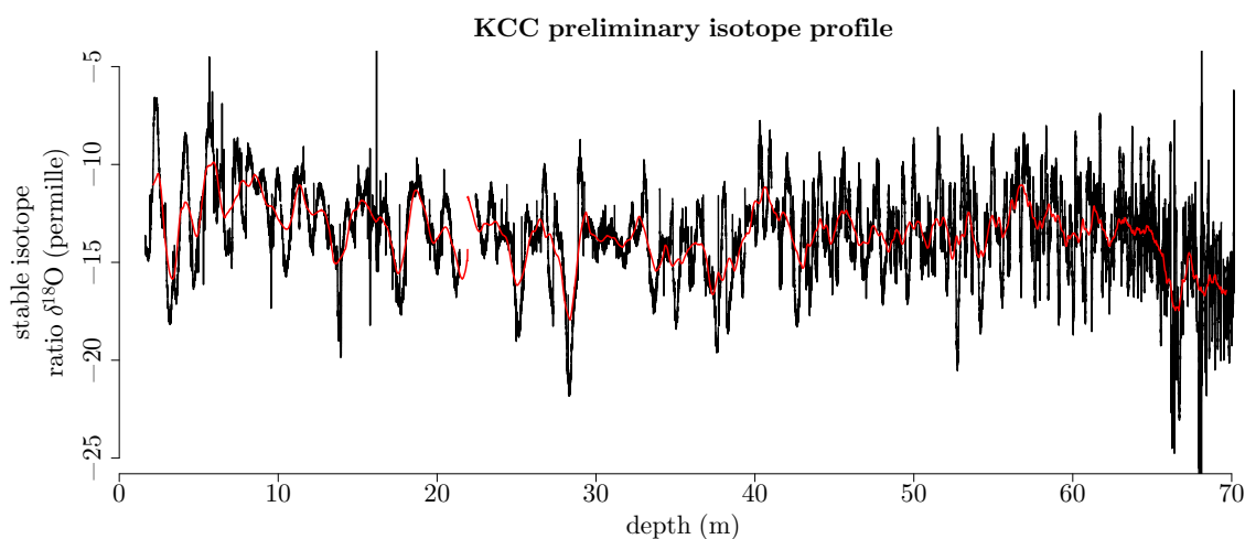
Fig. B.5: Stable oxygen isotope ratio \delta^{18}\text{O} (‰) of KCC ice core as measured online during CFA (pers. comm. H. Fischer/G. van der Wel, University of Bern, 2014).
