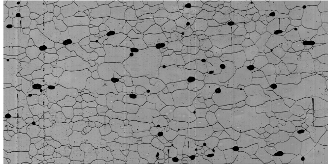
Fig. 4.13: LASM image detail (2 cm 2 ) from 71.26 m depth, sample 100-31, illustrating small grain distribution in basal section.
