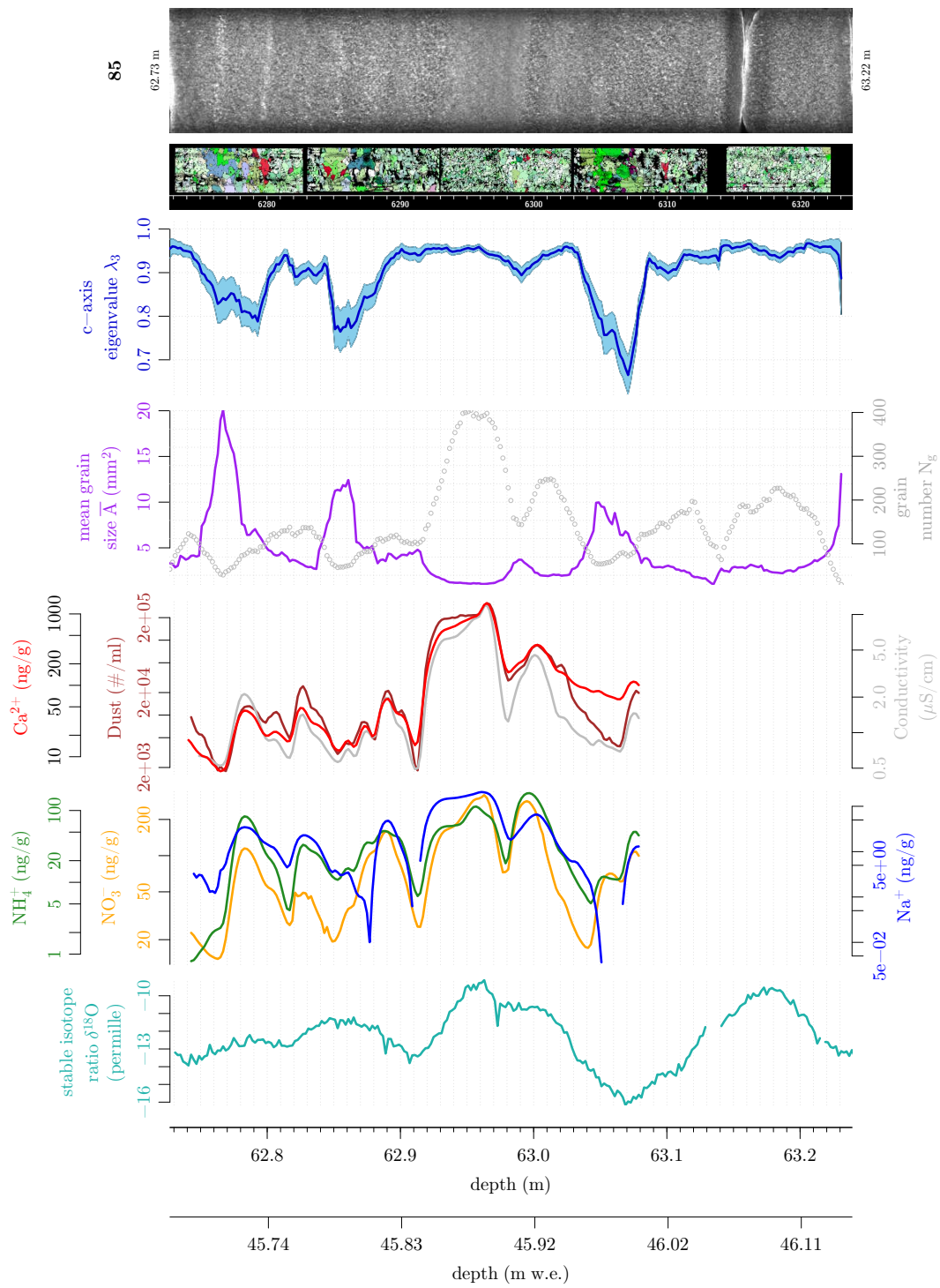
Fig. B.22: Fabric and microstructure parameters in cm-resolution in comparison with CFA data for KCC range 85.
