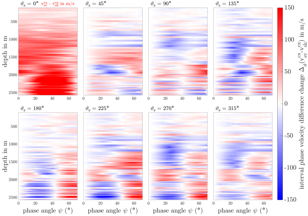
Fig. 6.9: Top left: Difference of EDML seismic velocities between SH- and SV-wave as calculated with c-axes framework for incidence angles up to 70^\circ . The other seven panels give the change of the S-wave difference for different seismic plane azimuth angles \vartheta_s .
