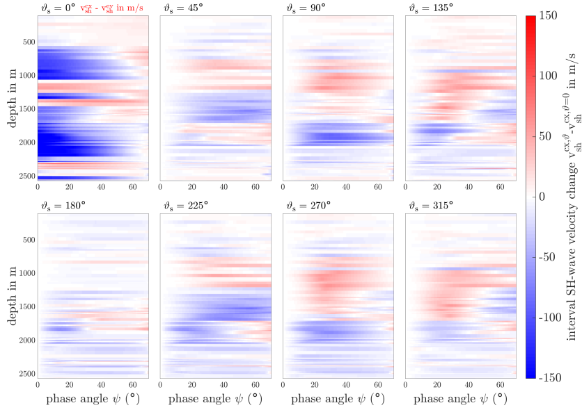
Fig. D.5: Top left: Difference in EDML seismic SH-wave interval velocity between c-axes and eigenvalue method. For \vartheta_s > 0^\circ the change in difference is shown as compared to \vartheta_s = 0^\circ .
