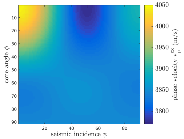
Fig. 6.3: P-wave velocity v_p^{cx} for cone fabric from random c-axes using the c-axes framework.
