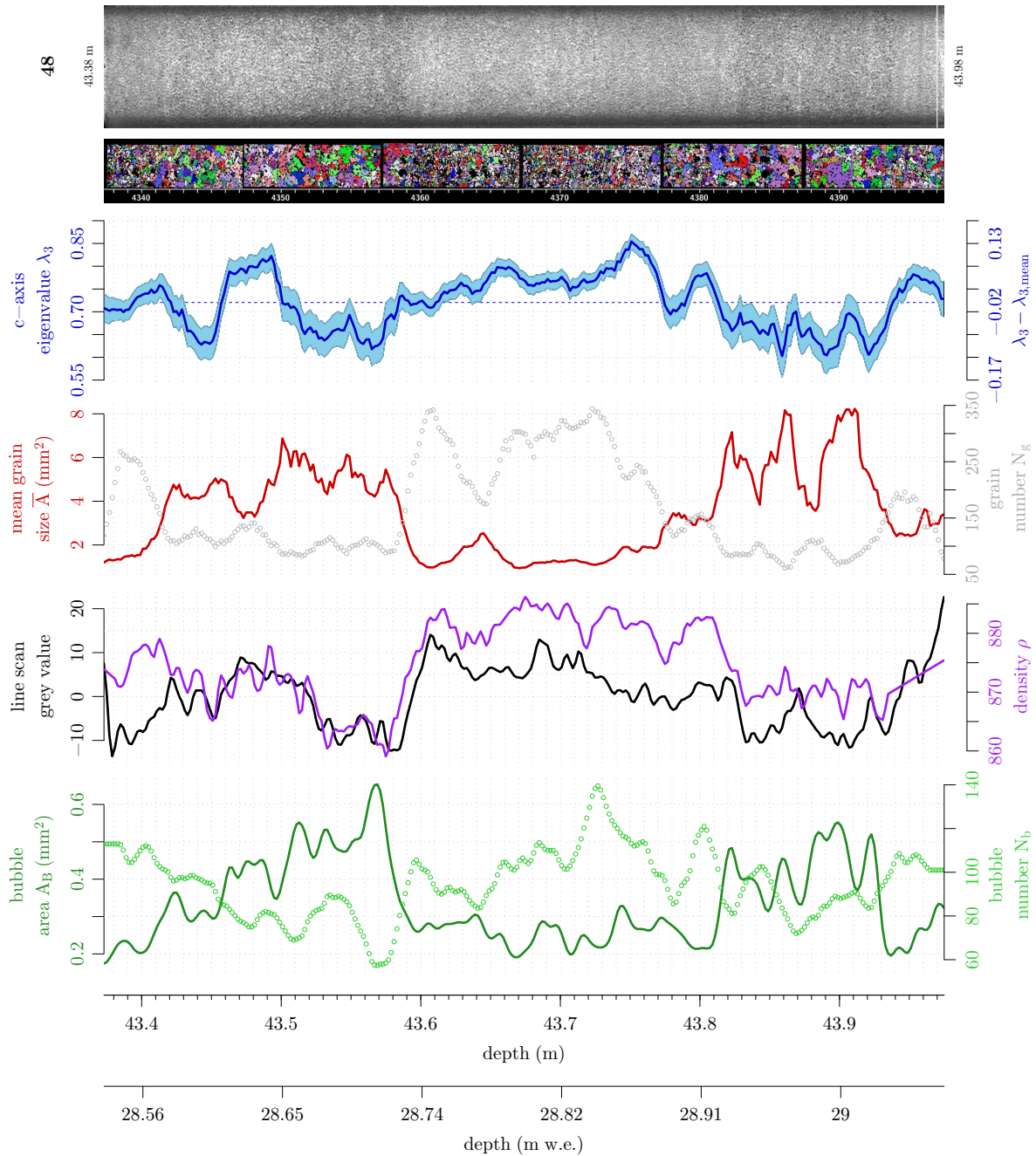
Fig. 4.21: Fabric and microstructure parameters in cm-resolution for KCC run 48. At the top the line scan image is shown (ice top to the left, white lines indicate the beginning and/or end of the section which corresponds to the parameter records), followed by the grain images produced with cAxes showing the identified grains and their orientation (colorcode described in Fig. 3.11). The panels show the parameters as calculated for moving frames of 2 cm width in 2 mm steps (c-axis eigenvalue \lambda_3 with uncertainty range (eq. (2.5)), mean grain size \bar{A} , bubble and grain number) or kernel smoothed with a bandwidth of 5 mm (line scan grey value, high-resolution density \rho , bubble area A_B ). The mean c-axis eigenvalue is indicated with the dashed blue line. Depth is additionally provided in metre of water equivalent (m w.e.).
