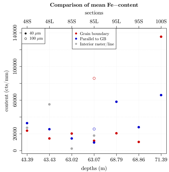
Fig. 5.9: Summary of the mean iron content from all grains of each section for different locations.
