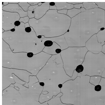
(e) Protruding and island grains and bubble alignment in 49 m depth, sample 58-11.
