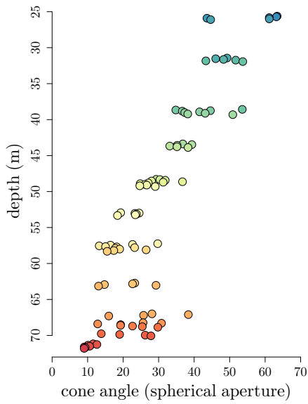
Fig. 4.7: Cone angle (spherical aperture) as calculated for KCC thin section fabric. Color as in Fig. 4.6.
