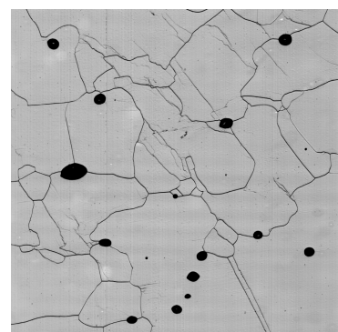
(i) Parallel GBs at high inclination in 67.1 m depth, sample 92a-21.
