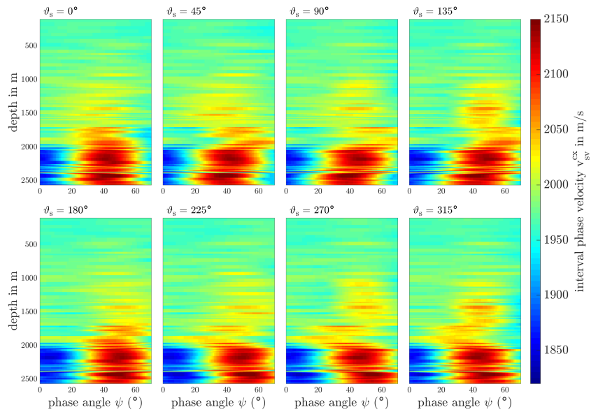
Fig. D.4: Seismic SV-wave interval velocity for c-axes method (EDML).
