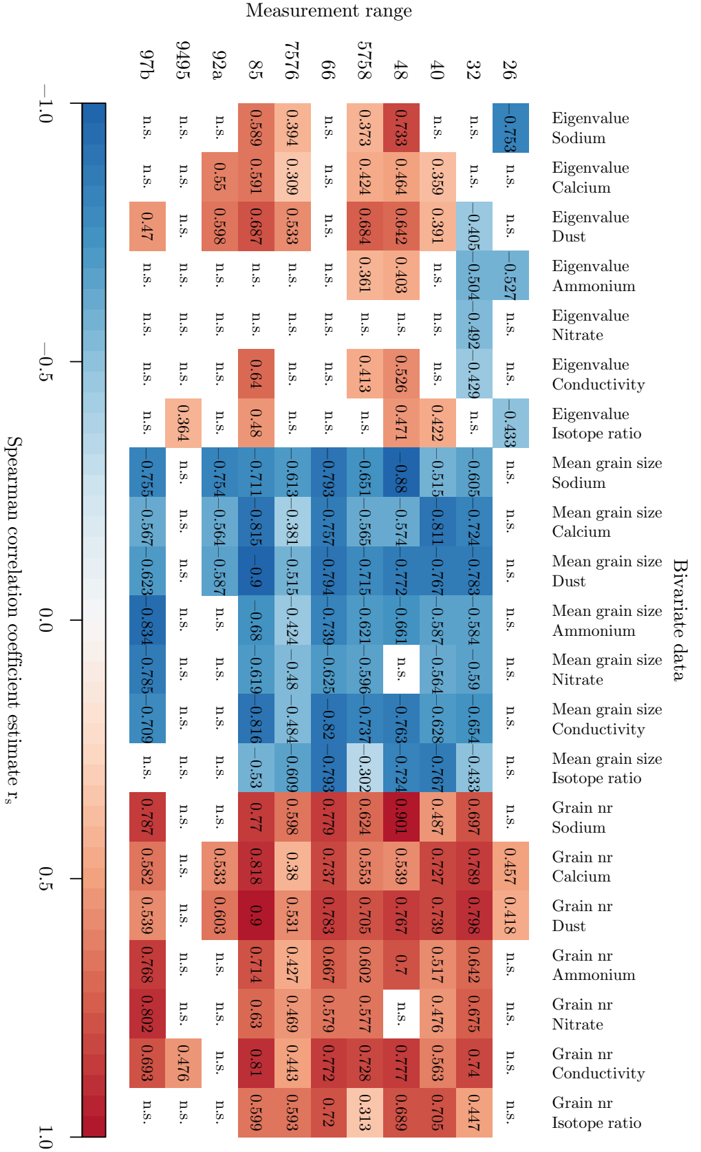
Fig. 5.4: Spearman's rank correlation coefficient r_s for c-axis eigenvalue, mean grain size and grain number with impurities from CFA and stable oxygen isotope ratio for 11 measurement ranges (no CFA data available for bottom range). Values represent the median of the correlation coefficients from all possible subsets of the bivariate data with a sample interval of 2 cm. The sample size lies between 13 and 53 pairs per calculation, depending on the length of the range and the occurrence of missing intervals in the CFA data. Non-significant (n.s.) values are excluded, i.e. if the p-value > 0.05 (section 3.4.6, p. 30). Blue shades indicate negative, red shades positive correlation.
