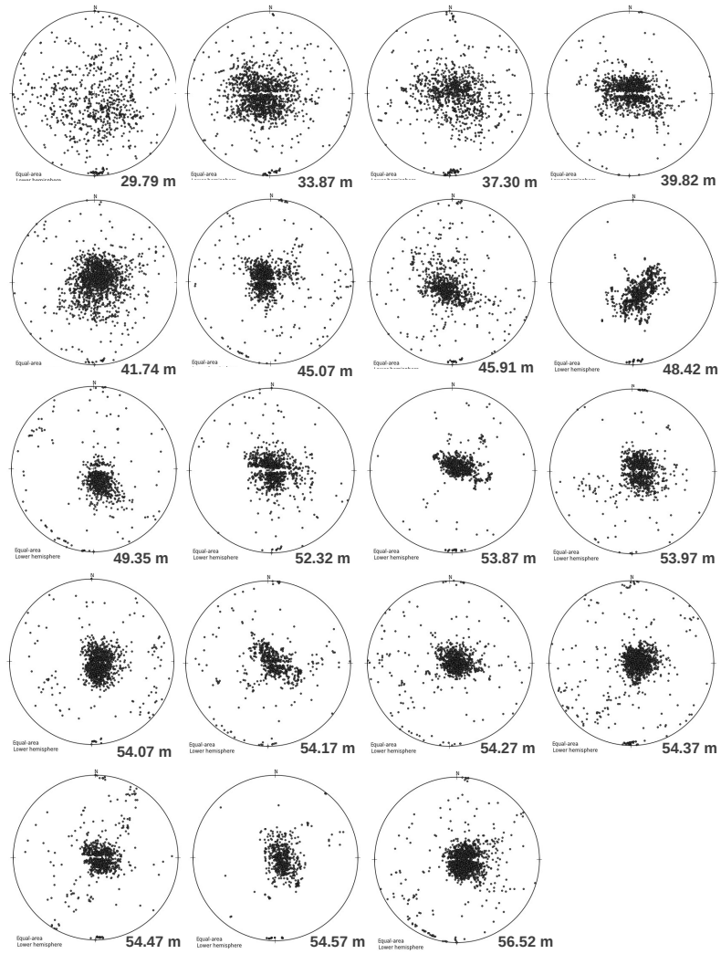
Fig. B.2: Schmidt diagrams for KCI thin sections (pers. comm. Jan Eichler, 2013). Each dot represents one c-axis. Depth is indicated on the bottom right. The interval is approx. 2–3 m with continuous thin section measurements between 53.87 and 54.57 m.
