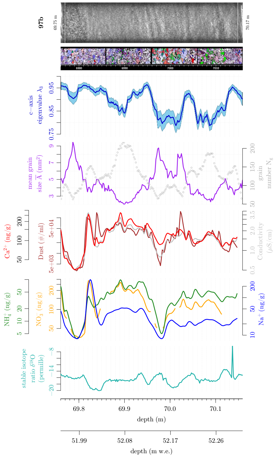
Fig. B.25: Fabric and microstructure parameters in cm-resolution in comparison with CFA data for KCC range 97b.
