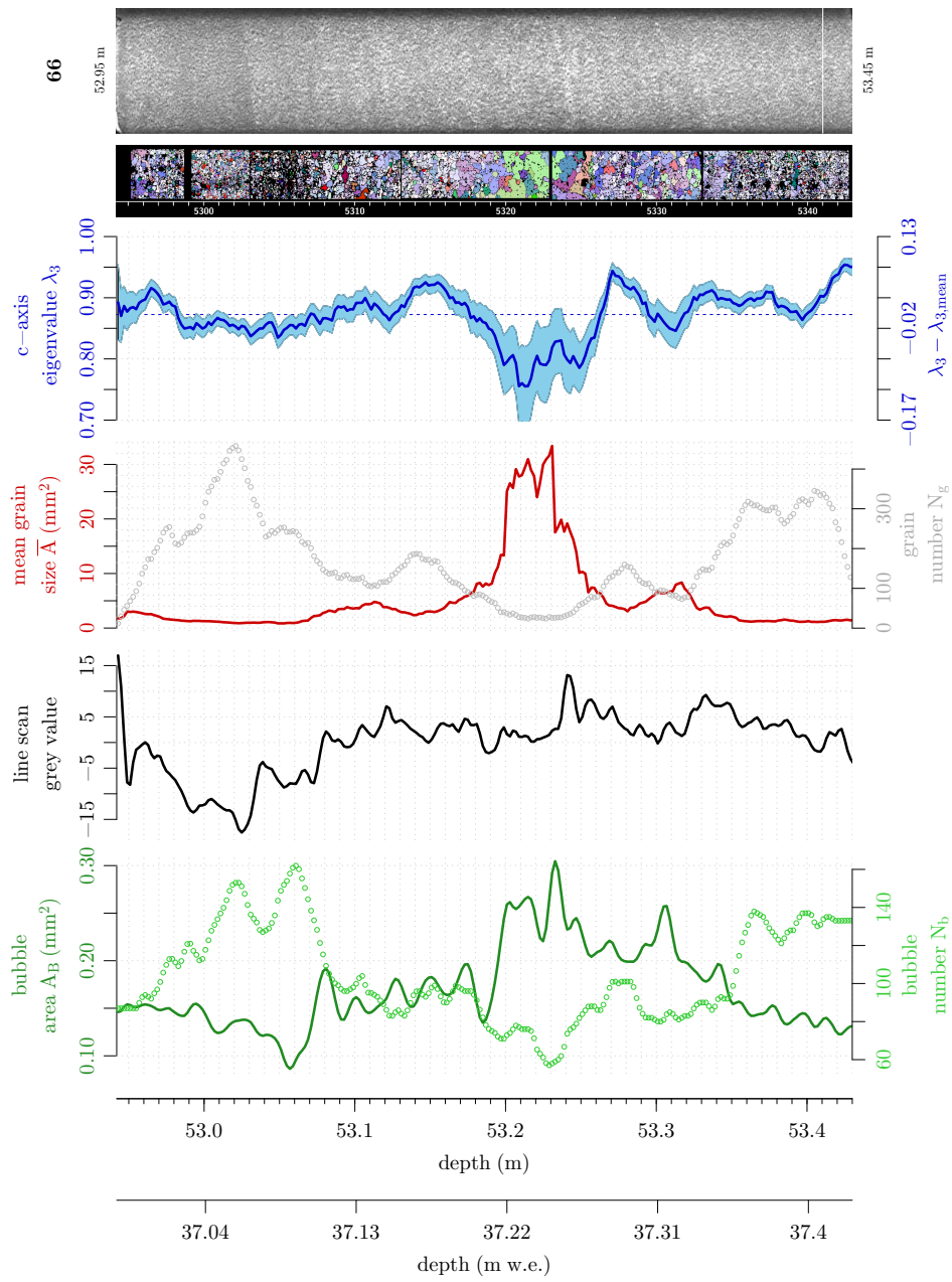
Fig. B.12: Fabric and microstructure in cm-resolution for KCC run 66. A thick layer of less oriented large grains with few large bubbles stands out.
