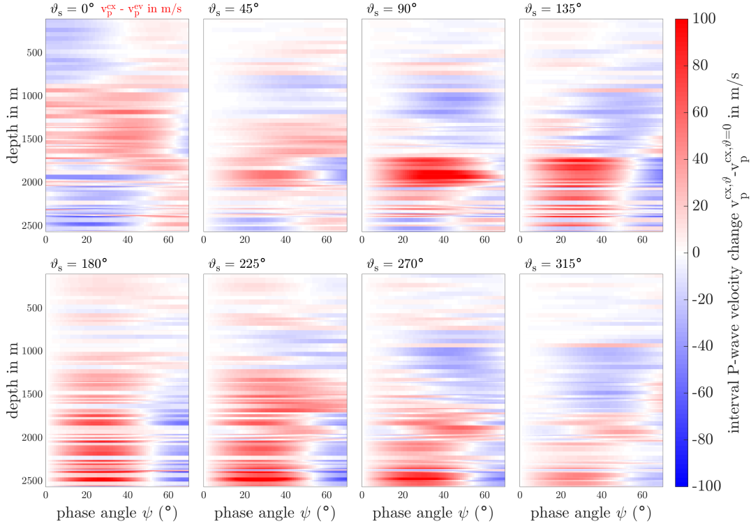
Fig. 6.8: Top left: Difference of EDML seismic P-wave velocity between c-axes and eigenvalue framework for incidence angles up to 70^\circ . Blue colour indicates overestimation of velocity by eigenvalue framework, red shades show the opposite. The other panels show the change in P-wave velocity, as calculated with c-axes framework for different seismic plane azimuth angles \vartheta_s , compared to \vartheta_s = 0^\circ .
