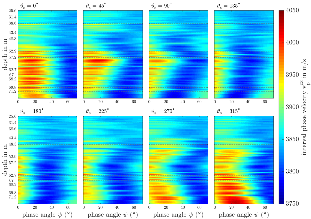
Fig. 6.11: Seismic P-wave velocities for KCC calculated with c-axes framework for incidence angles up to 70^\circ and eight seismic plane azimuth angles \vartheta_s . Note the breaks of the depth axis (dashed lines), where noted depth values refer to the top of the downward extending depth range.
