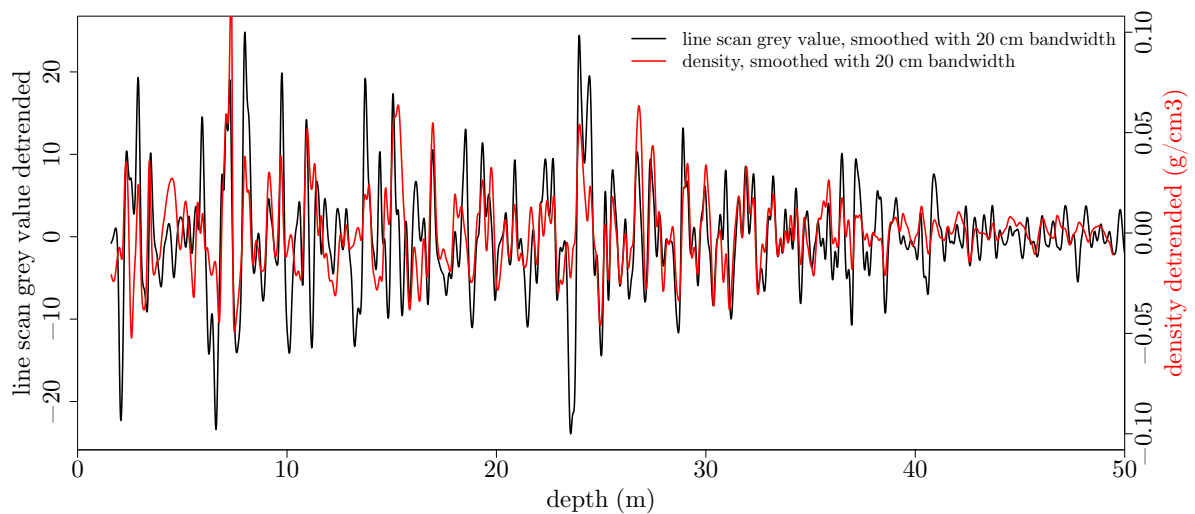
Fig. 4.3: Comparison of line scan grey value (black) and density profile (red). Both curves show the remaining variations after subtracting the mean grey value respectively the general density trend and subsequent smoothing with a 20 cm kernel.
