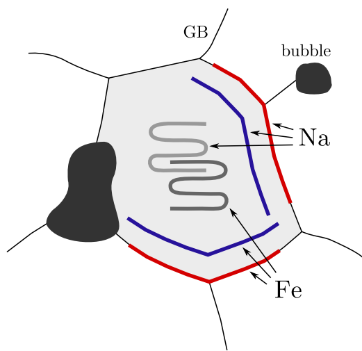
Fig. 3.18: Sketch of measurement coordination at a typical grain setting: ablation traces on and parallel to grain boundaries (red, blue) for different elements, interior raster in grey.
