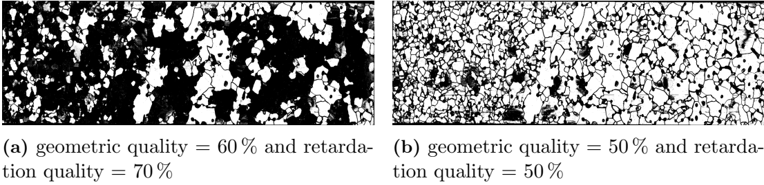
Fig. 3.12: cAxes output (sample 48-01, 10 cm wide) indicating in white which pixels are above the quality threshold and used for the analysis.
