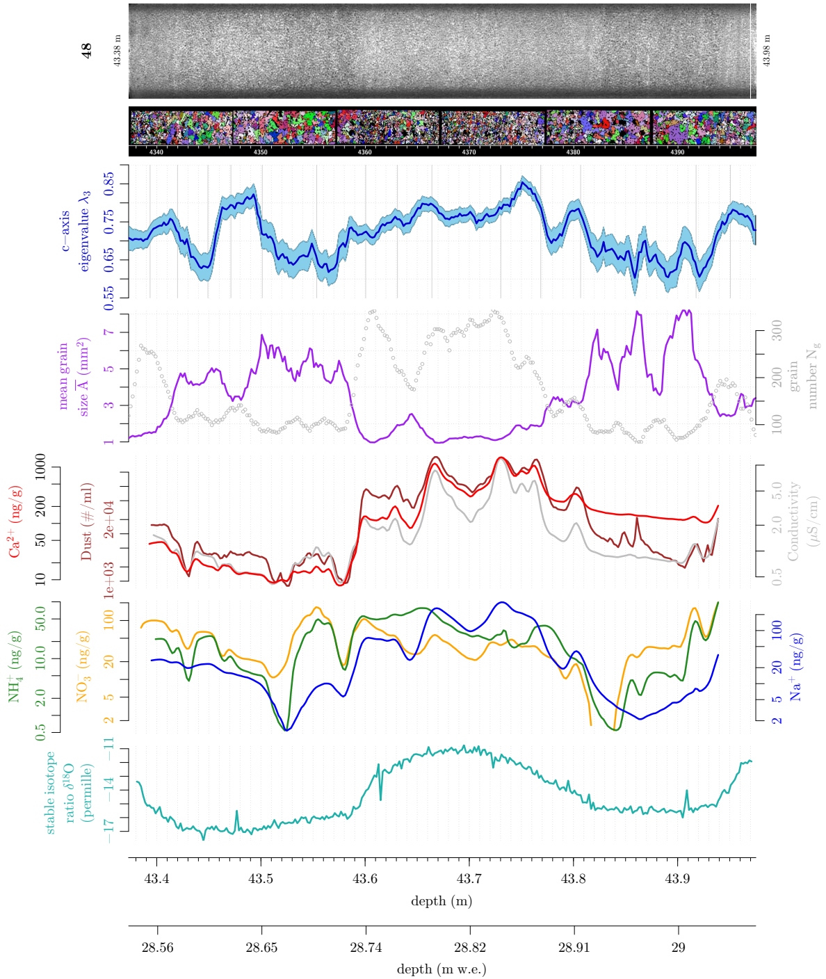
Fig. 5.2: Fabric and microstructure parameters in cm-resolution in comparison with CFA data for KCC range 48. Vertical grey solid lines indicate annual-layers as picked from CFA data. In this run correlations between all parameters can be found.
