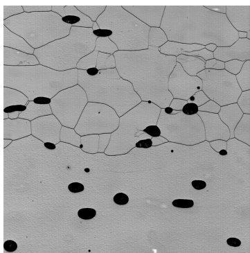
(g) Transition from small grain section to enormously large grain in 57.35 m depth, sample 75a-12.
