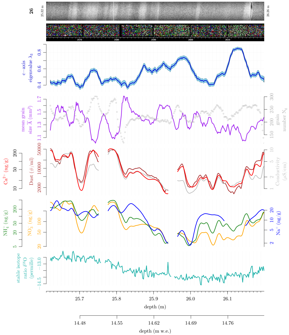
Fig. B.18: Fabric and microstructure parameters in cm-resolution in comparison with CFA data for KCC range 26.
