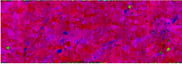
Fig. 4.18: Trend image of section 101-11 ( 3.2 \times 10 \text{ cm}^2 ), ice top on the left. Steeply inclined chains of similarly oriented grains can be observed. Red and pink shades correspond to (near-) vertical c -axis orientation.
