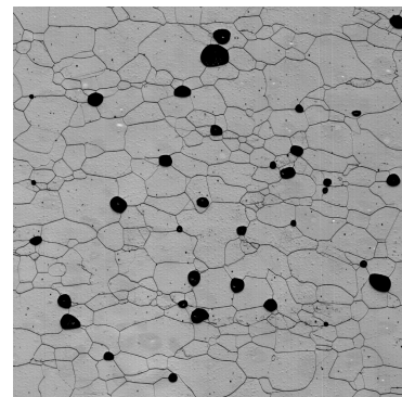
(f) Heterogeneous small grain section in 53.03 m depth, sample 66-21.
