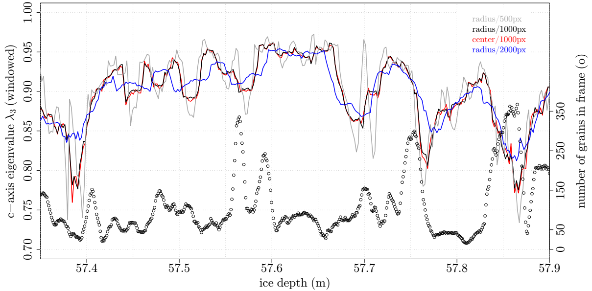
Fig. 3.14: Comparison of windowed eigenvalue computation with rMean for different frame length and grain-weighting ( center/radius ). Black circles give the number of grains in each frame.
