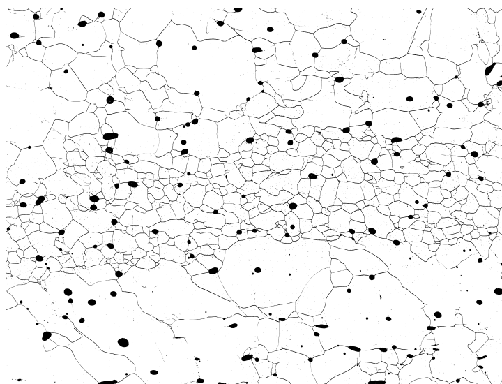
Fig. 5.12: Example ( 3 \times 2.3 cm 2 ) of a fine-grain layer ( \sim 7.5 mm thickness) at 68.3 m depth (sample 94-01).
