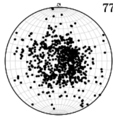
Fig. 2.3: Exemplary schmidt diagram for a thin section with 776 grains forming a weak cluster fabric (48-01 from KCC ice core).
