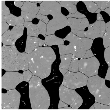
(a) Typical fine \mu\text{S} in 25.9 m depth, sample 26-61.
