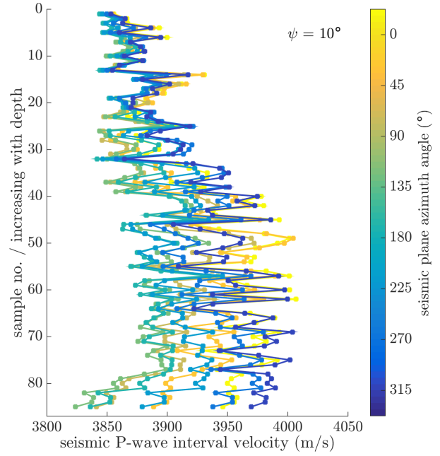
Fig. 6.12: Profiles of KCC seismic P-wave interval velocity for an incidence angle \psi of 10^\circ . The rotation of the seismic plane is color coded. For clarity the data points are plotted not against depth but are equidistant along the y-axis. The spread of velocities for a full rotation of the core for each sample exceeds 50 m/s for a large part of the samples, with up to 120 m/s for the bottom samples.
