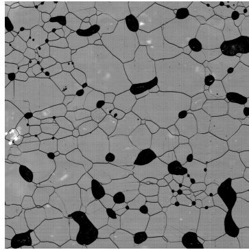
(b) Small grain/bubble clusters in 31.63 m depth, sample 32-41.
