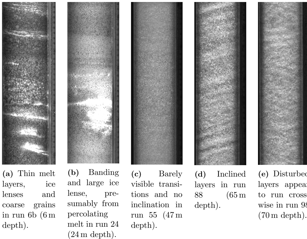
Fig. 4.1: Line scan image details (31 cm length, image top equals ice core top) illustrating different stratigraphic features observed in the KCC ice core.
