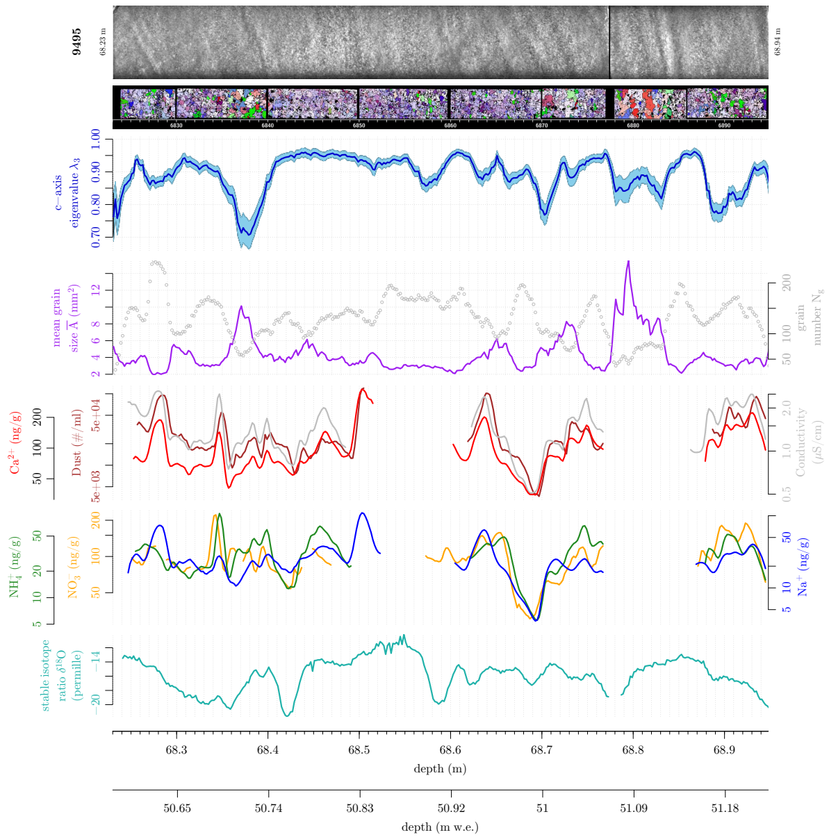
Fig. B.24: Fabric and microstructure parameters in cm-resolution in comparison with CFA data for KCC range 94/95.
