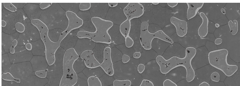
Fig. 3.9: Overlay of LASM images ( 25 \times 9 \text{ mm}^2 ) for illustrating pore space increase during sublimation. Light grey margins around bubbles show material loss at the pore margins during 6 hours. For a section in run 32 (above the FIT) at densities between 0.7 and 0.8 \text{ g/cm}^3 the pore space accounts for ca. 13.5% of the LASM image of the fresh surface. After 4 hours of sublimation the fraction is 17.4%, after 6 hours it is 18.7%.
