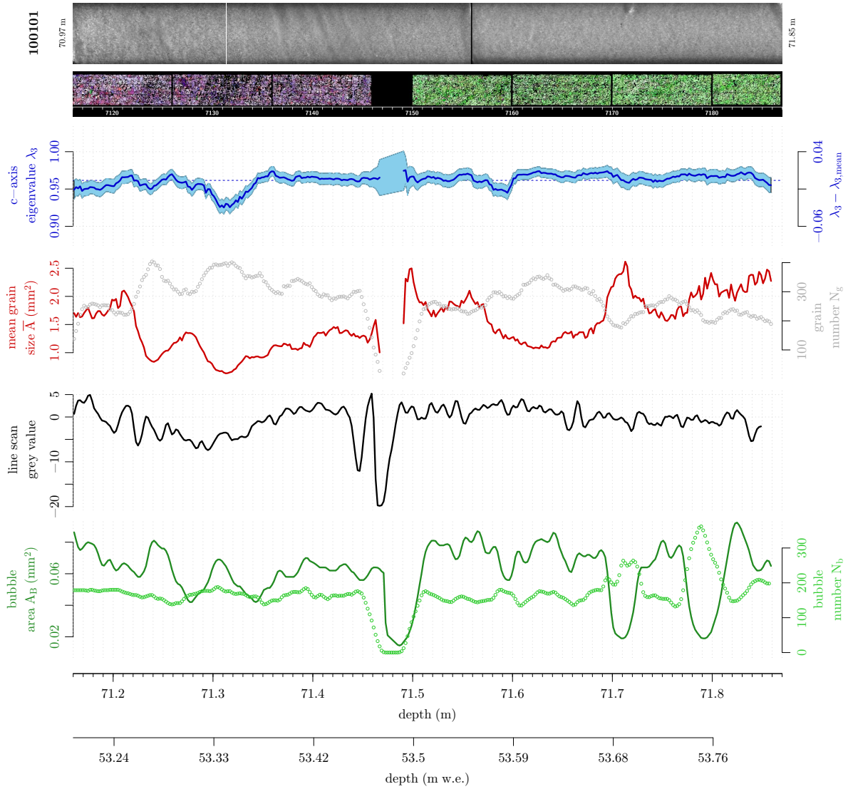
Fig. B.17: Fabric and microstructure in cm-resolution for KCC range 100/101. The basal microstructure is fairly homogeneous. The grain images are differently shaded due to different core azimuth. The lowermost run (green shades) exhibits very faintly steeply inclined structures marked by a slightly different c -axis orientation (Fig. 4.18).
