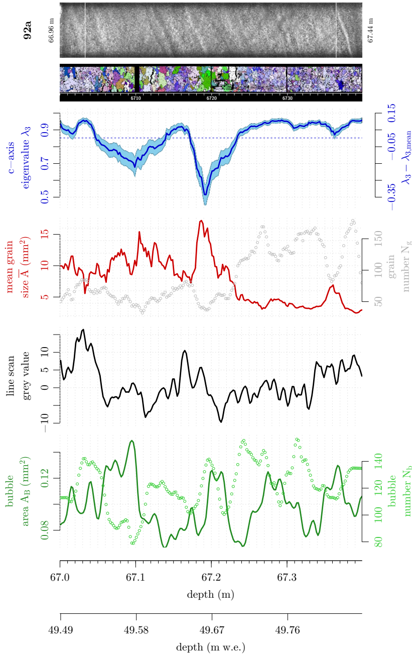
Fig. B.15: Fabric and microstructure in cm-resolution for KCC run 92a. This run is marked by a 20 cm long large-grain section that can be subdivided in three layers of alternating fabric strength. The strongest change in fabric strength in the entire data set is found at 67.2 m depth. The finer stratigraphy of inclined layers visible in the linescan is not represented in the fabric variations. For the upper part of the long section larger and fewer bubbles are observed.
