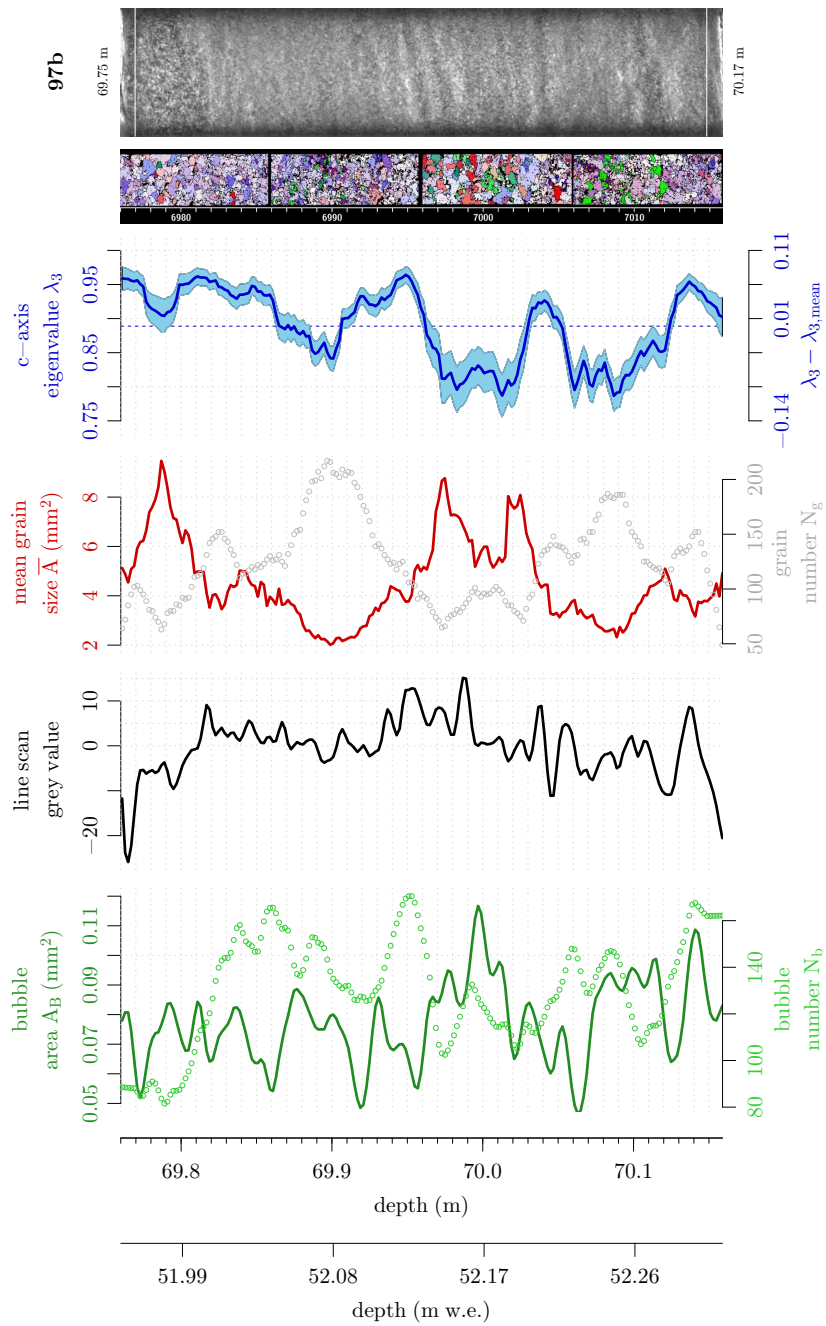
Fig. B.16: Fabric and microstructure in cm-resolution for KCC run 97b. Next to a large-grain section with less oriented grains the fabric is weakened in some sections by several scattered grains with a c-axis orientation almost perpendicular to the cone orientation. These grains contribute to the faint girdle apparent in Fig. 4.9 and B.1.
