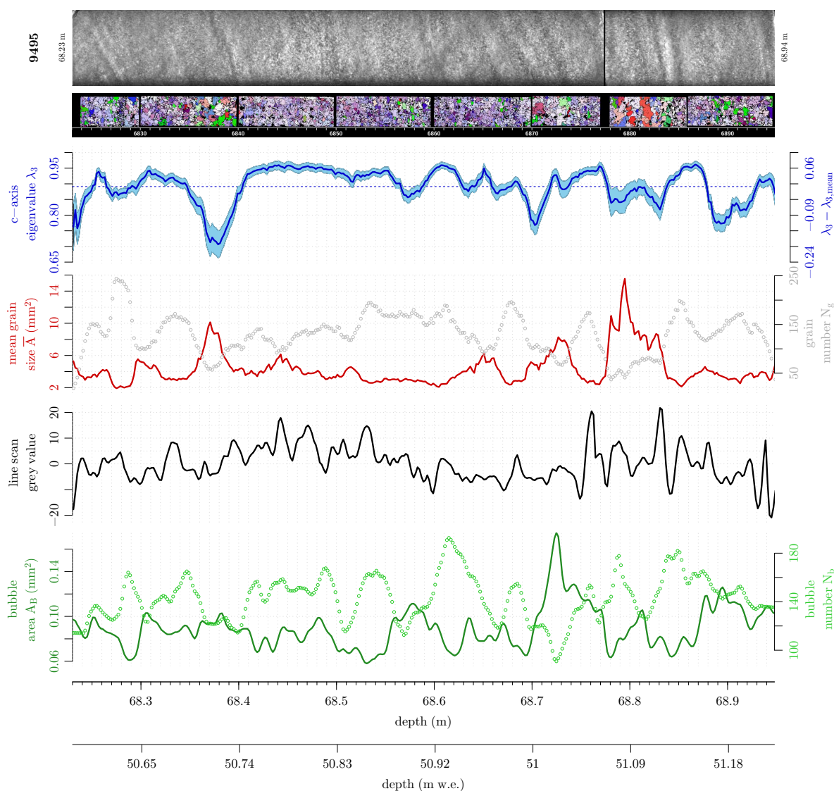
Fig. 4.22: Fabric and microstructure parameters in cm-resolution for KCC range 94/95. Some less oriented large-grain layers or single grains can be observed. The microstructural parameters appear more independent, other than the occasional inverse eigenvalue/mean grain size relationship. The line scan shows inclined layers down to the order of 1 cm thickness which have no representation in the eigenvalue.
