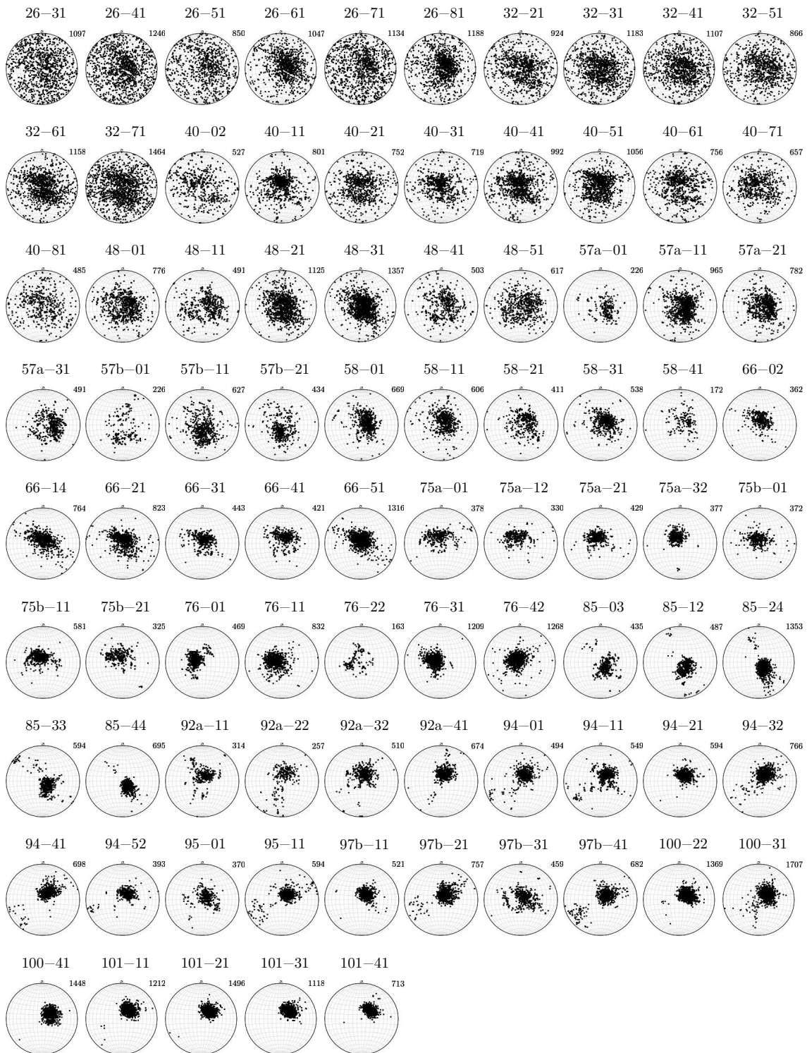
Fig. B.1: Schmidt diagrams for all KCC thin sections. Each dot represents one c-axis. Number of axes is indicated on the top right of each pole figure.
