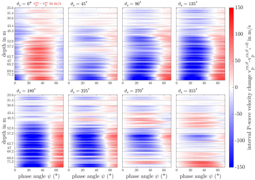
Fig. 6.13: Top left: Difference of KCC seismic P-wave velocity between c-axes and eigenvalue framework ( v_p^{cx} - v_p^{ev} ) for incidence angles up to 70^\circ . The other panels show the change in P-wave velocity as calculated with c-axes framework for different seismic plane azimuth angles \vartheta_s compared to \vartheta_s = 0^\circ . Note the breaks of the depth axis where noted depth values refer to the top of the downward extending depth range.
