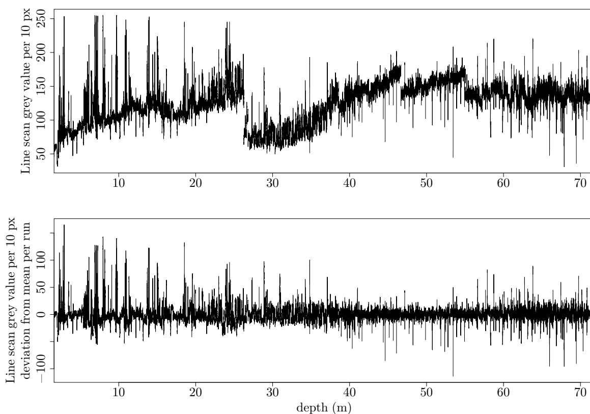
Fig. 3.15: Grey value averaged over 10 pixel lines from line scan images of KCC. Top panel: absolute grey values depending on illumination on recording of the images; jumps correspond to illumination changes. Bottom panel: Grey value difference from image mean grey value.
