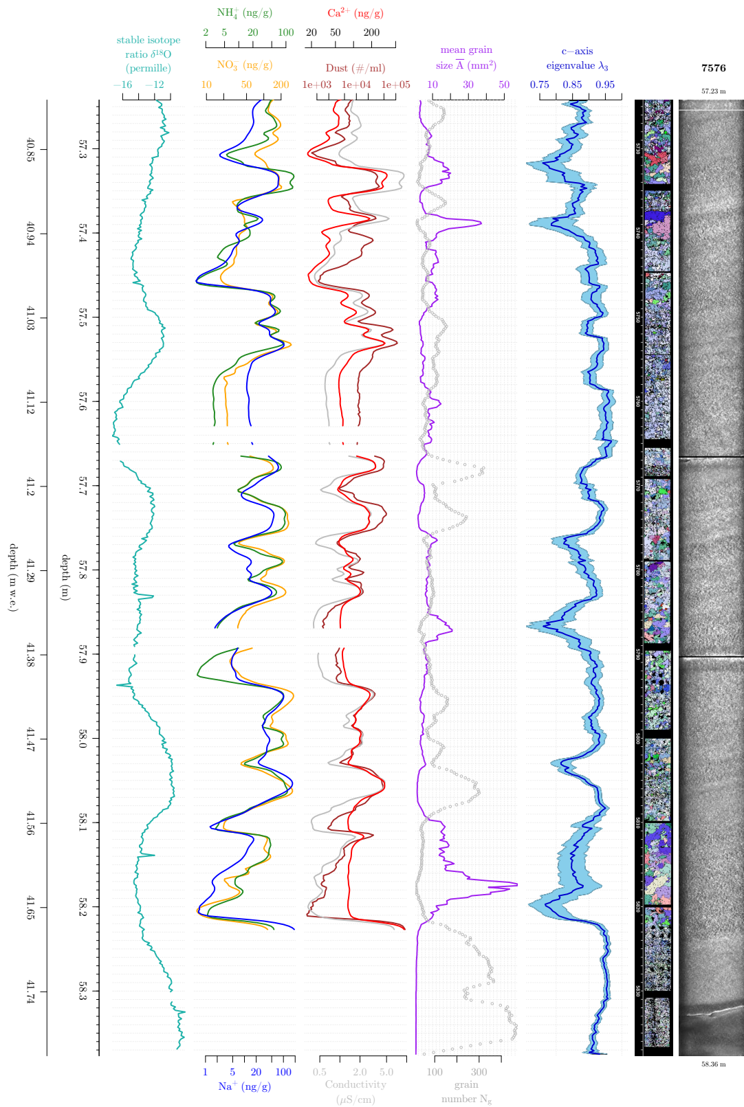
Fig. 5.3: Fabric and microstructure parameters in cm-resolution in comparison with CFA data for KCC range 75/76.
