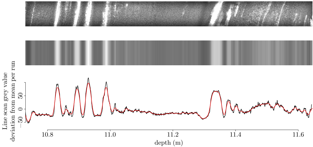
Fig. 4.2: Illustration of grey value stratigraphy from line scan images (run 11b, 93 cm long, from 10.7 m depth). Top panel: Line scan raw image. Middle: Grey value image. Bottom panel: Grey value line graph in 0.05 mm resolution (black) and smoothed with 1 cm bandwidth (red).
