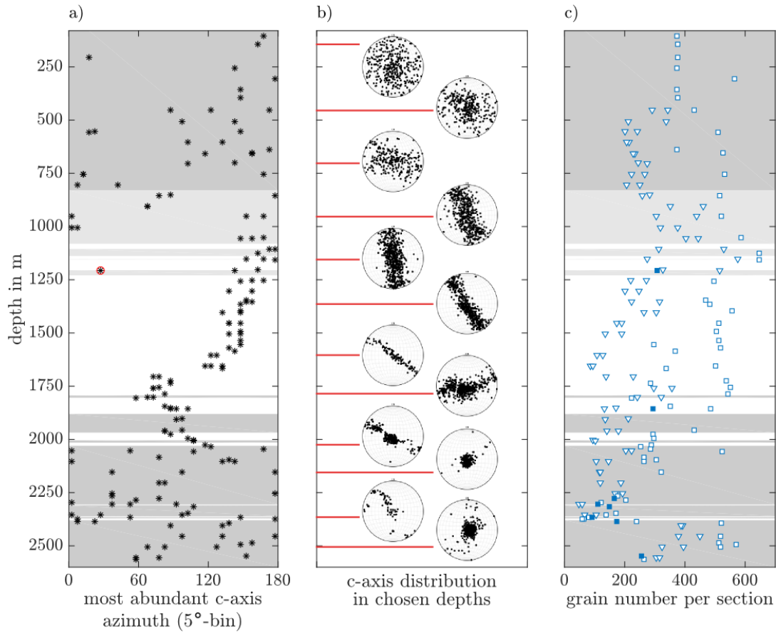
Fig. 6.7: Additional information on EDML's c-axes distributions. Shading as in Fig. 6.5. a) From the c-axis azimuth angle distribution of each sample the approximate direction of the girdle is found (5° angle interval). One data point appearing as outlier (red circle) could not be corrected. b) Examples of stereographic projections for different depths illustrate the development from isotropic/cone to girdle and back to cone fabric. c) shows the number of grains in each thin section sample with symbols as in Fig. 6.6. The total area of vertical thin sections is generally larger and contains more grains.
