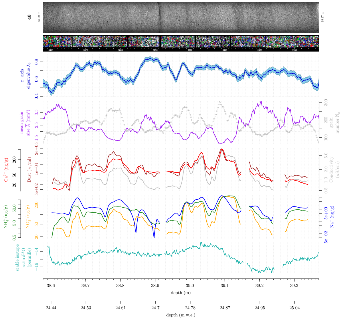
Fig. B.19: Fabric and microstructure parameters in cm-resolution in comparison with CFA data for KCC range 40.
