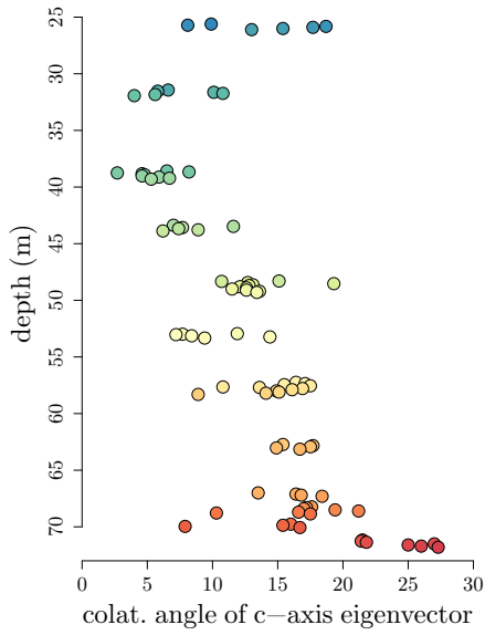
Fig. 4.5: Colatitude angle of c-axis eigenvector with respect to the ice core axis for each sample. Color as in Fig. 4.6.
