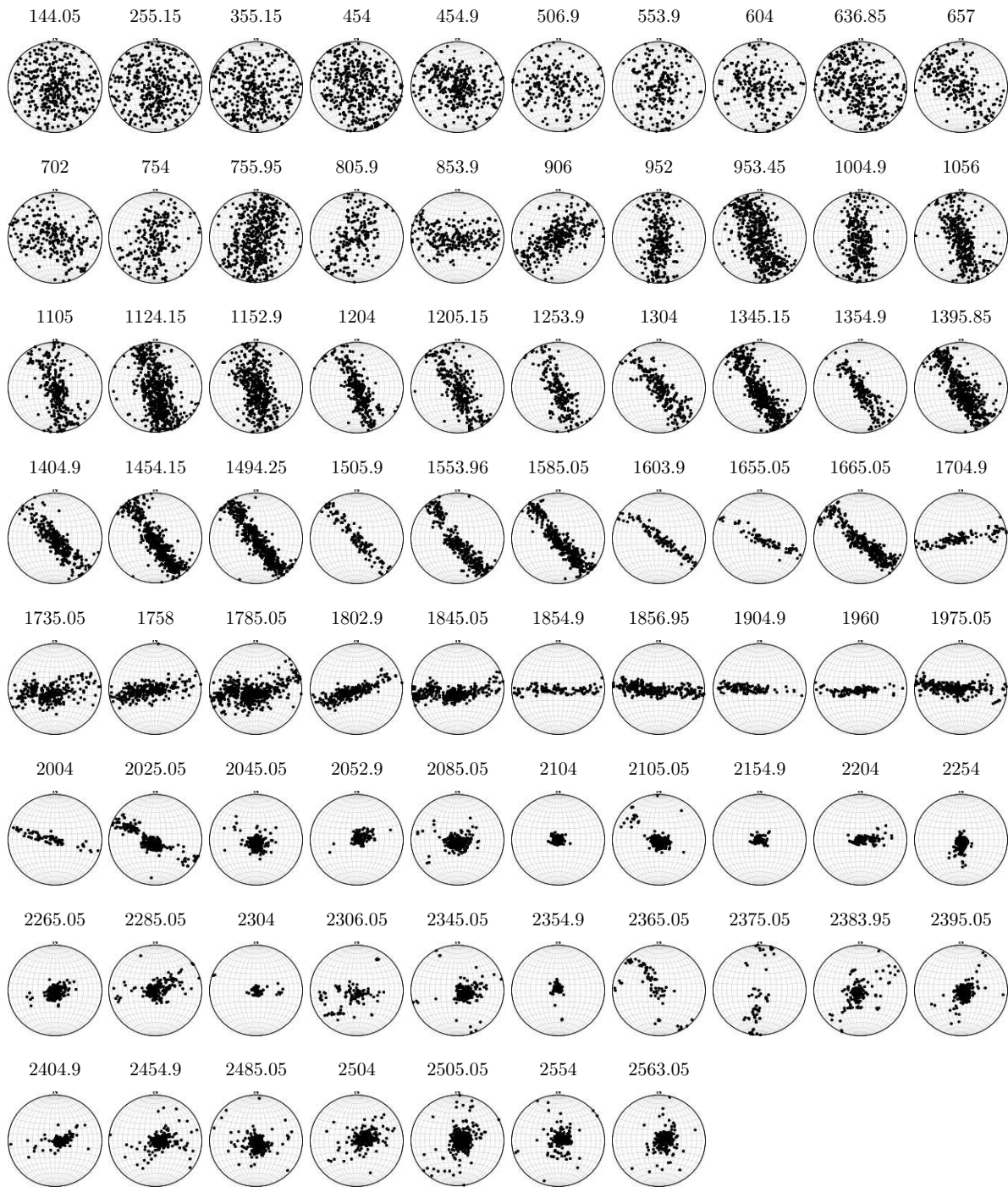
Fig. B.3: Schmidt diagrams for every second EDML thin sections used in this study. Each dot represents one c-axis.
