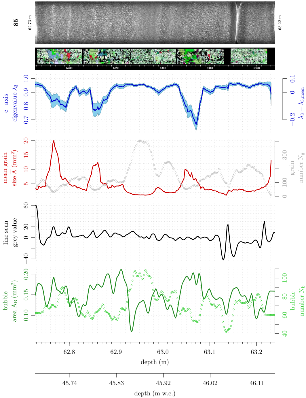
Fig. B.14: Fabric and microstructure in cm-resolution for KCC run 85. Three less oriented large grain layers with a tendency of larger bubbles are apparent. Line scan grey value peaks are again artificially induced from breaks and gaps, otherwise nondescript. The greenish shades of the grain images is due to the different core azimuth of this run as compared to most other runs with shades of purple.
