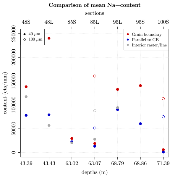
Fig. 5.8: Summary of the mean sodium content from all grains of each section for different locations. S and L denote small- or large-grained.
