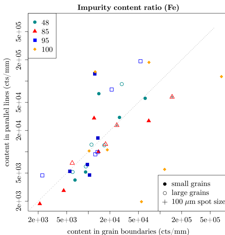
Fig. 5.11: The ratio of iron content is illustrated. For about a third of all grains the ratio is above 1, indicating higher iron content in the grain interior. Some grains of the basal section appear as outliers.
