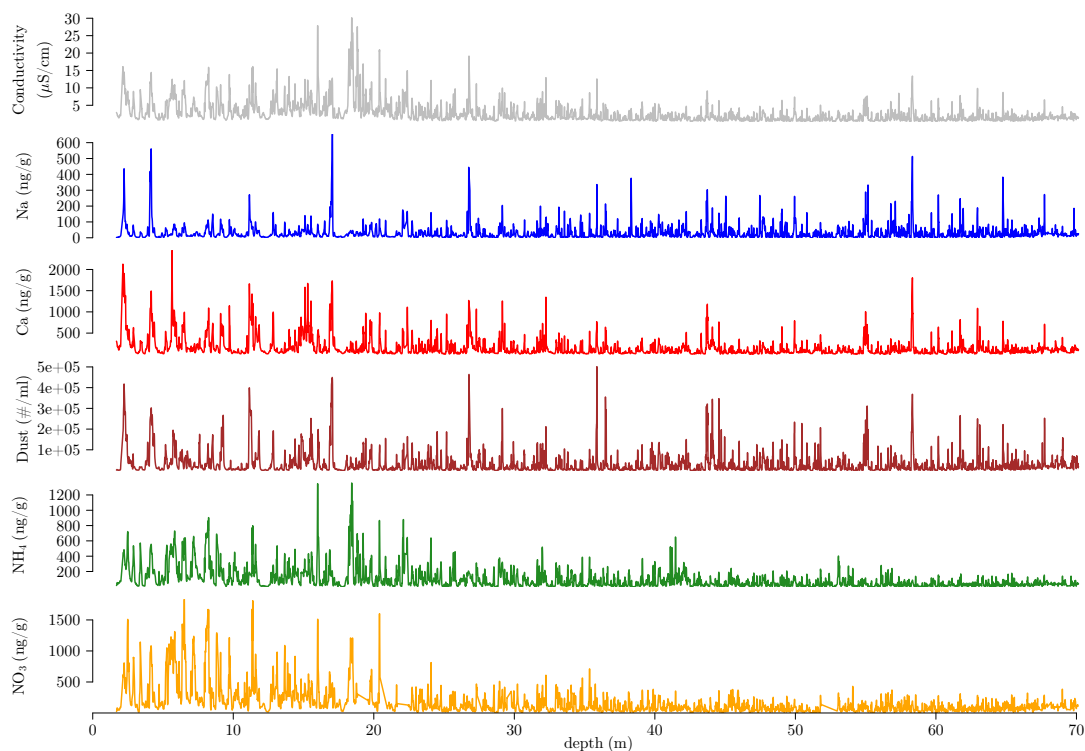
Fig. B.4: CFA data from KCC ice core (pers. comm. H. Fischer/T. Erhardt, University of Bern, 2014). Conductivity, calcium ( \text{Ca}^{2+} ), sodium ( \text{Na}^+ ), particulate dust content, ammonium ( \text{NH}_4^+ ) and nitrate ( \text{NO}_3^- ) were measured and are shown here smoothed with 2 cm bandwidth.
