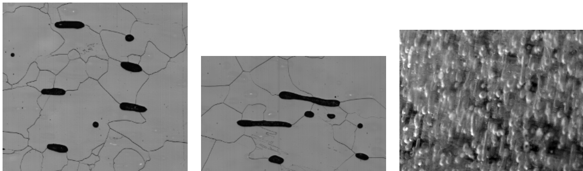
(a) LASM image detail from sample 85-01, 9 \times 8 \text{ mm}^2 . (b) LASM image detail from sample 85-11, 9 \times 6 \text{ mm}^2 . (c) Photo detail from ^{14}\text{C} aliquot of run 77a, approx. 1 \times 1.5 \text{ cm}^2 .
