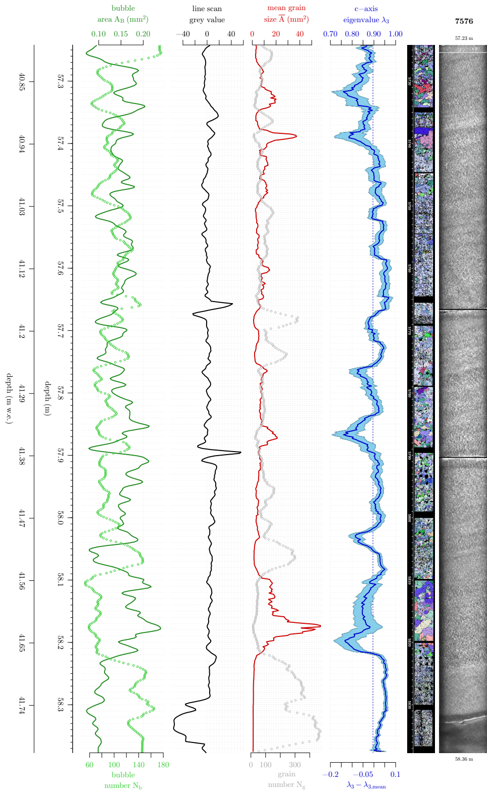
Fig. B.13: Fabric and microstructure in cm-resolution for KCC range 75/76. Several less oriented large-grain layers can be observed, including some strong grain size gradients. Only for a more than 10 cm long section with enormous grains fewer and larger bubbles can be found. At the bottom of this range a stark change in the line scan coincides with a break. The peaks in line scan grey value at 57.65 and 57.89 m depth are artificial.
