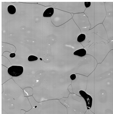
(d) Small single grains and zigzagging subGB in 43.87 m depth, sample 48-51.
