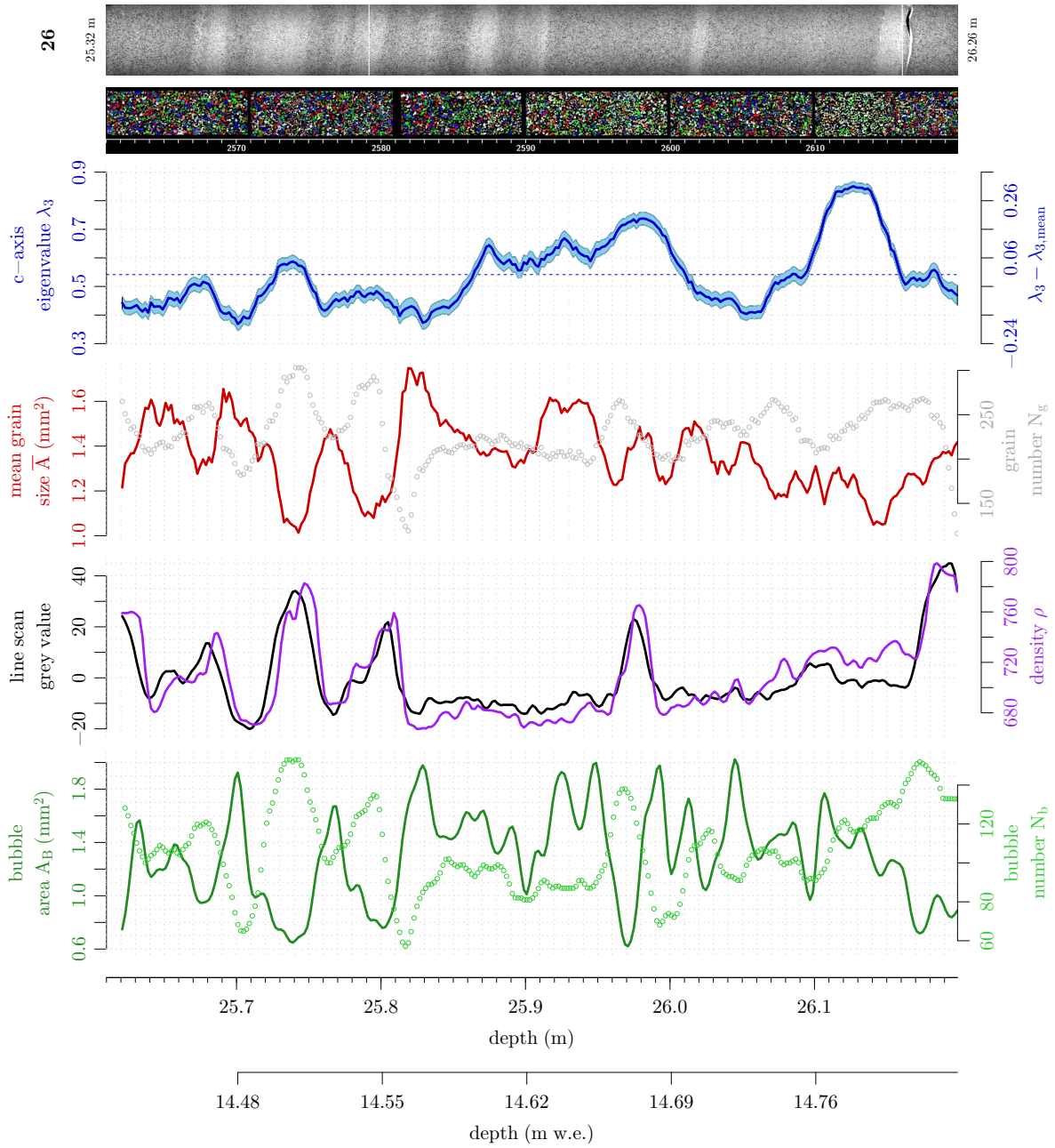
Fig. B.8: Fabric and microstructure in cm-resolution for KCC run 26. The eigenvalue appears largely independent of the other microstructural parameters which relate to each other to a certain degree. Strongest eigenvalue variability of all ranges. Only the middle part (between white lines) of the line scan corresponds to the parameter records.
