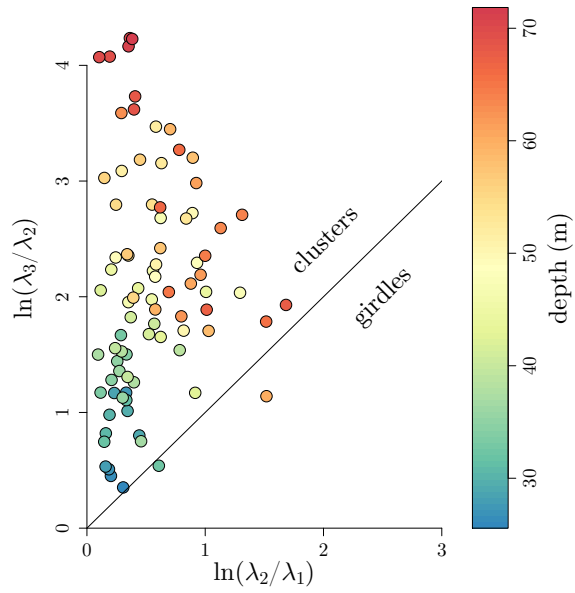
Fig. 4.6: Woodcock diagram illustrating the predominant cluster classification of KCC fabric.
