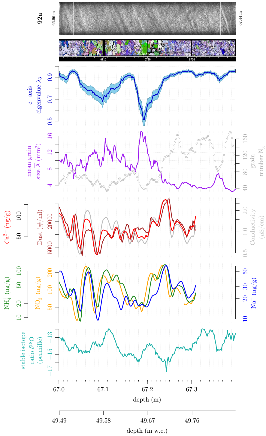
Fig. B.23: Fabric and microstructure parameters in cm-resolution in comparison with CFA data for KCC range 92a.
