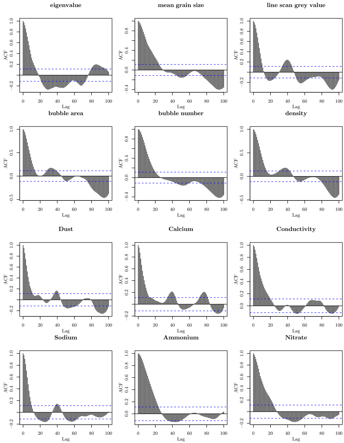
Fig. B.7: Autocorrelation for fabric, microstructure and impurity data of range 32 is shown exemplarily. The lag is given in 2 mm steps, max. lag 20 cm.
