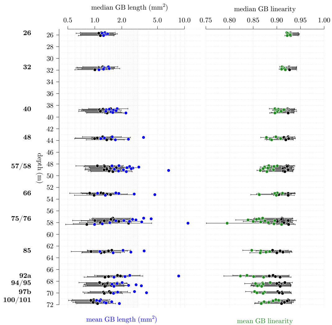
Fig. 4.14: The evolution of grain boundary length and linearity with depth. Median values and interquartile range per thin section sample are shown in black, mean values are shown in blue (GB, on a log-scale) and green (linearity).
