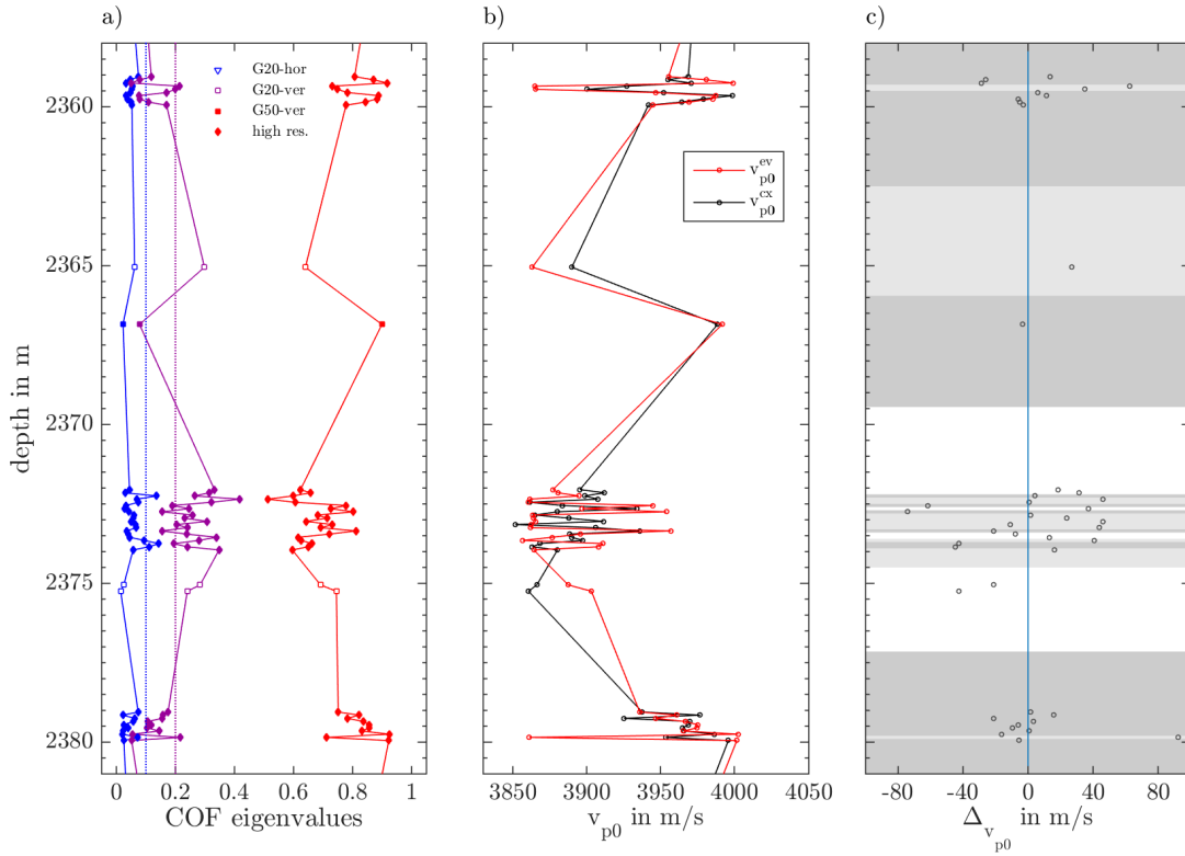
Fig. 6.6: Comparison of P-wave velocities at vertical incidence, calculated from EDML fabric data that was measured in high resolution between 2358 and 2380 m depth . The panels show the same variables as in Fig. 6.5, lines are for visual assistance. The different symbols used for eigenvalue data indicate horizontal (hor) and vertical (ver) thin sections, and fabric analyser model. The recent measurements in high resolution (diamonds) were done with the G50 instrument.
