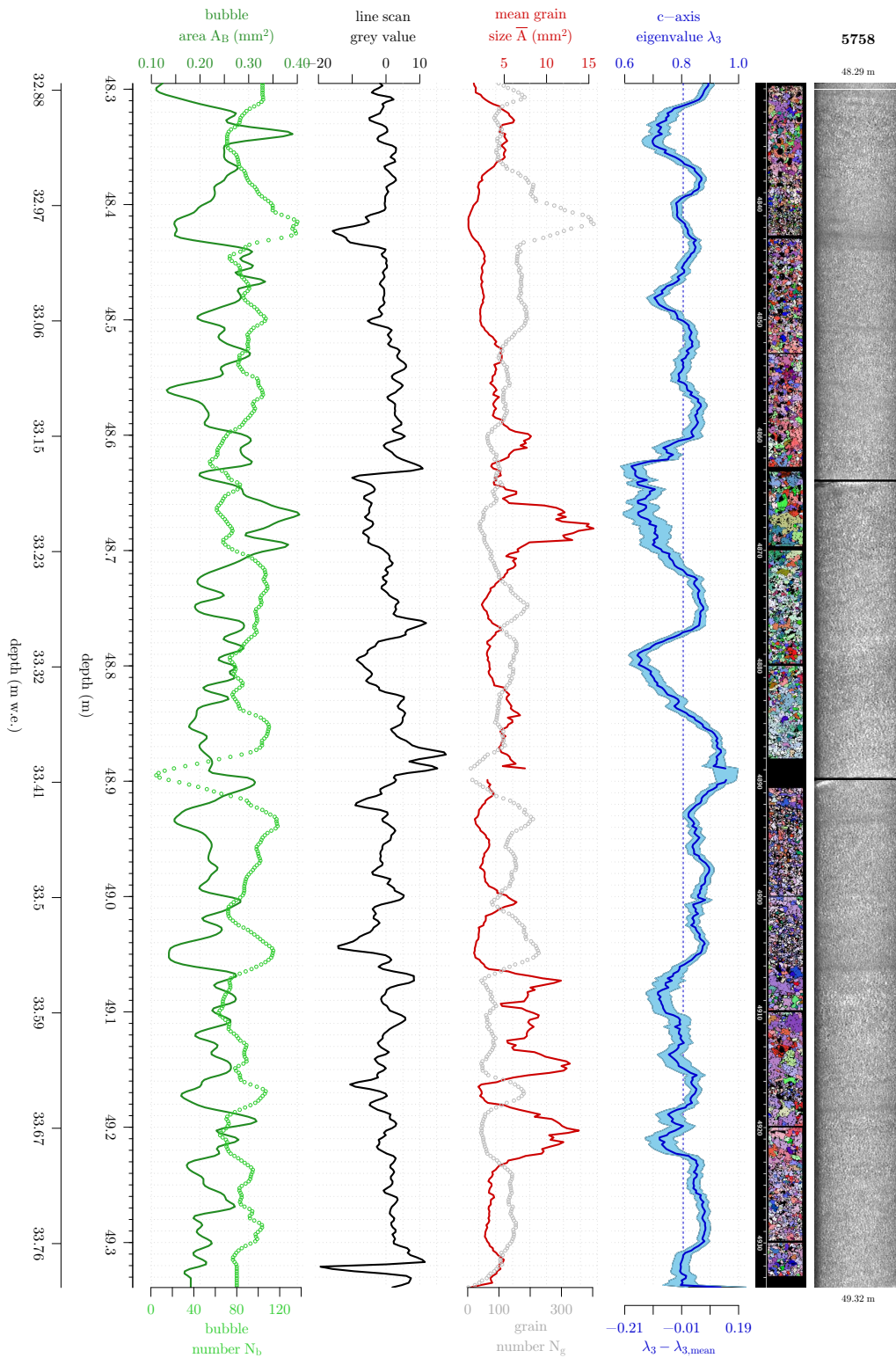
Fig. B.11: Fabric and microstructure in cm-resolution for KCC range 57/58. Some layers with fairly large grains have low eigenvalues. Transitions in the line scan stratigraphy appear to coincide with fabric layer transitions when comparing both the records and the images.
