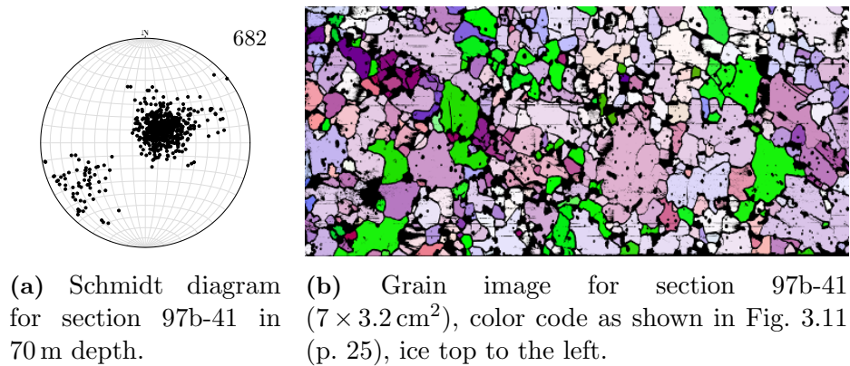
Fig. 4.24: Next to a slightly inclined strong single maximum a second maximum appears in the schmidt diagram, corresponding to the green grains, oriented approximately 90^\circ away from the first. They consist of both large and small grains, sometimes clustered but otherwise distributed in the single maximum grain matrix.
