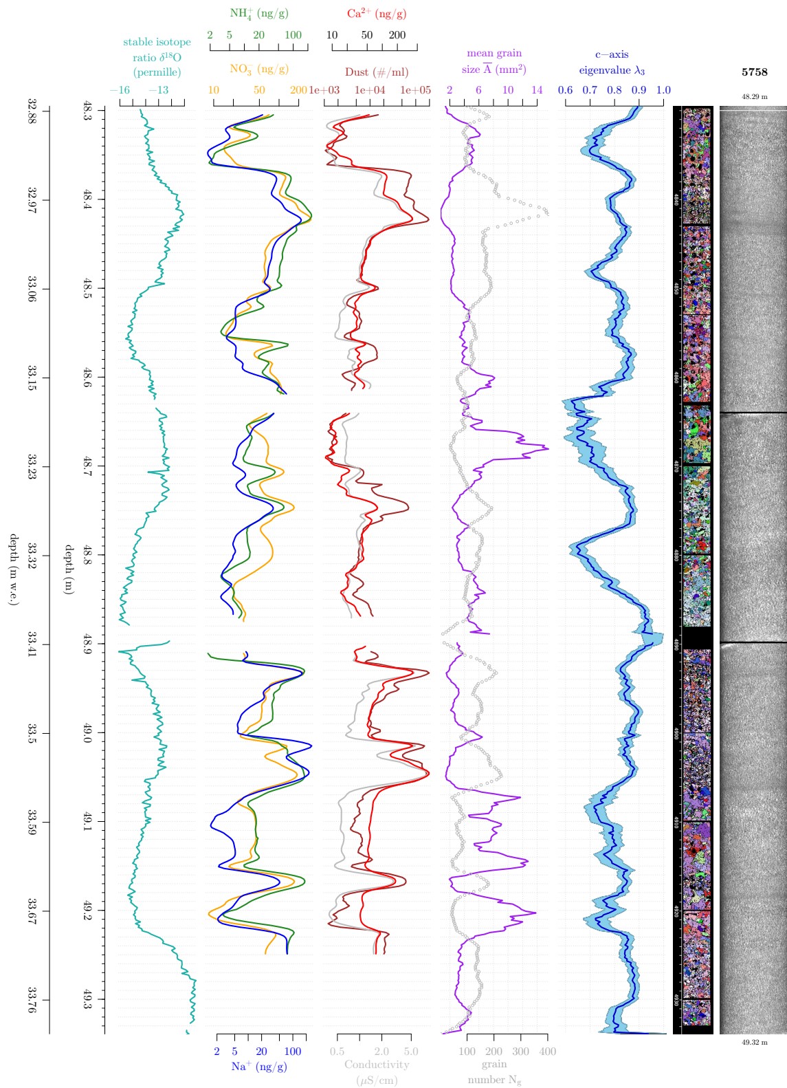
Fig. B.20: Fabric and microstructure parameters in cm-resolution in comparison with CFA data for KCC range 57/58.
