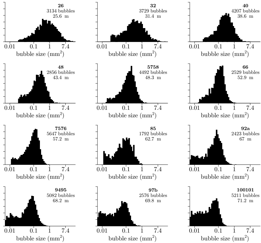
Fig. 4.15: Bubble size distributions for all KCC ranges. The bins are logarithmically spaced. The frequencies are normalised but total bubble number per range is indicated.
