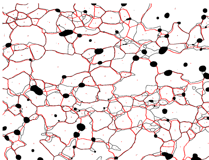
Fig. 3.13: Exemplary matching of grain boundaries (sample 48-51, 2.3 \times 1.7 \text{ cm}^2 ) extracted from LASM (black) and FA (red) images (pers. comm. T. Binder, 2016). In fine-grained regions the cAxes algorithm shows a tendency to neglect very small grains. Part of these grains with a very similar orientation could be subgrains while others show a distinct different orientation (verified on trend image).
