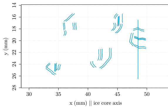
Fig. 3.19: Laser ablation traces are plotted from coordinates collected during the measurement of a large grain section. The area corresponds to the surface area of the ice accessible with the laser during a set of measurements, i.e. within a yellow box as shown in Fig. 3.16. Features of five grains can be distinguished. The vertical line which is still visible with the naked eye on the ice surface after the measurement is used as depth anchor.
