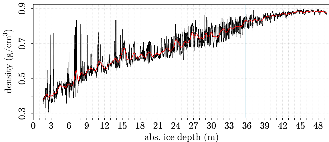
Fig. 3.7: High resolution density for the upper 50 m of the KCC ice core with corrected depth scale. The high resolution density data were smoothed with a bandwidth of 0.005 m and 0.5 m (red). The depth of the firn-ice-transition is indicated in lightblue.
