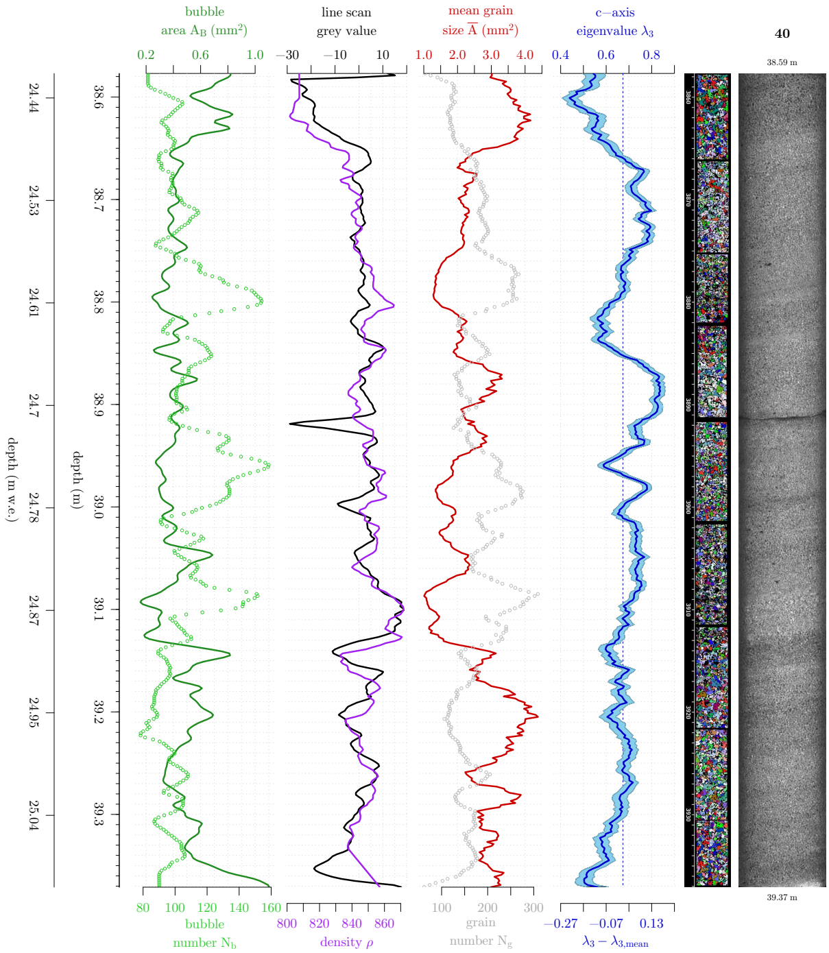
Fig. B.10: Fabric and microstructure in cm-resolution for KCC run 40. The line scan grey value peak at 38.92m is due to a break. While line scan and eigenvalue have a common tendency in some places, the inverse relation between grain size and eigenvalue is barely apparent. Third strongest short-scale variability in eigenvalue.
