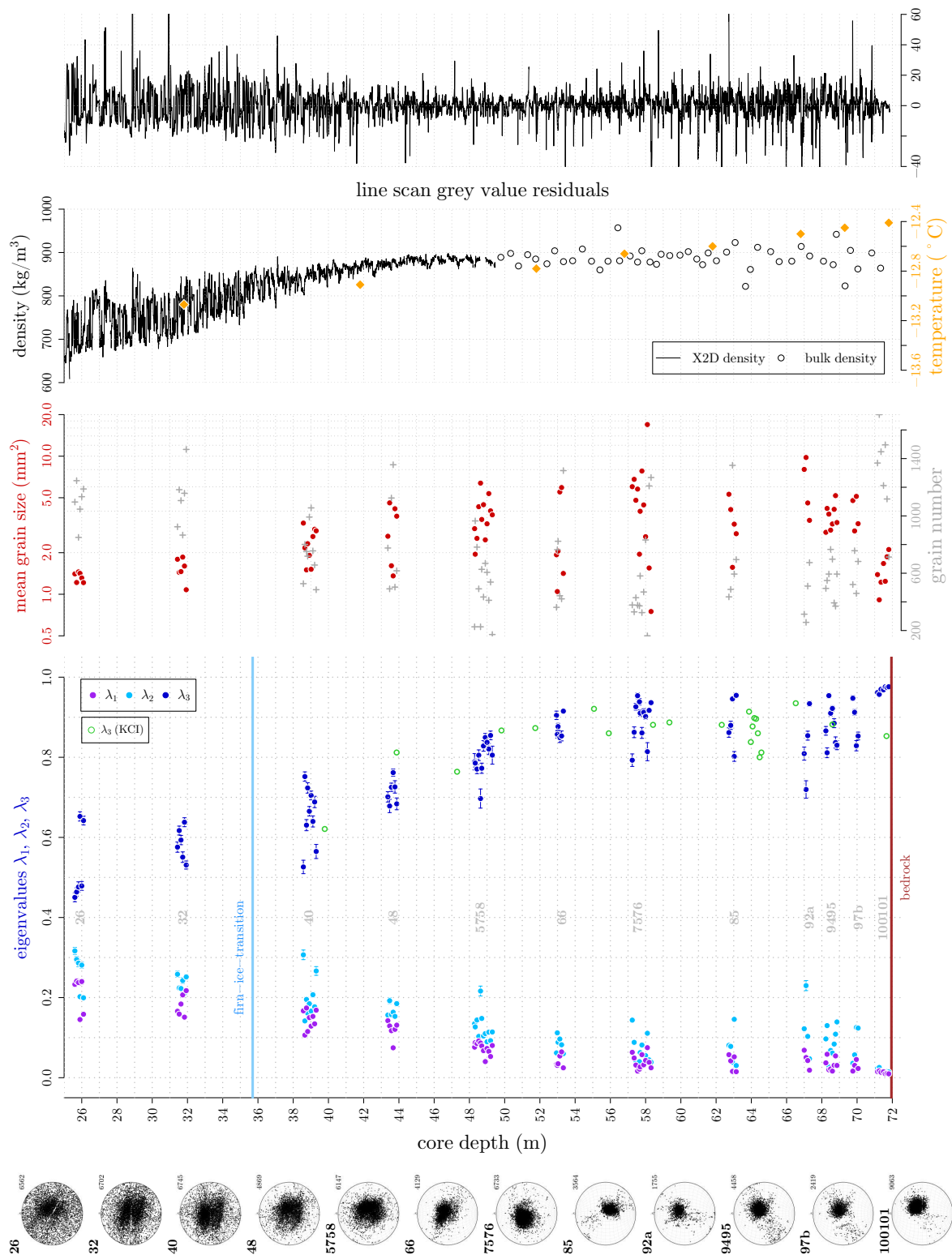
Fig. 4.9: Illustration of KCC fabric evolution with depth. Schmidtplots in classical glaciology projection (center of diagram refers to vertical core axis) show the c-axis distribution with the total number of grains indicated on the top right. Eigenvalues of the orientation tensor are shown with uncertainty. Mean grain size, density, temperature and line scan grey value residuals are shown for comparison.
