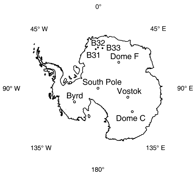
Figure 1. Geographical locations of the drill sites of the DML cores B31, B32, and B33, together with major deep ice core drillings of Antarctica.
