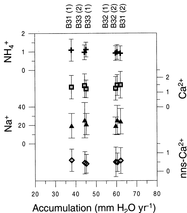
Figure 4. Mean concentrations of ammonium (cross), calcium (square), sodium (triangle), and nss calcium (diamond) in ppb as a function of average accumulation rates. The different time periods are indicated as (1) 500-900 AD and (2) 1100-1980 AD. Variation is given in one standard deviation from annual mean.
