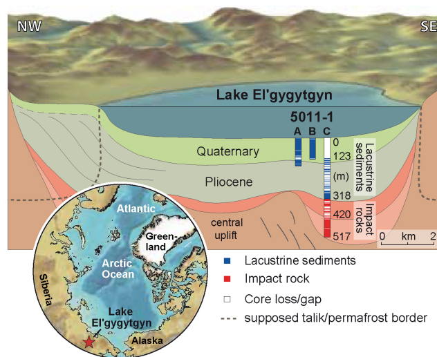
Fig. 1. Location of Lake El'gygytyn in north-eastern Russia (inserted map) and schematic cross-section of the El'gygytyn basin stratigraphy showing the recovery of holes A, B, and C at ICDP Site 5011-1 (modified after Melles et al., 2012).
