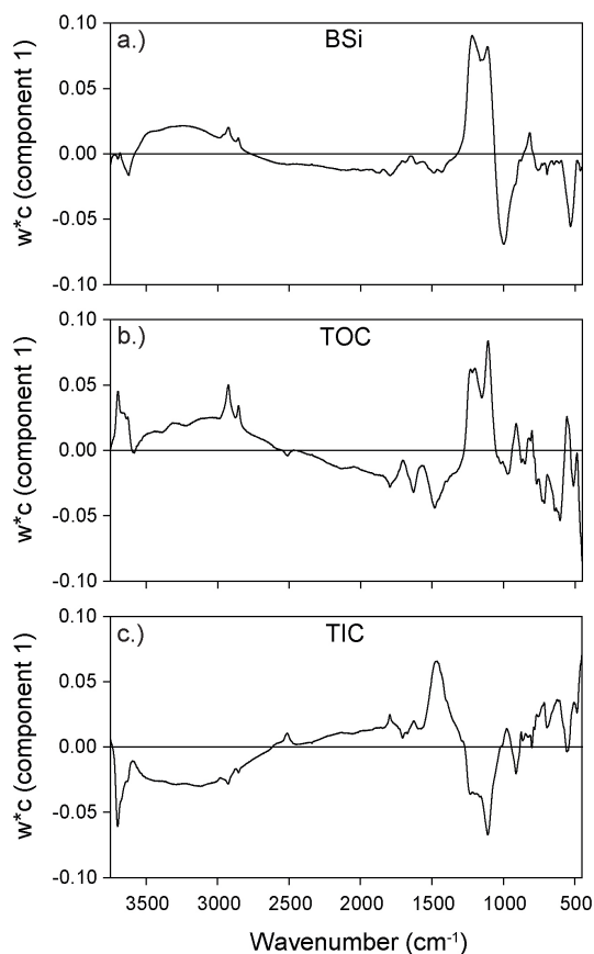
Fig. 3. Loadings of the developed FTIR-calibration models for (a) biogenic silica (BSi), (b) total organic carbon (TOC), and (c) total inorganic carbon (TIC) showing the contribution of each wavenumber to the partial least squares (PLS) regression model. Positive values indicate wavenumbers positively correlated with the property of interest and negative values indicate wavenumbers negatively correlated with the property of interest. Loadings are expressed by weight vectors ( w \times c ) of the first PLS model component ( x axis) and the corresponding spectral range ( y axis). The calibration models are based on sediment samples from percussion piston cores PG1351 ( n = 83 for BSi, n = 156 for TOC) and LZ1024 ( n = 204 for BSi) and samples distributed throughout the entire drill core composite profile of ICDP site 5011-1 ( n = 133 for BSi, n = 153 for TOC, n = 152 for TIC).
