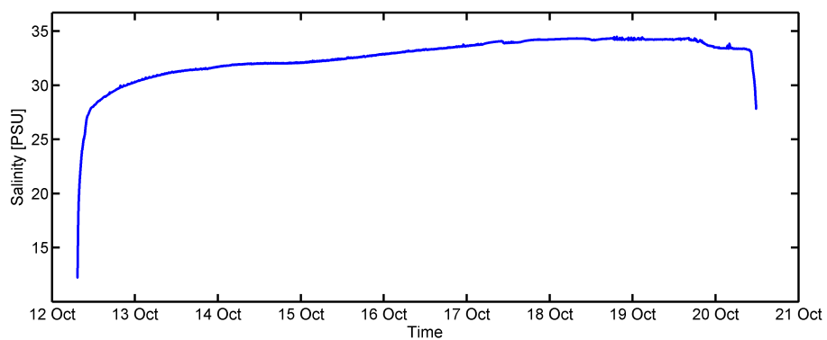
Figure 4: Salinity after geofilter.
