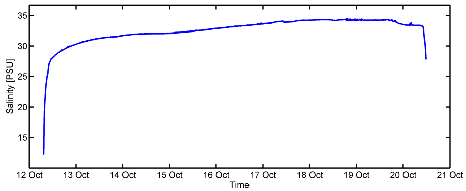
Figure 6: Salinity after temperature filter.
