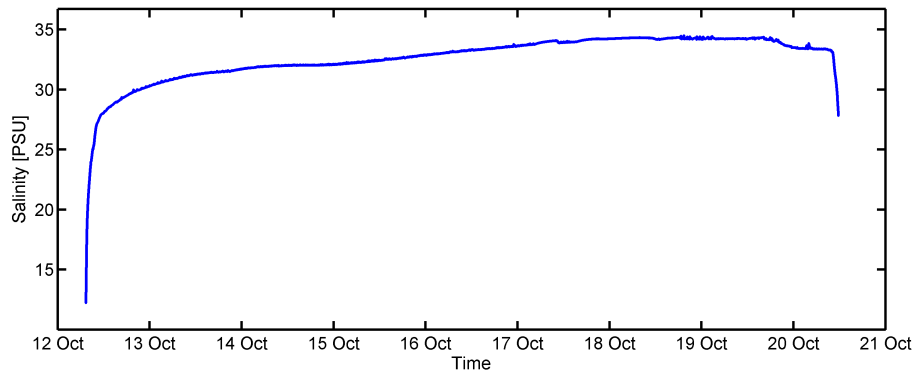
Figure 5: Salinity after speed filter.
