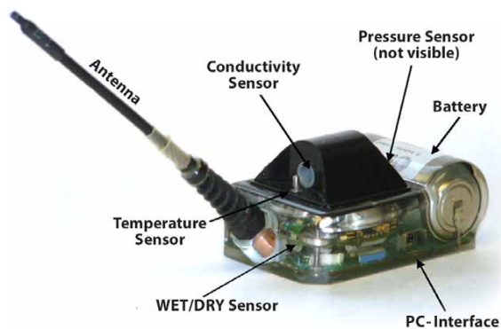
FIGURE B1. Photograph of a CTD-SRD, with visible hardware components labeled. The tag is housed in normal solid epoxy rated either to 500 m or 2,000 m depth. Standard sensors include pressure, a wet/dry saltwater switch, temperature, and conductivity. The tag has a PC interface and is powered by a primary cell (battery), and the standard version includes an antenna. From Photopoulou et al. (2015); photo by Lars Boehme, SMRU
