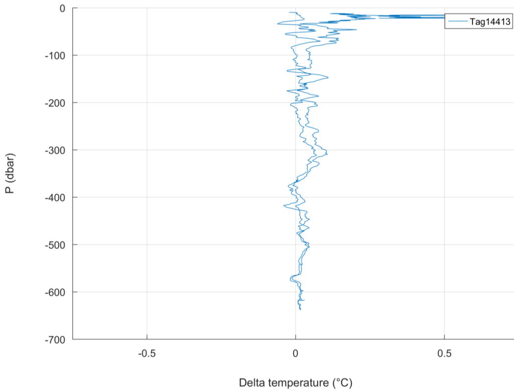
Figure 5.3. 12: Temperature differences between the CTD–SRDL and the ship-based CTD for the third calibration.
