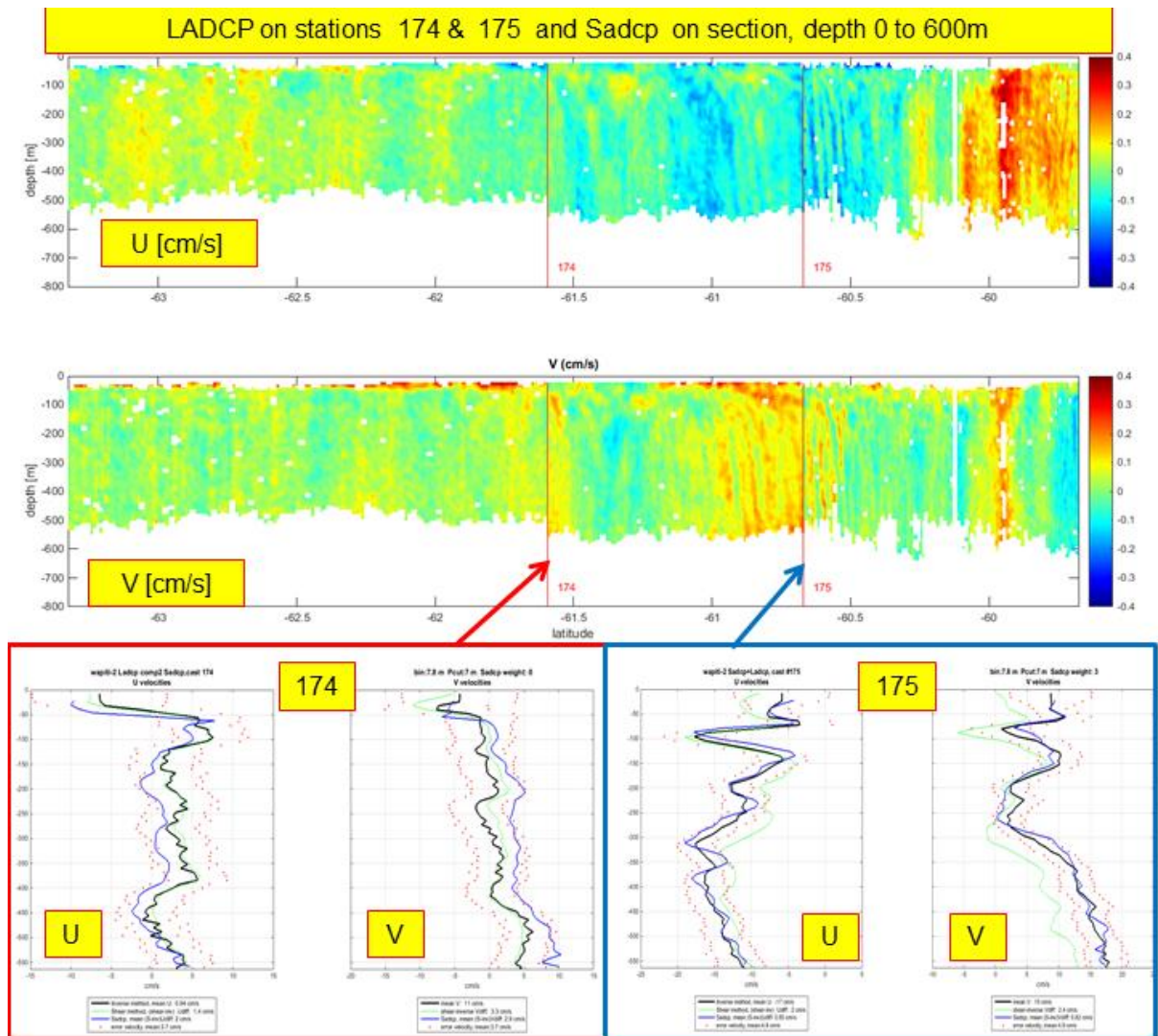
Figure 4.2.13: SADCPUV contours on section and SADCPU/LADCP vertical profiles on stations 174 and 175, for SADCPU max range (600m). Correlation between LADCP and SADCPU profiles is not great on station 174, but good on station 175.
