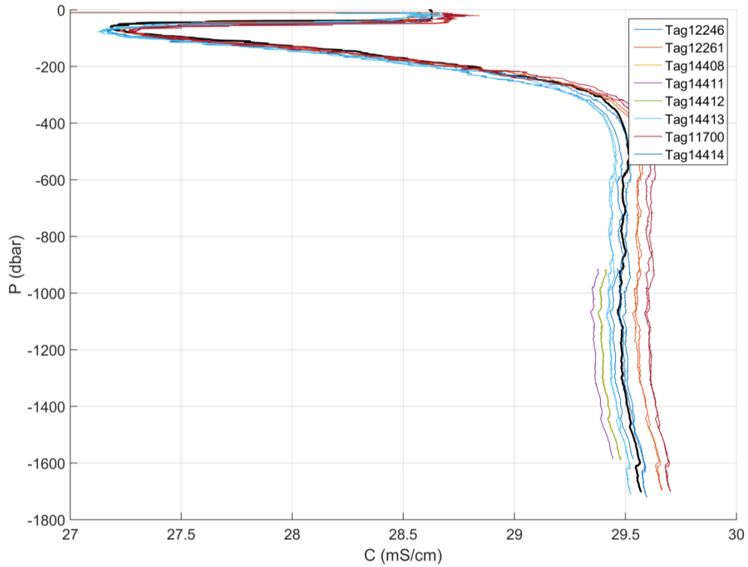
Figure 5.3. 5: Vertical profiles of conductivity, sampled by the 8 CTD-SRDLs (colours) and the ship-based CTD (black) during the same cast for the first calibration.
